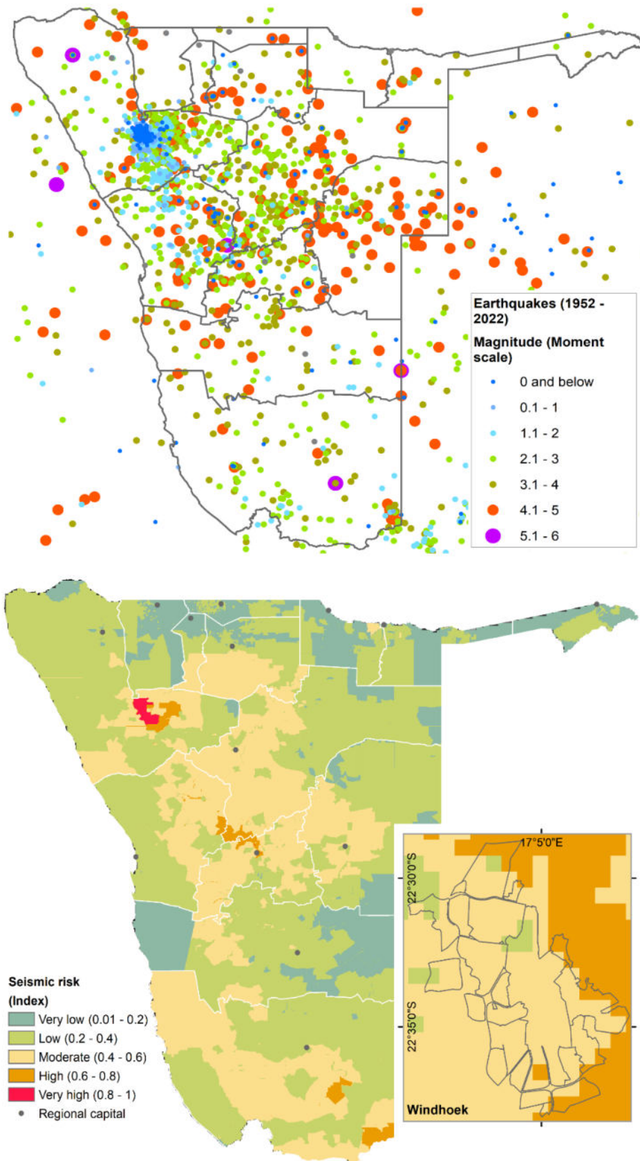
Earthquake occurrence (top) and risk (bottom) in Namibia
