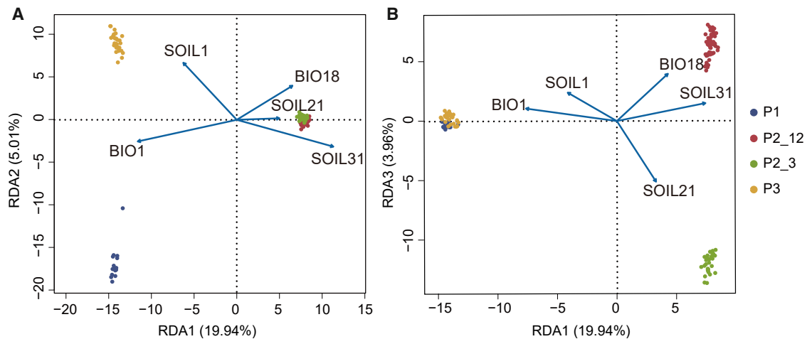
Figure 4. Redundancy analysis showing the relationships between the independent environmental parameters and the population structure of Welwitschia
