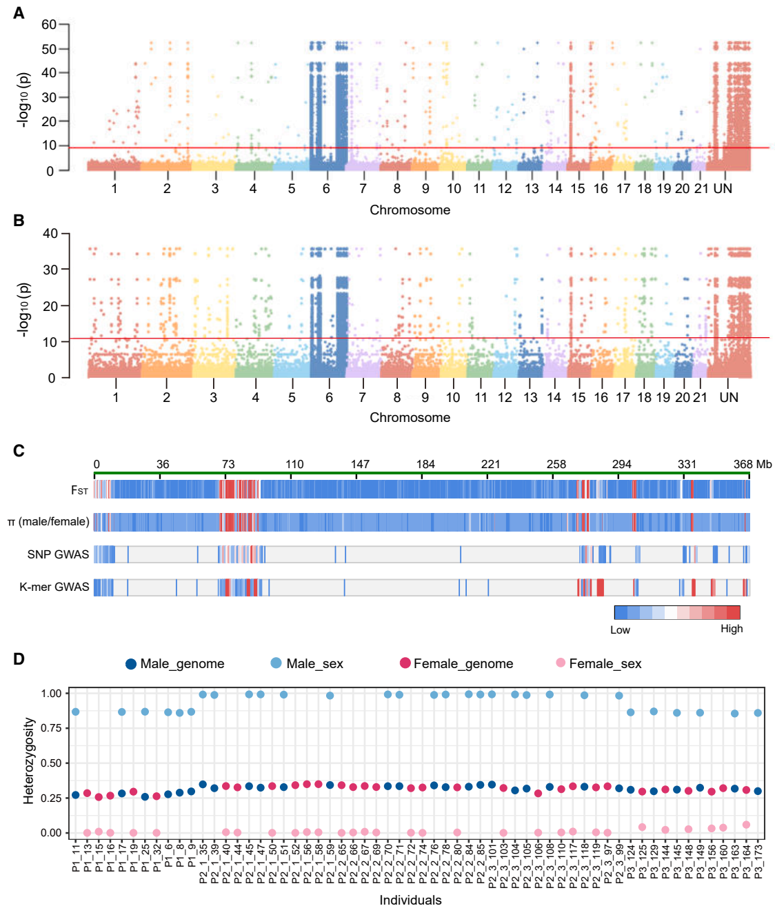
Figure 6. Sex-linked regions and sex-determining system of W. mirabilis
