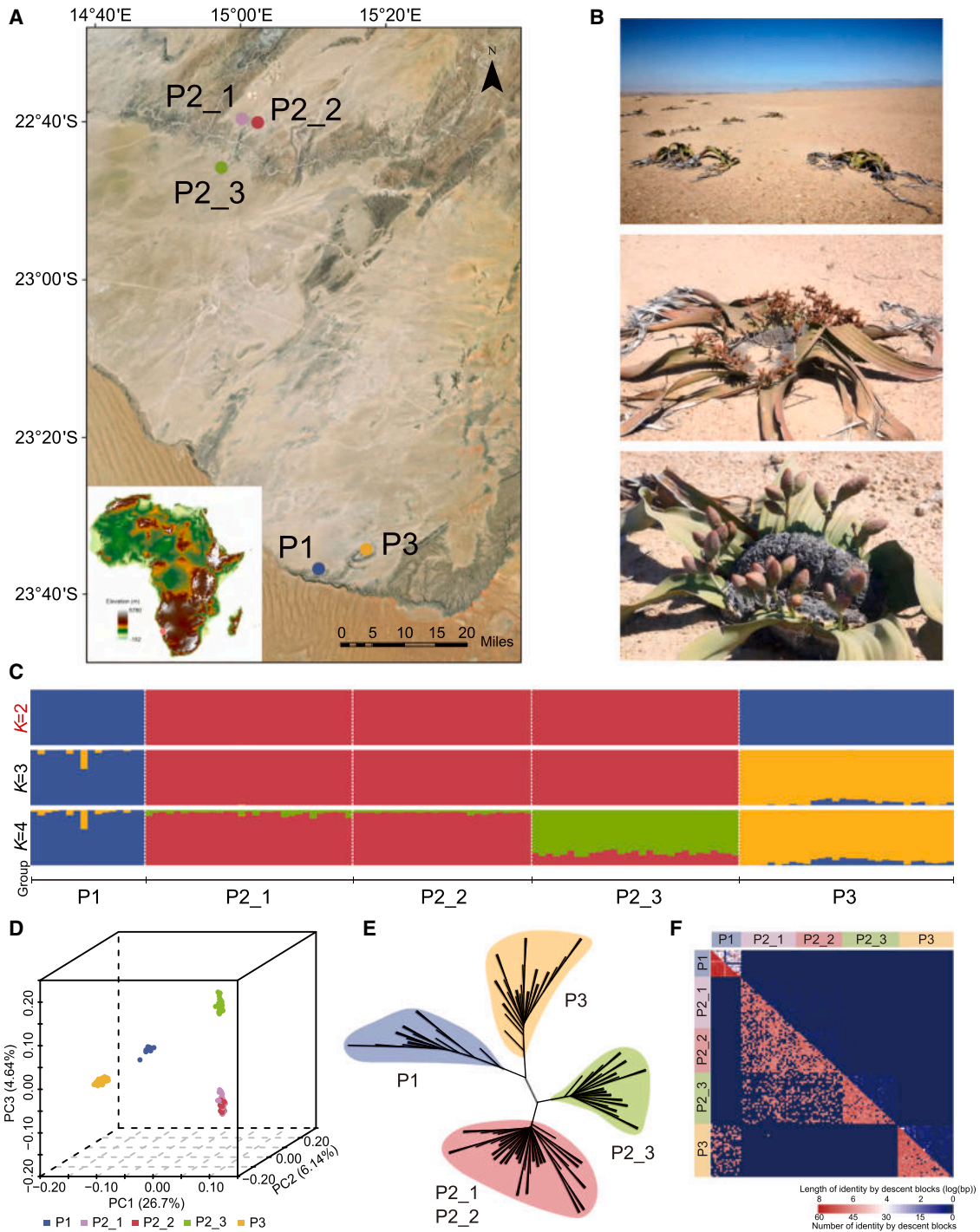
Figure 1. Sampling locations, habitat, morphology, and population genomic analysis of Welwitschia
