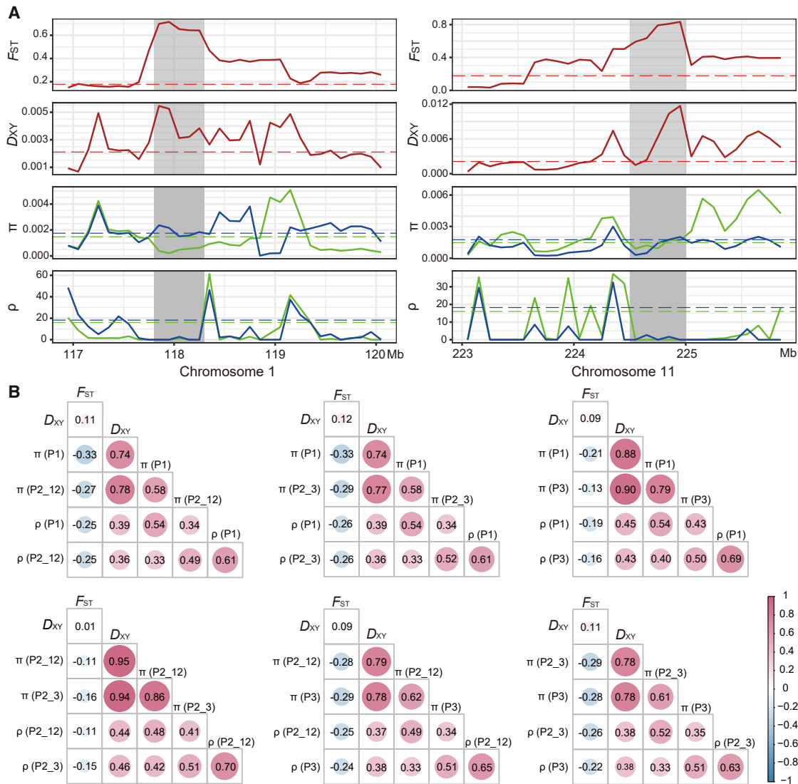
Figure 5. The heterogeneity of genomic divergence in four lineages
