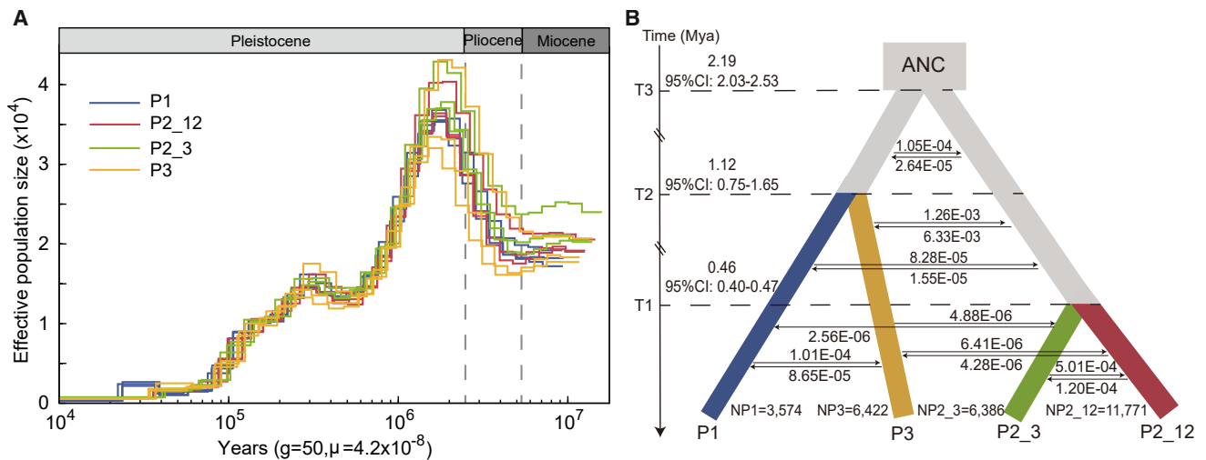
Figure 2. Demographic history of Welwitschia
