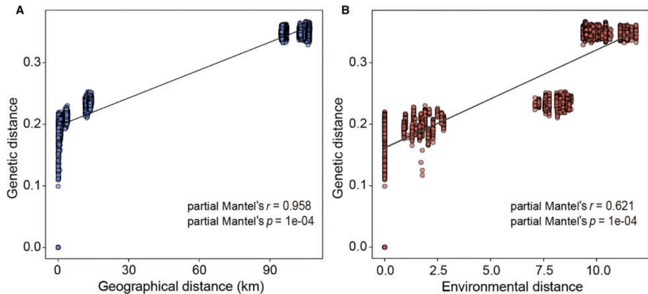
Figure 3. The relationship between genetic and geographical or environmental distances based on partial Mantel tests
