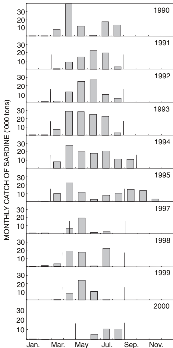
Fig. 6: Monthly sardine catches from 1990 to 2000. Lines indicate the beginning and end of the sardine fishing seasons. Note that the catches in 1996 were insignificant and are not shown. The fishing season was from mid May to end of August in that year
