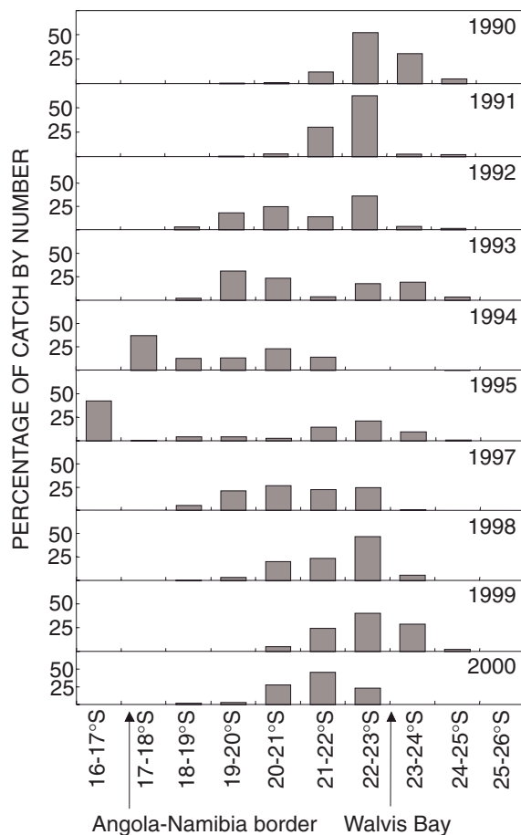
Fig. 8: Distribution of sardine catches by degree latitude during the period 1990–2000. Note that the catches in 1996 were insignificant and are therefore not shown
