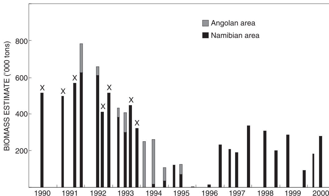
Fig. 4: Biomass estimates of the sardine stock from acoustic surveys from 1990 to 2000. Bars with an X indicate that the Angolan area was not surveyed although sardine was probably present
