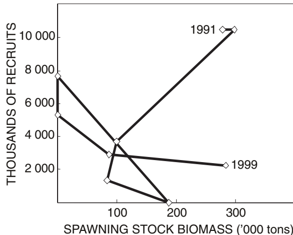
Fig. 9: Number of recruits estimated by the November survey plotted against spawning stock biomass in January of the same year
