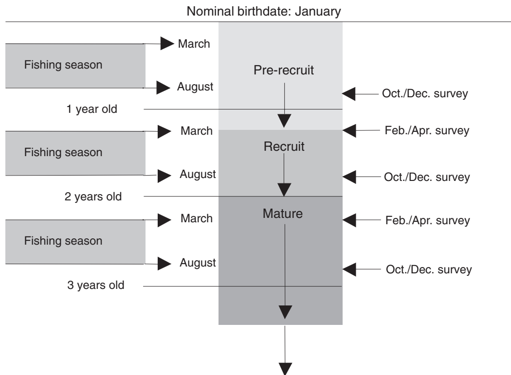
Fig. 3: Major annual events in the fishery and assessment surveys in relation to the life history of northern Benguela sardine
