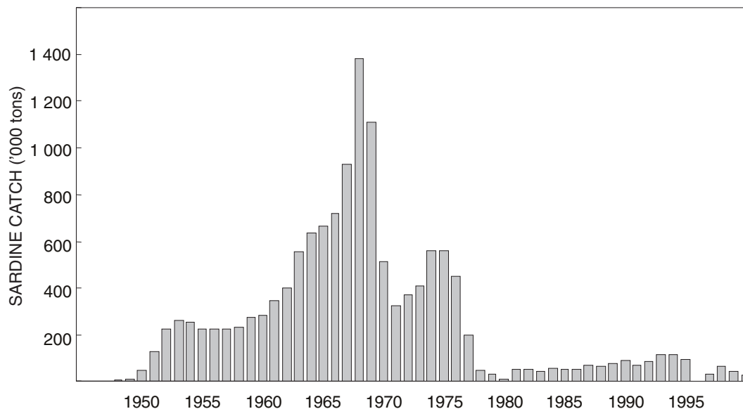
Fig. 2: Catches of sardine from the Namibian part of the northern Benguela since 1947
