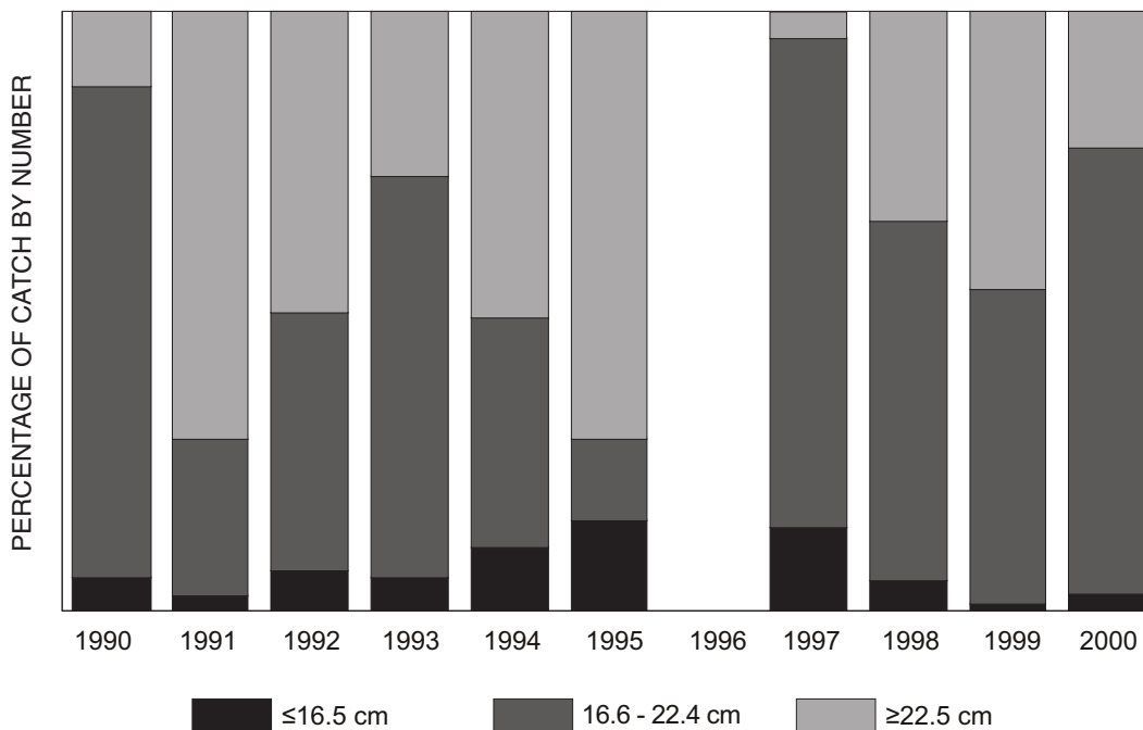
Fig. 7: Proportion of three length-classes (total length) of sardine in commercial catches for the period 1990–2000
