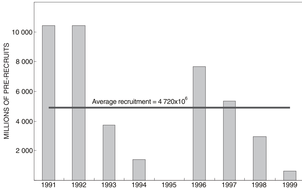
Fig. 5: Estimates of the number of pre-recruits (approx. 9–12 months old) obtained directly from acoustic biomass surveys in the period October–December
