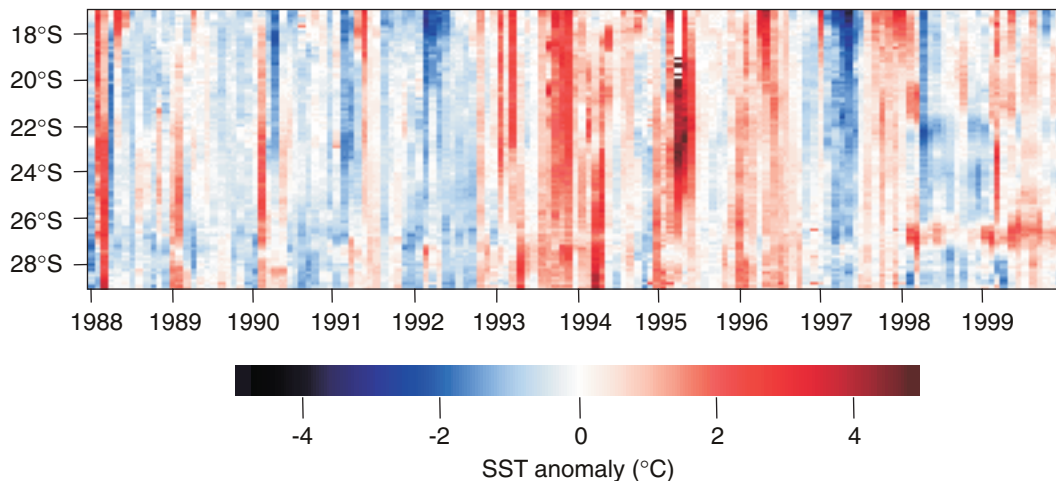
Fig. 10: Sea surface temperature along the Namibian coast (mean from the coast to 50 km offshore). Data supplied by EU project ENVIFISH, contract no. IC18.CT98-329
