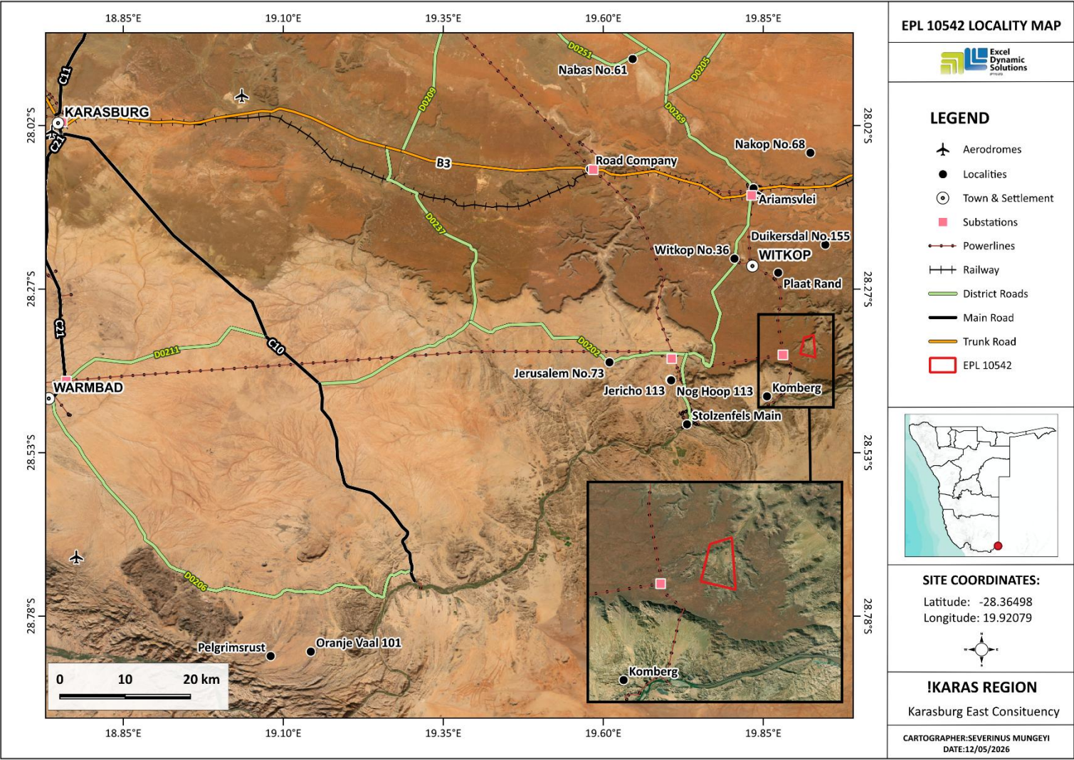
Figure 1: Locality map of EPL No. 10542, Hardap Region, Namibia
