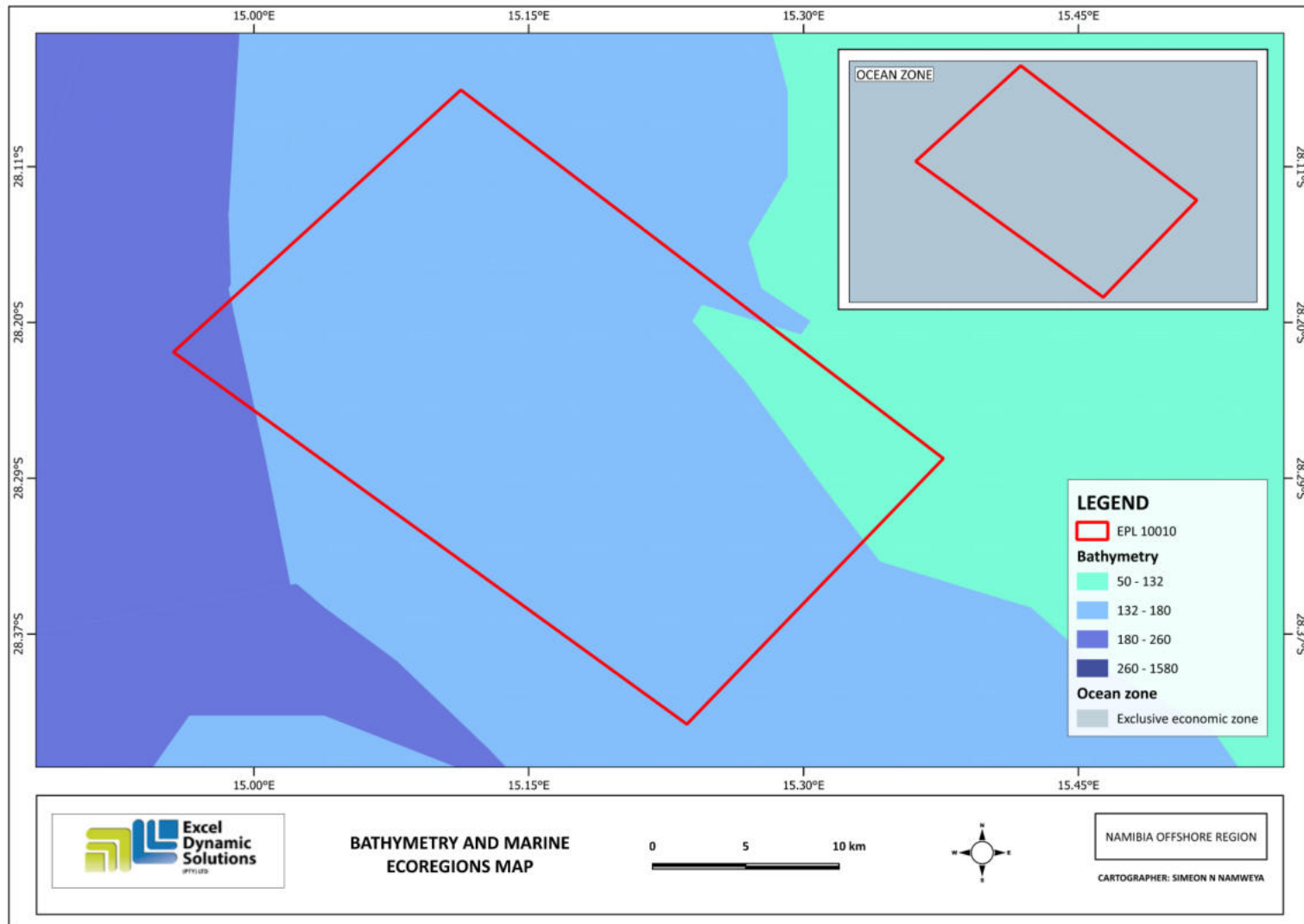
Figure 2: Bathymetry and marine spatial zones of EPL No. 10010 within Namibia's Exclusive Economic Zone (EEZ)
