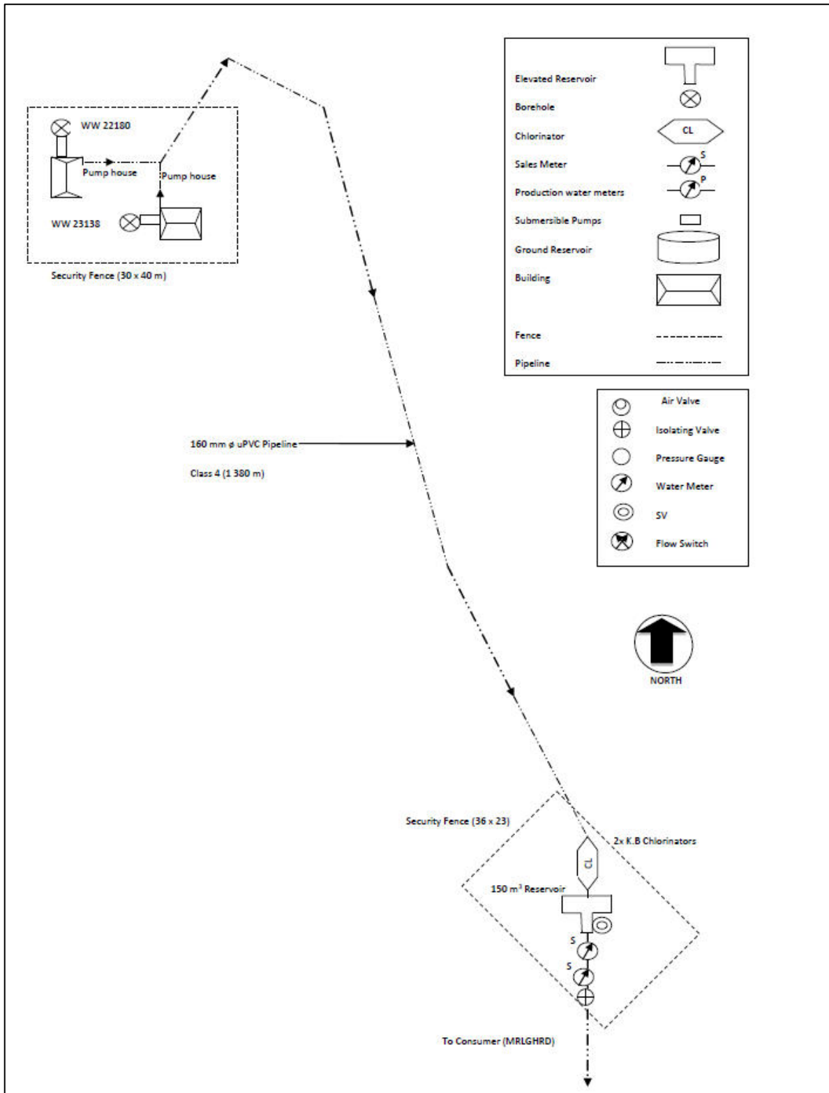
Figure 2: Berseba Scheme Schematic Layout
