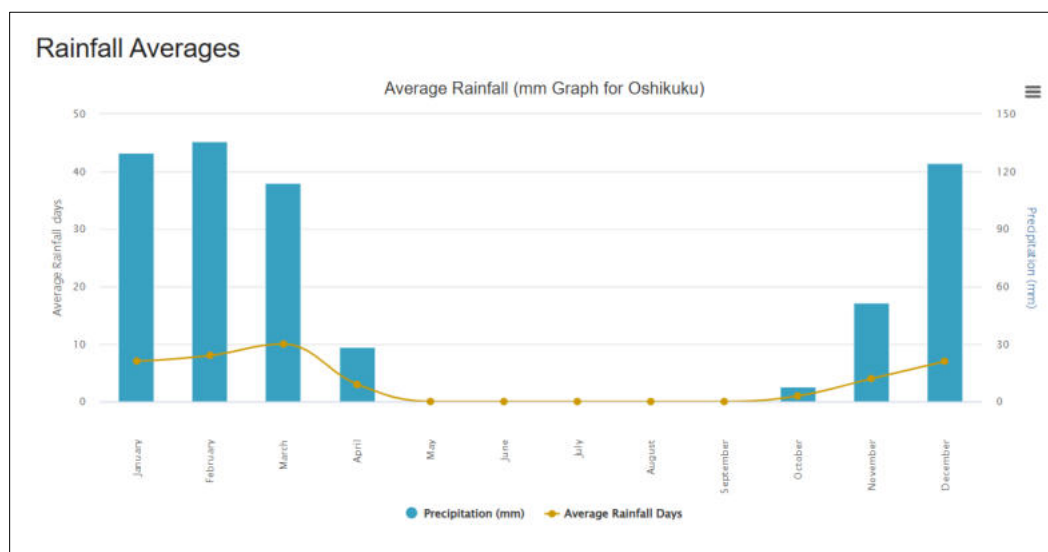
Figure 5-5: Average rainfall chart for the area (source: World Weather Online, 2026)
