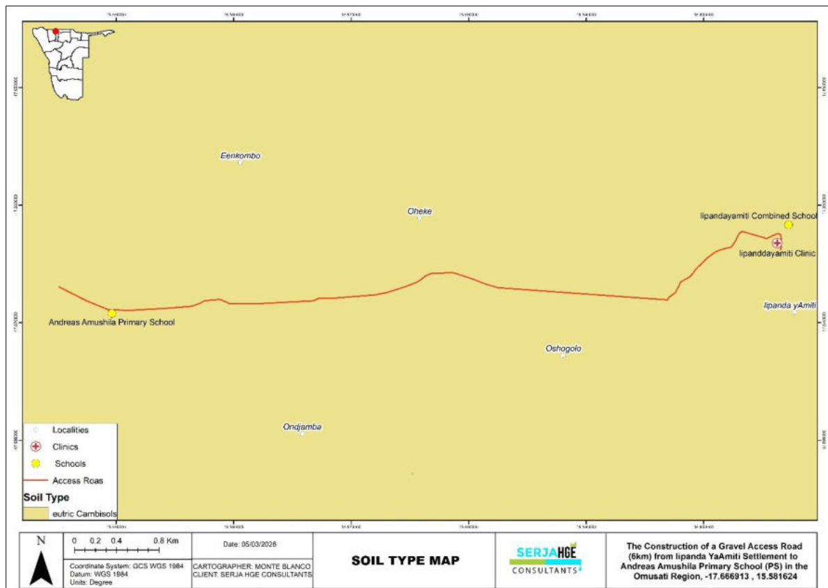
Figure 5-8: The dominant soil types along the access road
