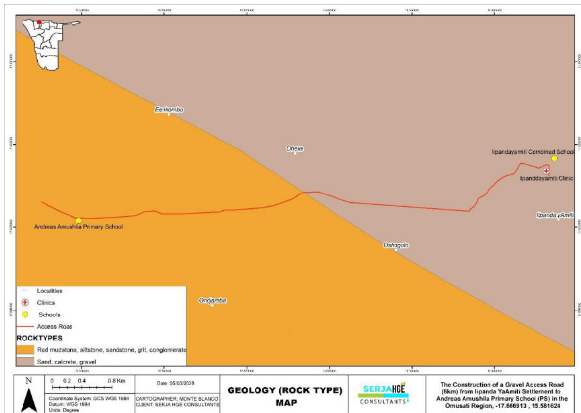
Figure 5-7: The geology of the project route area and surroundings
