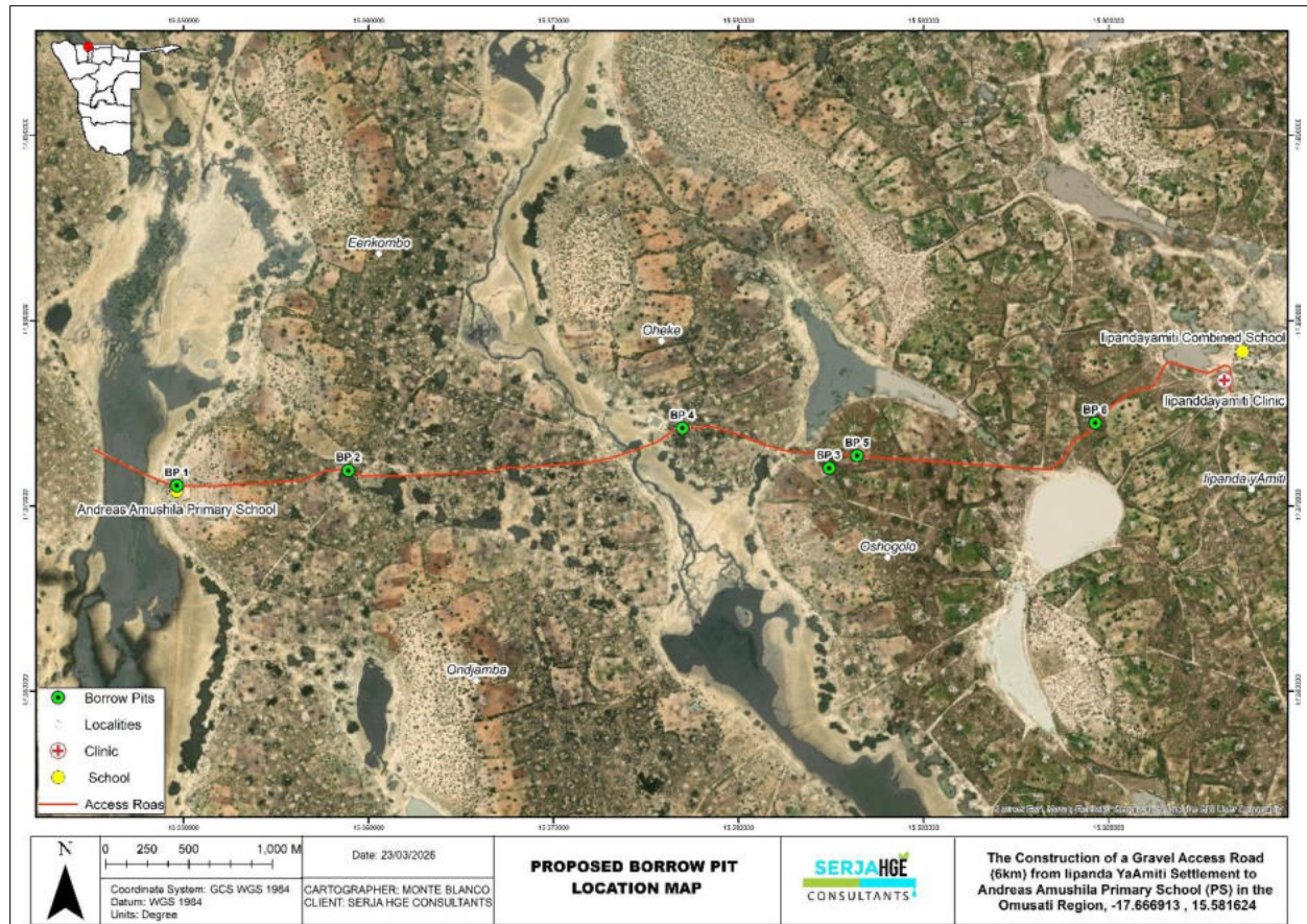
Figure 2-3: The locality map of proposed borrow pits between lipanda YaAmiti Settlement and Andreas Amushila Primary School
