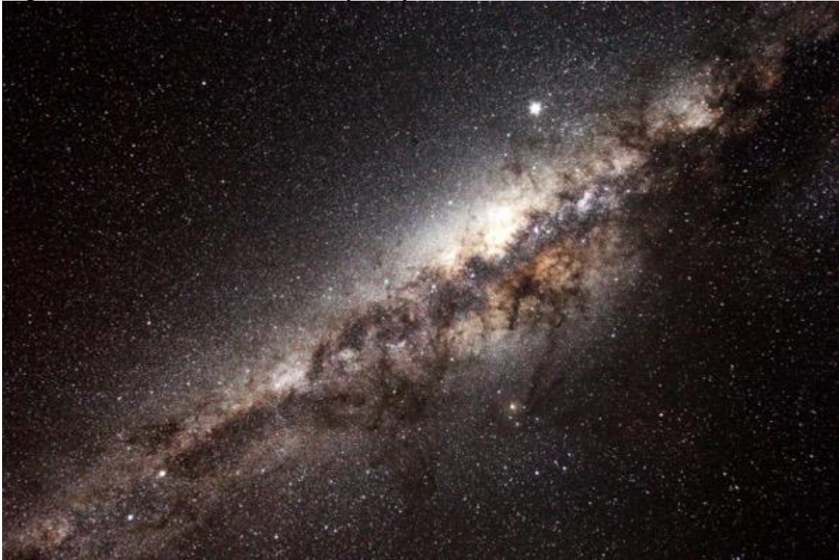
Figure 8: The Centre of the Milky Way
