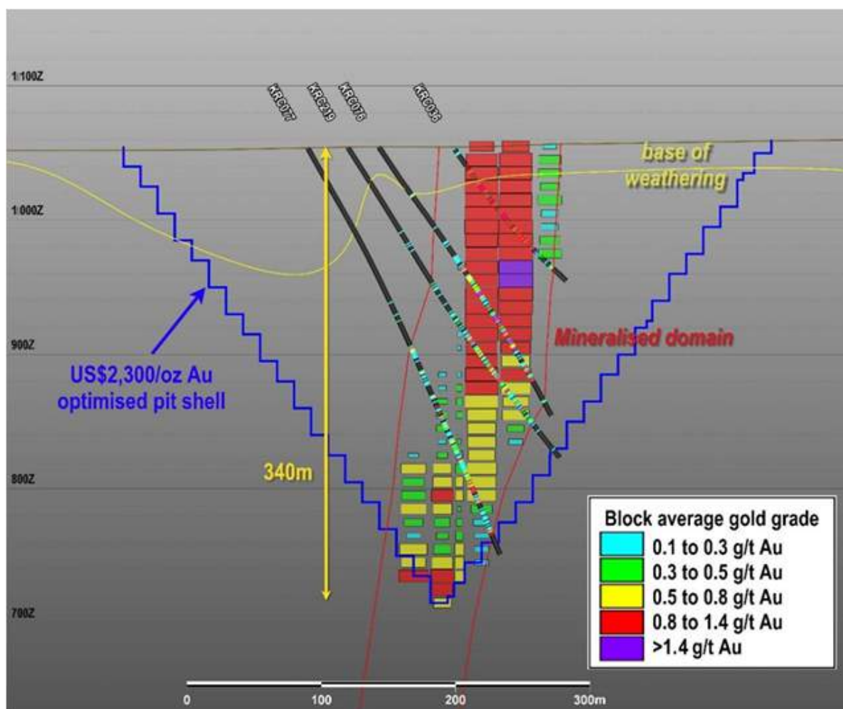
Figure 12 - Cross section of the southern zone, showing US$2,300/oz pit shell, weathering base, mineralised domains and block model scaled by proportion at 0.50 g/t cut-off over drilling results (Source: WiaGold, 2025)
