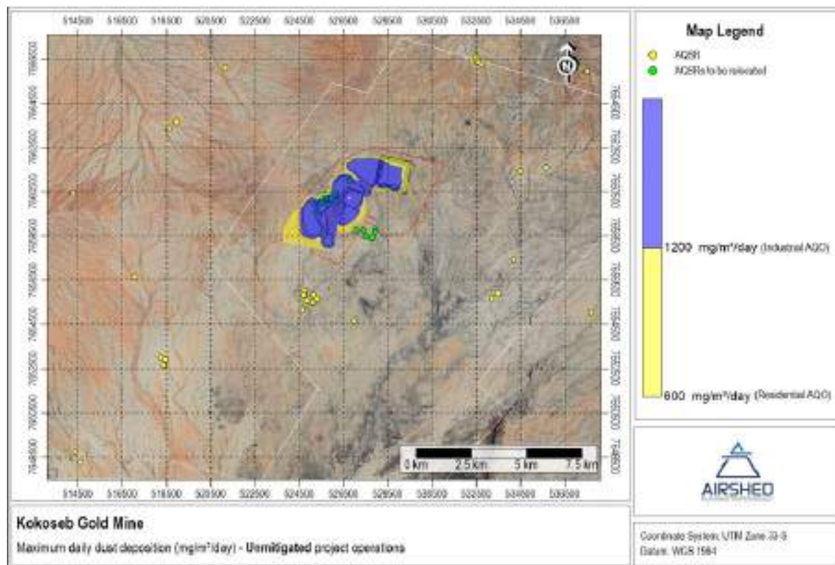
Figure 104 - Dust fallout dispersion concentrations (before mitigation) during year three (3) of operations (Source: Airshed, 2025)
