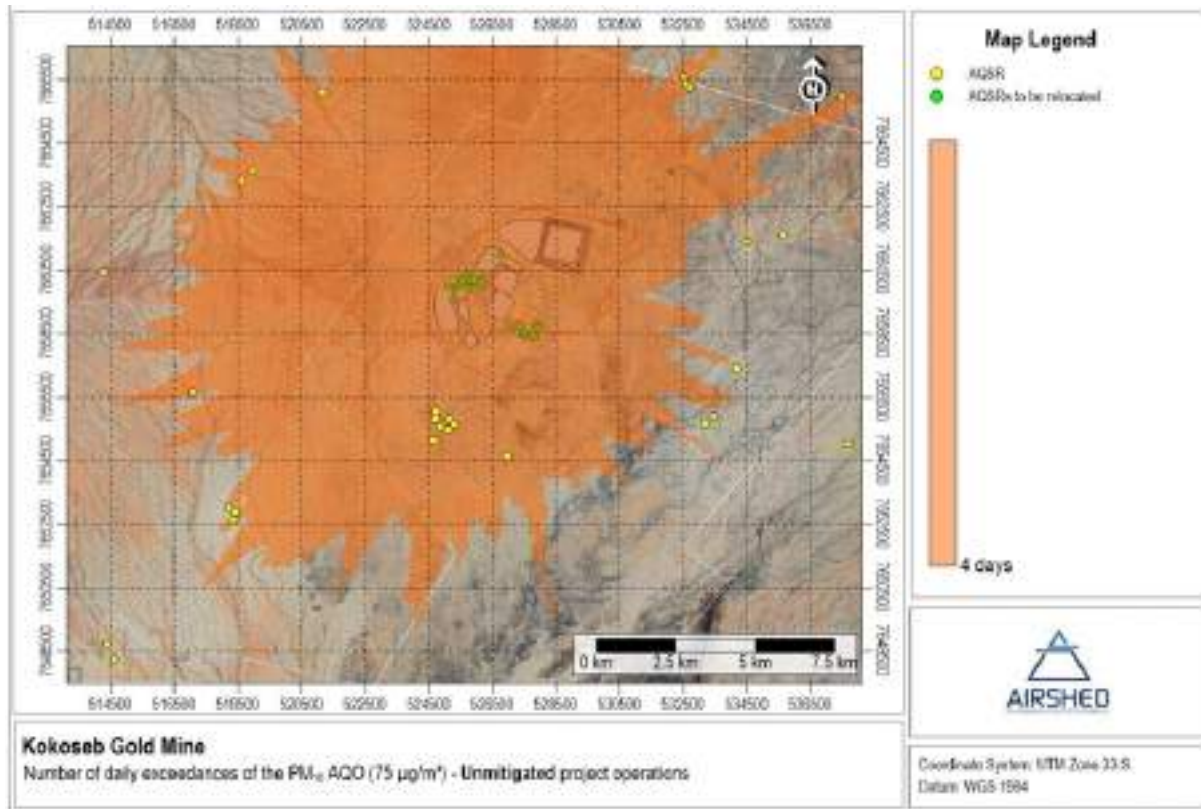
Figure 106 - Simulated daily PM 10 dispersion concentrations (before mitigation) during year three (3) of operations (Source: Airshed, 2025)
