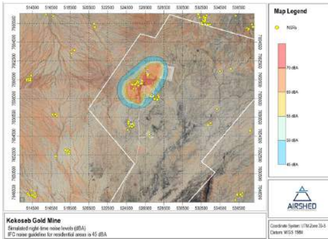
Figure 87 - Simulated nighttime noise levels during normal Project operations in relation to NSRs (Airshed, 2025)
