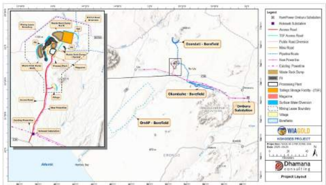
Figure 19 - Location of the bore fields and pipeline routes (Source: WiaGold, 2025)
