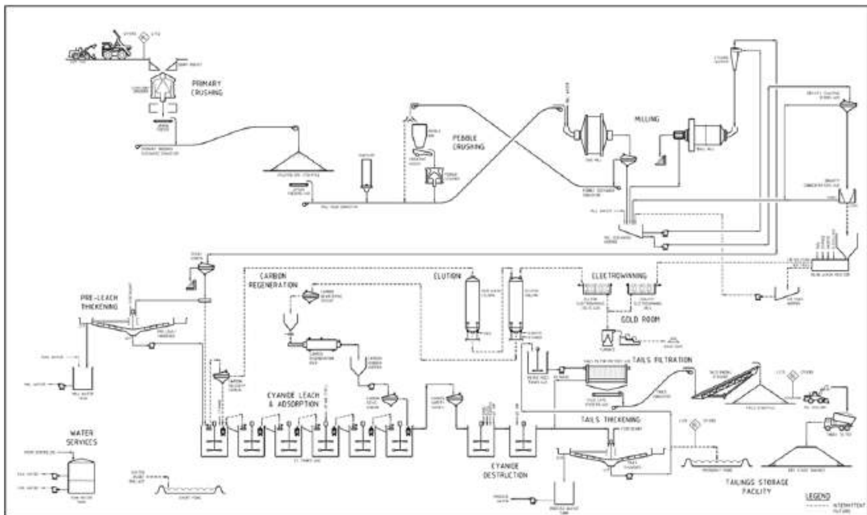
Figure 16 - Metallurgical process flow (Source: WiaGold, 2025)
