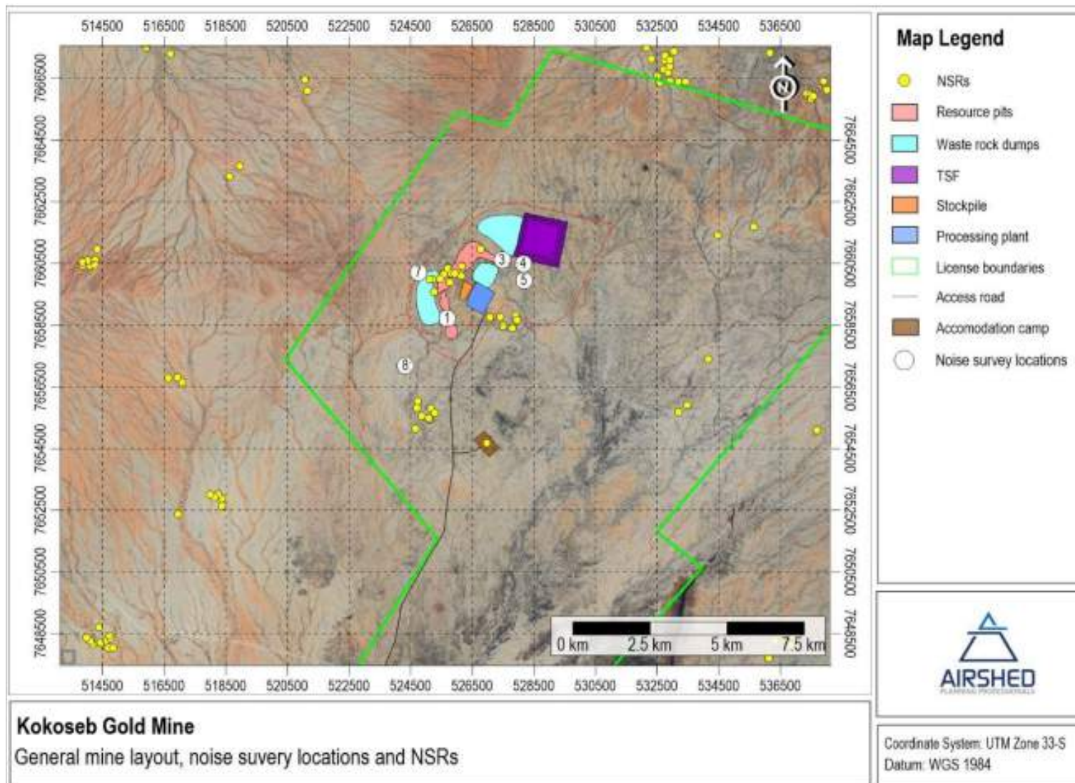
Figure 36 - Baseline noise survey locations and NSRs (Source: Airshed, 2025)
