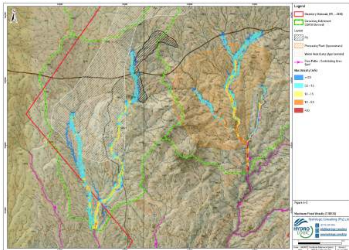
Figure 120 - Maximum flood velocity (Hydrologic, 2025)
