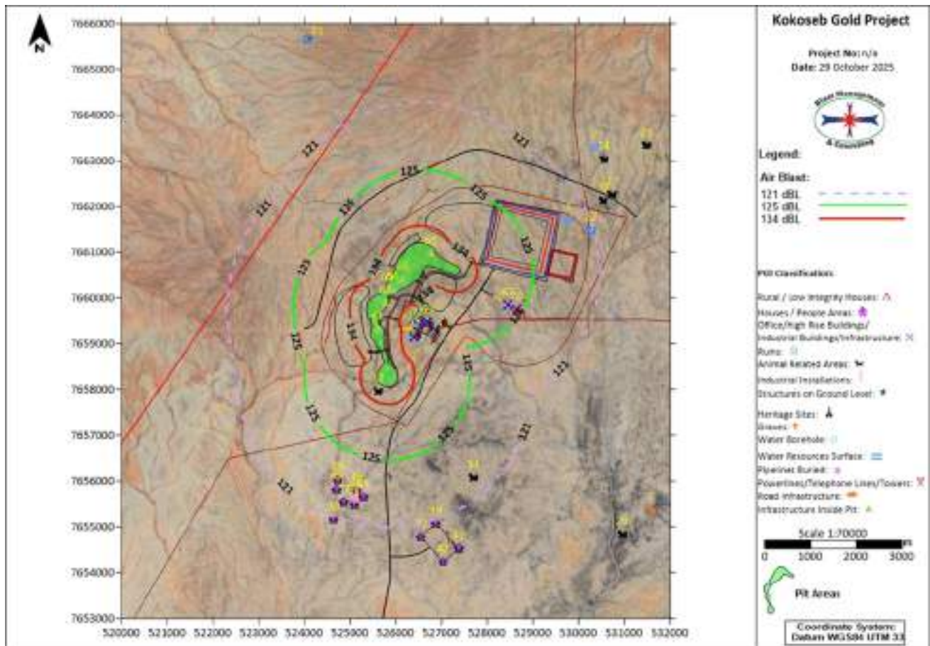
Figure 92 - Air blast influence from the maximum charge per delay (689 kg) (Source: BMC, 2025)
