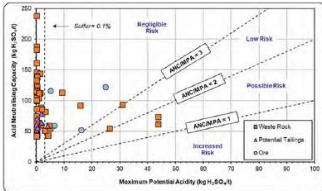
Figure 60 - ANC vs MPA for the tested mine material samples (Source: RGS, 2025)
