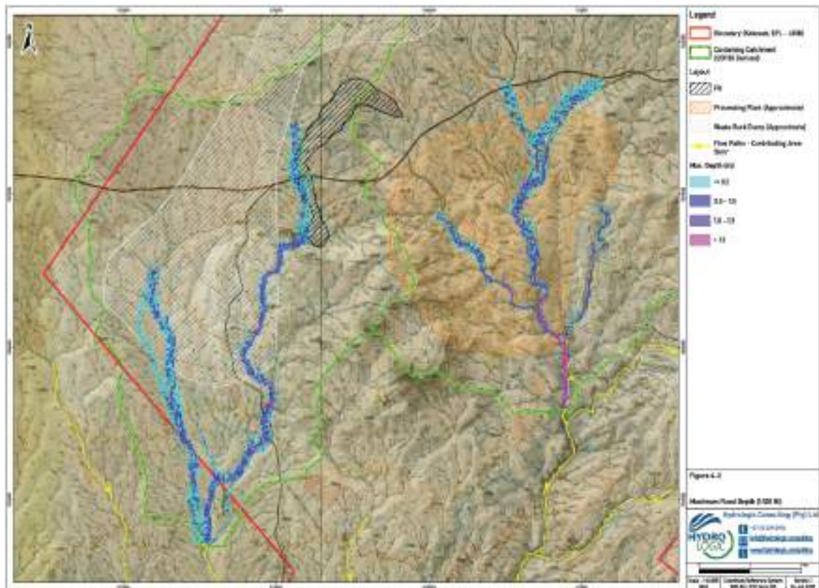
Figure 119 - Maximum depth of flooding for the 1:100 RI event (Hydrologic, 2025)
