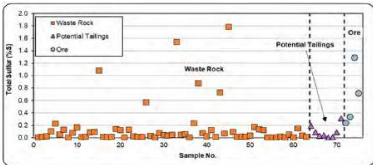
Figure 58 - Total sulphur concentrations of the tested mine materials (Source: RGS, 2025)
