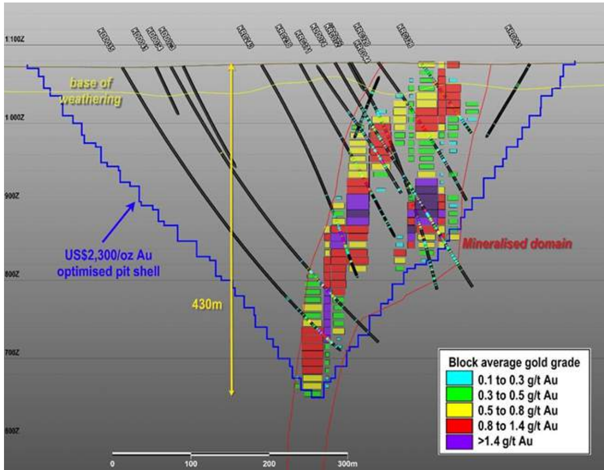
Figure 11 - Cross section of the central zone, showing US$2,300/oz pit shell, weathering base, mineralised domains and block model scaled by proportion at 0.50 g/t cut-off over drilling results (Source: WiaGold, 2025)
