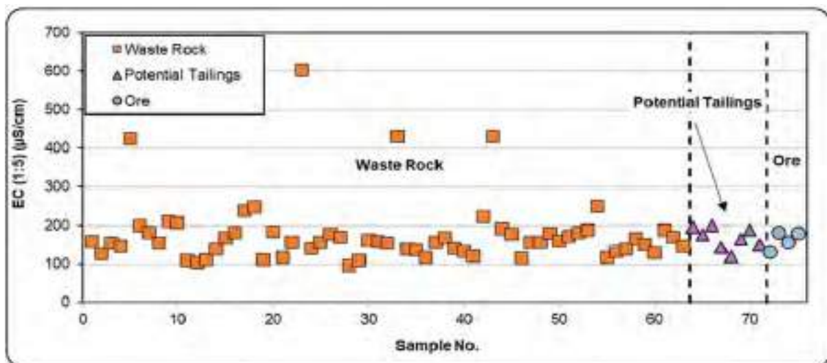
Figure 57 - EC values for the tested mine materials (Source: RGS, 2025)
