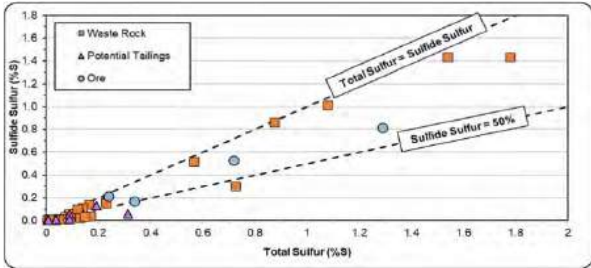
Figure 59 - Total sulphur vs sulphide sulphur for mine material samples (Source: RGS, 2025)
