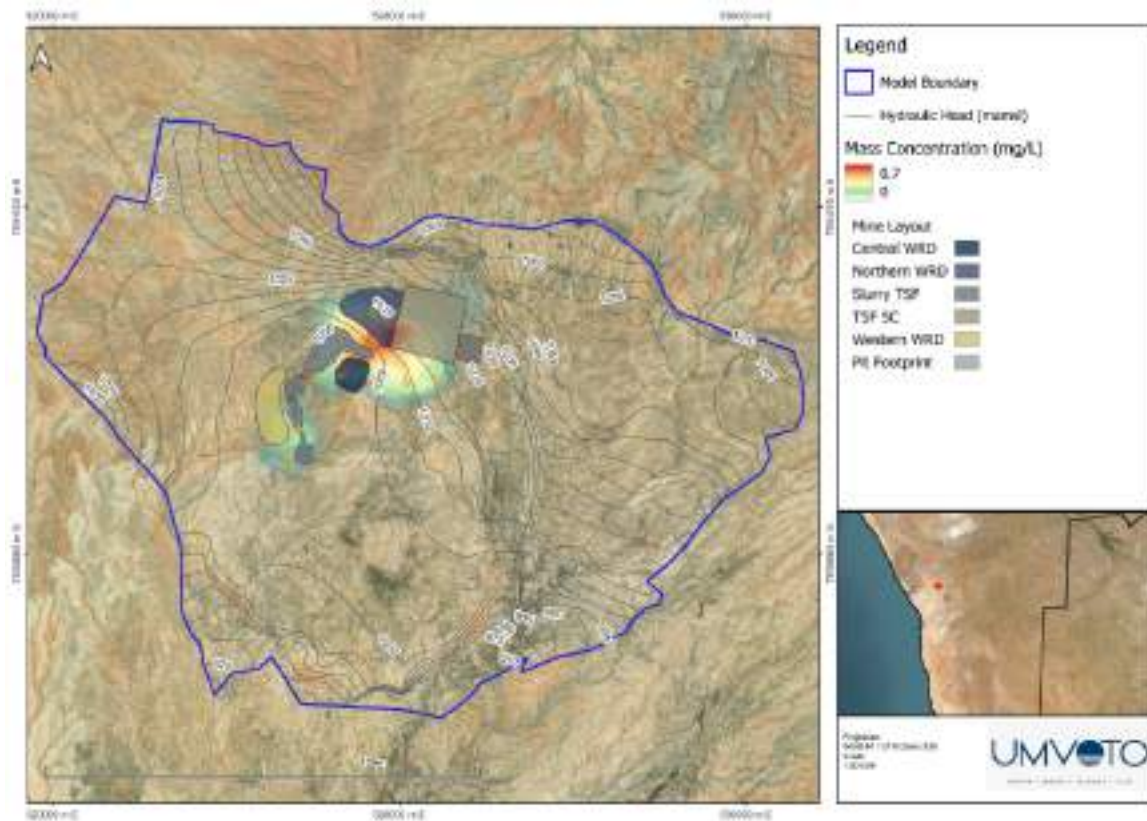
Figure 124 - Extent of potential contaminant plume prior to migrating toward the pit (Umvoto, 2024; Umvoto, 2025)
