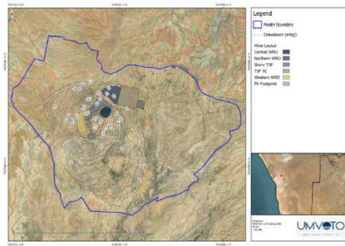
Figure 123 - Drawdown cone due to pit dewatering (Umvoto, 2024; Umvoto, 2025)
