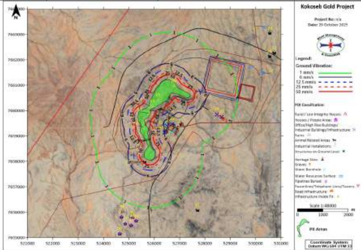
Figure 90 - Ground vibration influence from the maximum charge per delay (Source: BMC, 2025)
