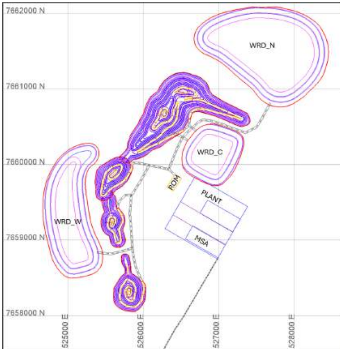
Figure 21 - Location of the WRDs (Source: WiaGold, 2025)
