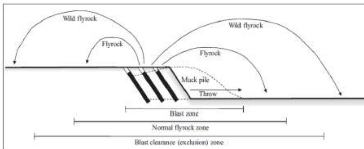
Figure 94 - Schematic of fly rock terminology (Source; BMC, 2025)
