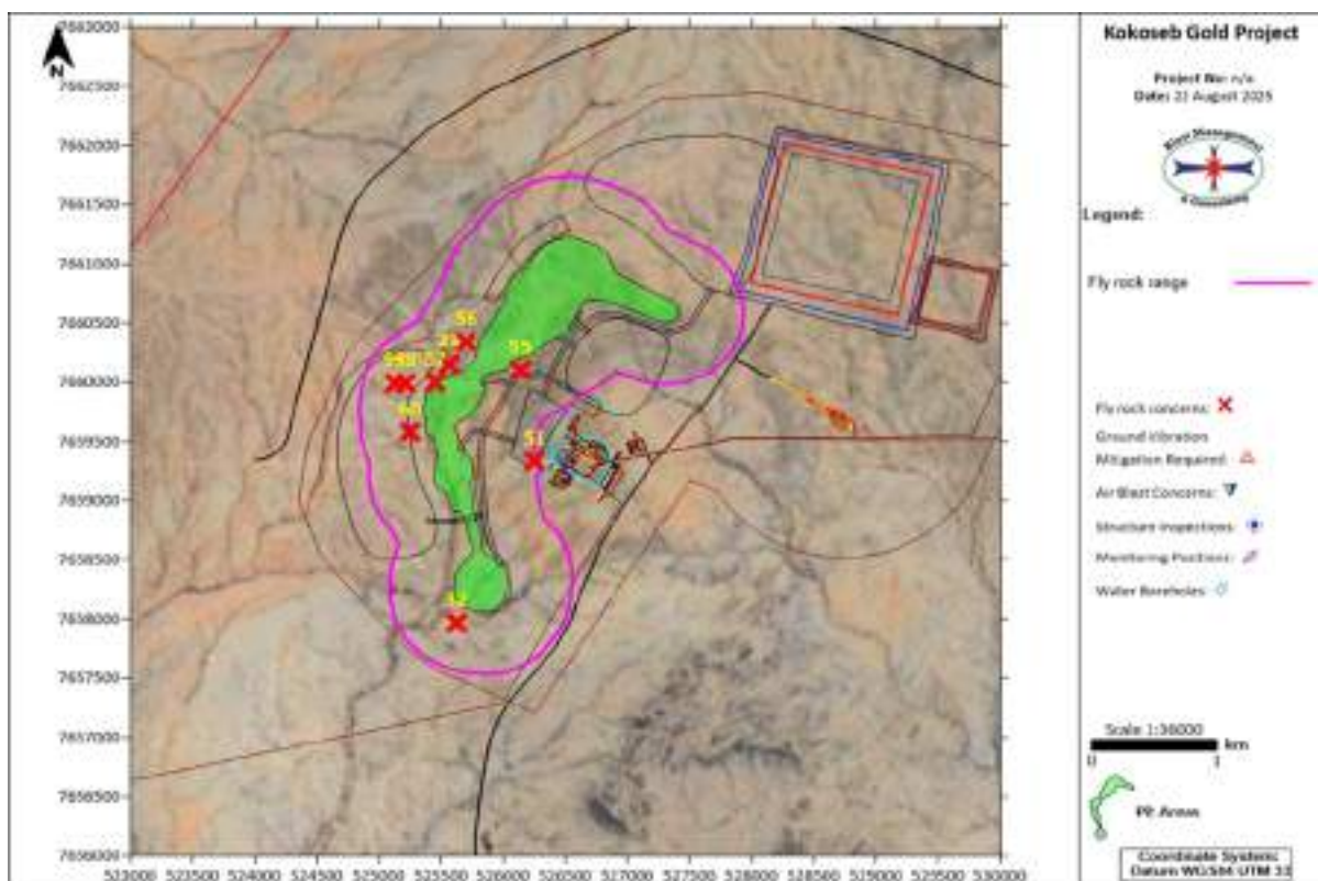
Figure 96 - Predicted fly rock exclusion zone for the Kokoseb Gold Project open pit operations (Source; BMC, 2025)
