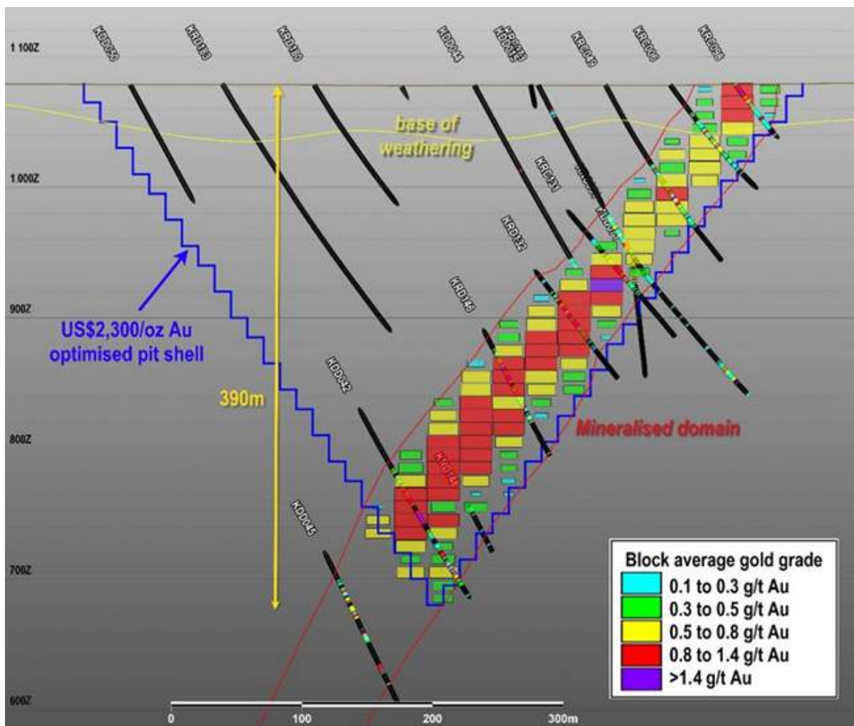
Figure 10 - Cross section of the northern zone, showing US$2,300/oz pit shell, weathering base, mineralised domains and block model scaled by proportion at 0.5 g/t cut-off over drilling results (Source: WiaGold, 2025)
