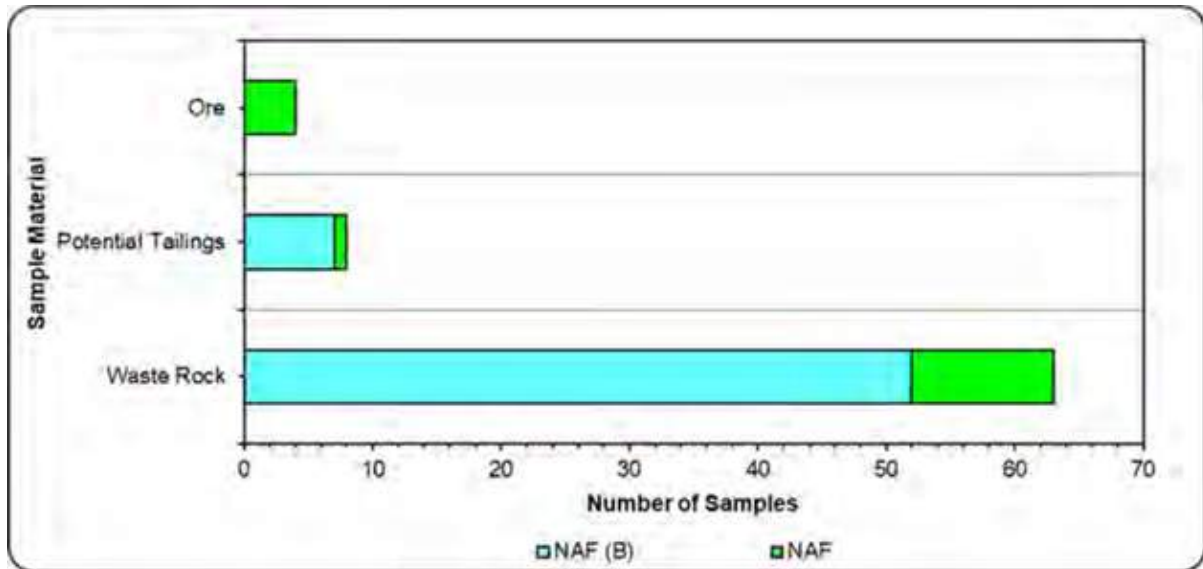
Figure 62 - Geochemical classification by material type (Source: RGS, 2025)
