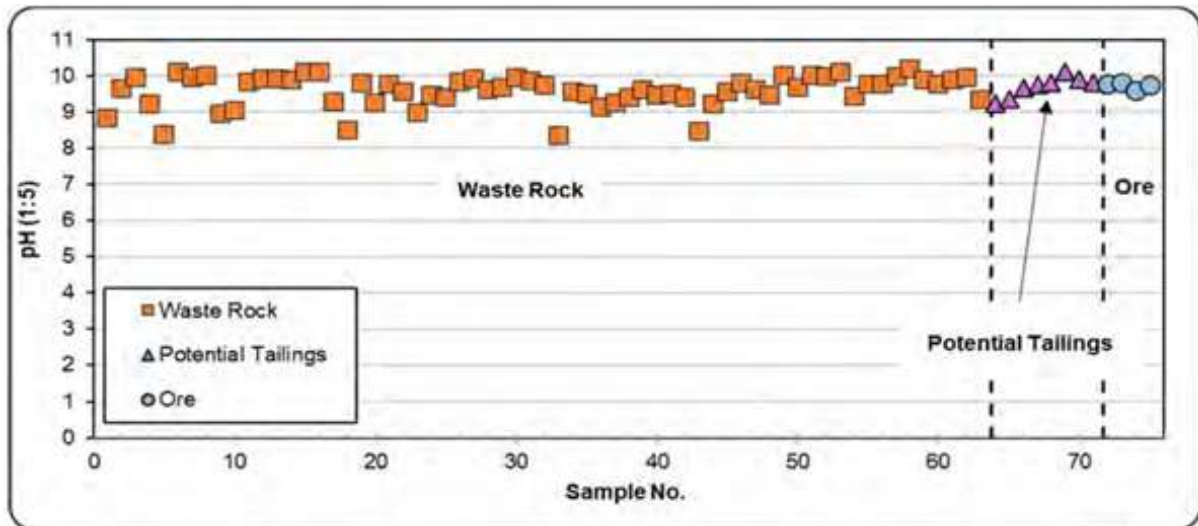
Figure 56 - pH values of tested mine materials (Source: RGS, 2025)
