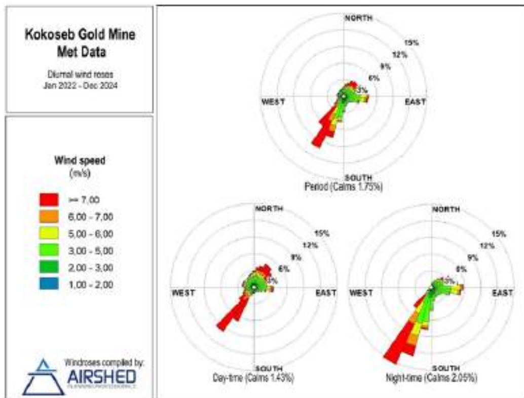
Figure 48 - Daytime and nighttime wind roses for the broader region, derived from WRF modelled data (01 January 2022 to 31 December 2024) (Source: Airshed, 2025)
