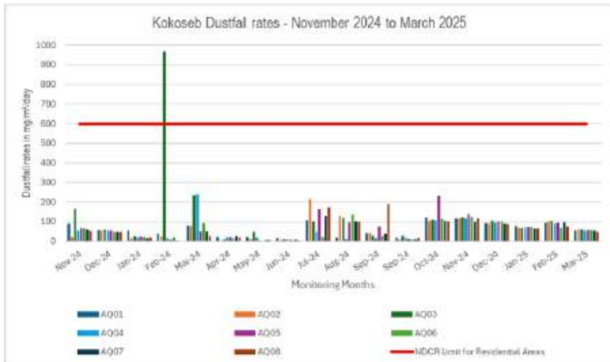
Figure 44 - Dust fallout results from November 2024 to March 2025 (Source: Airshed, 2025)
