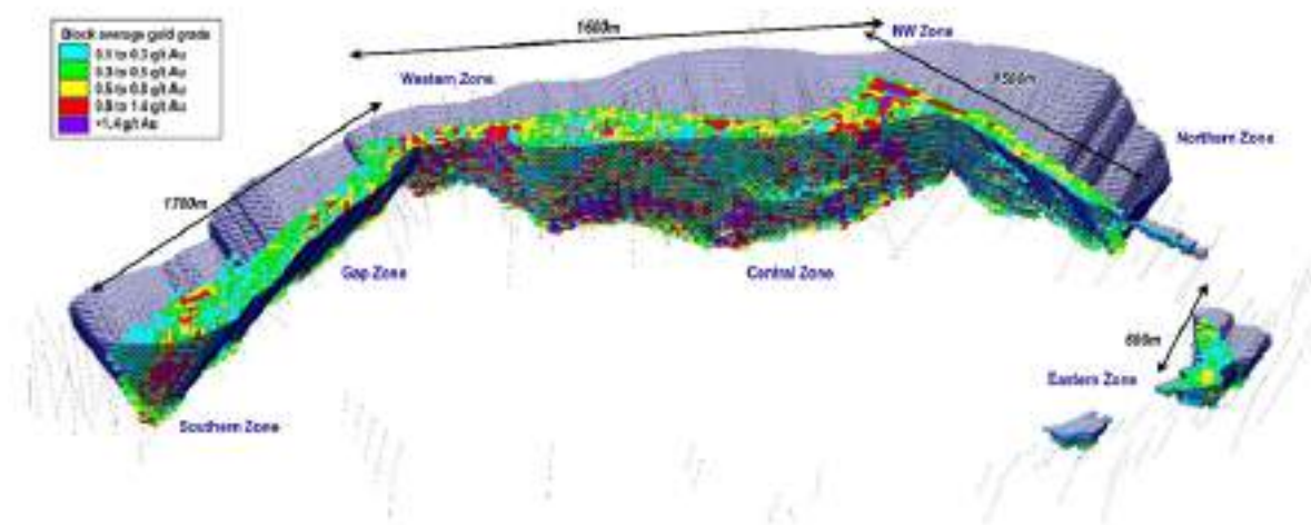
Figure 9 - Block model of the Kokoseb deposit (Source: WiaGold, 2025)
