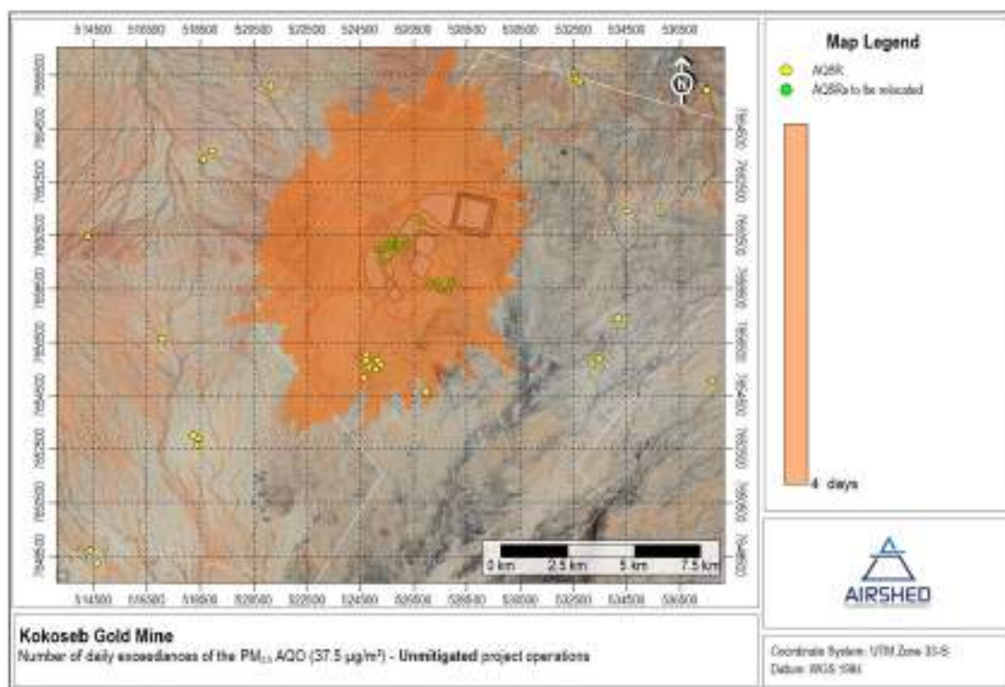
Figure 108 - Simulated daily PM 2.5 dispersion concentrations (before mitigation) during year three (3) of operations (Source: Airshed, 2025)
