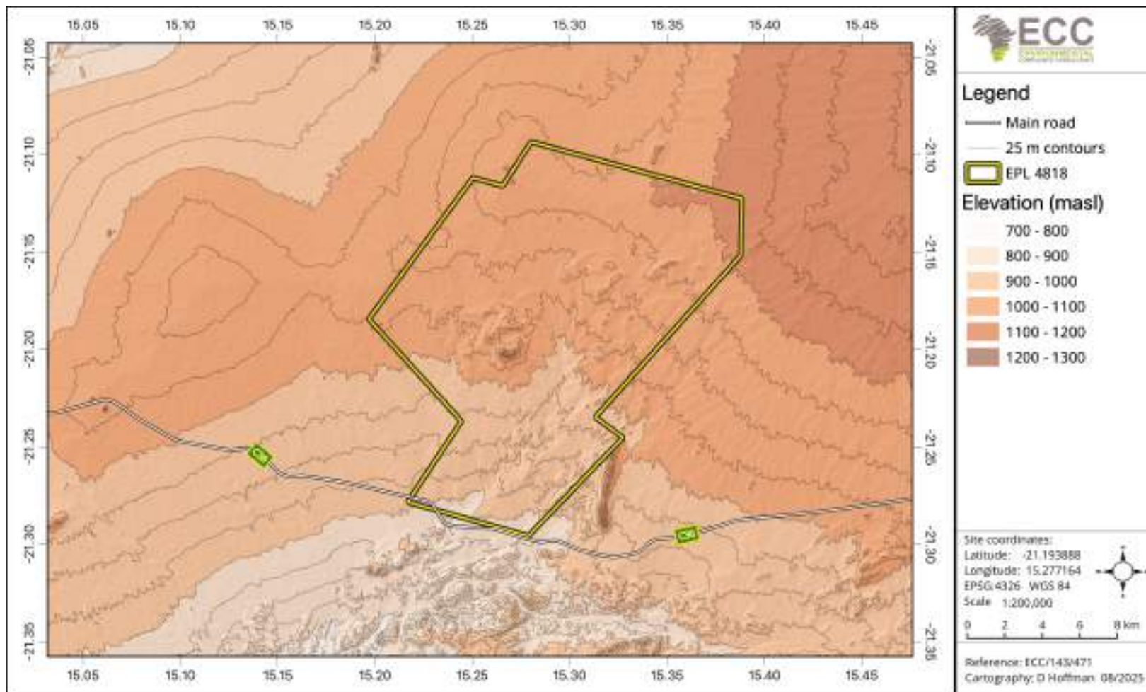
Figure 47 - Topography map for the Project area
