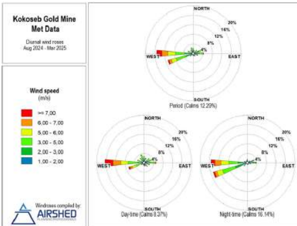
Figure 50 - Daytime and nighttime wind roses for the Project site, derived from on-site meteorological data (30 August 2024 to 06 March 2025) (Source: Airshed, 2025)
