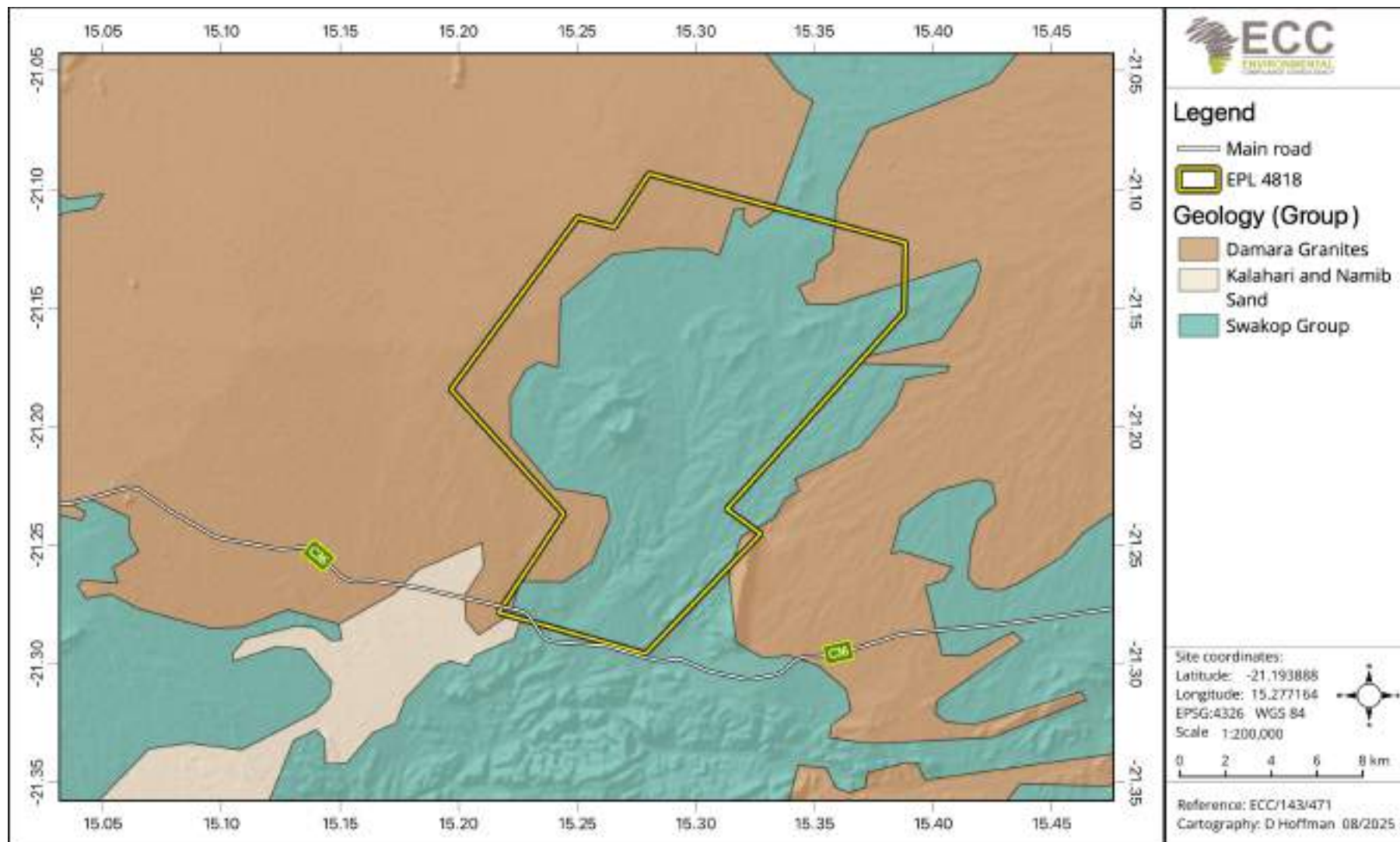
Figure 46 - Regional geological setting of the Project site
