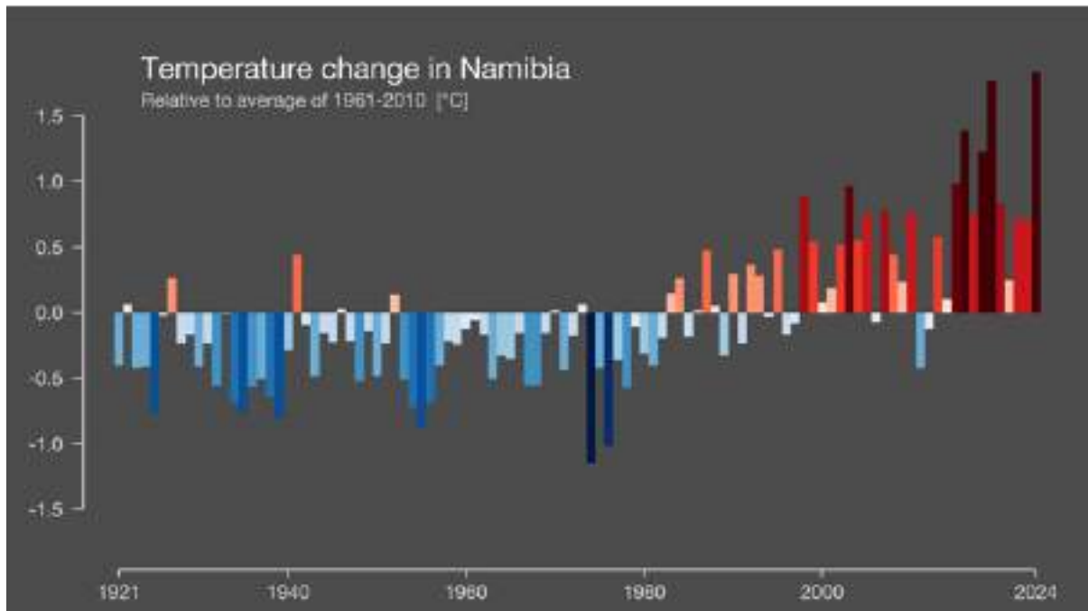
Figure 52 - Changes in Namibia's average mean temperature (°C) from 1921 to 2024 (Source: RDJ Consulting, 2025)
