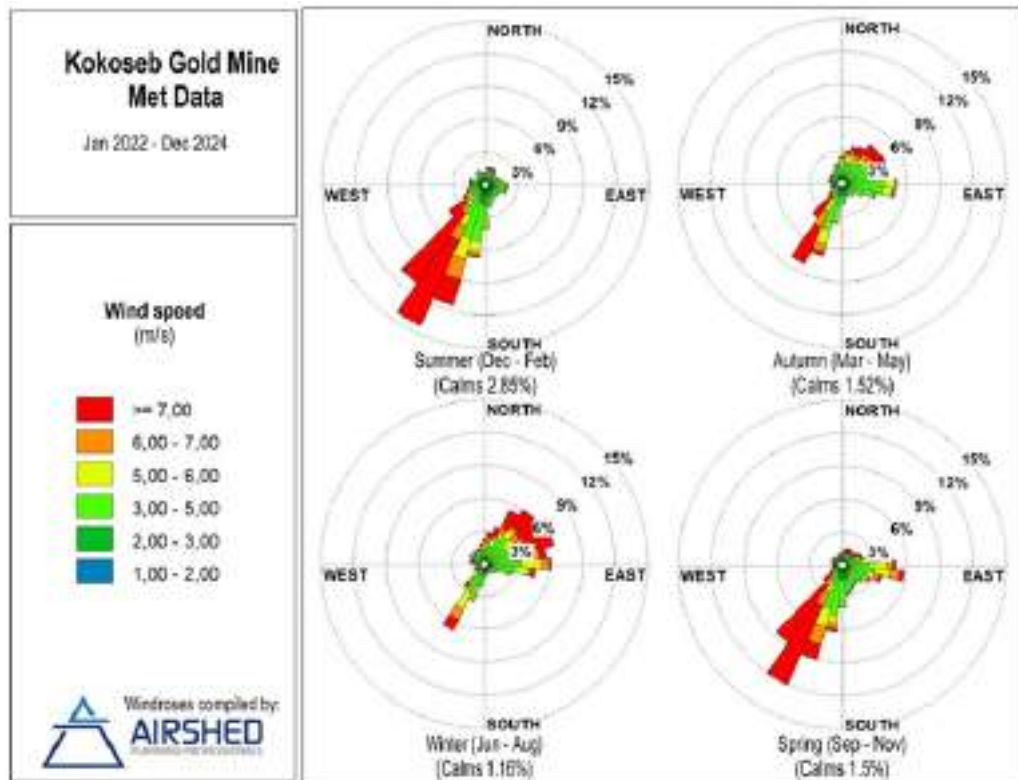
Figure 49 - Seasonal wind roses for the broader region, derived from WRF modelled data (01 January 2022 to 31 December 2024) (Source: Airshed, 2025)
