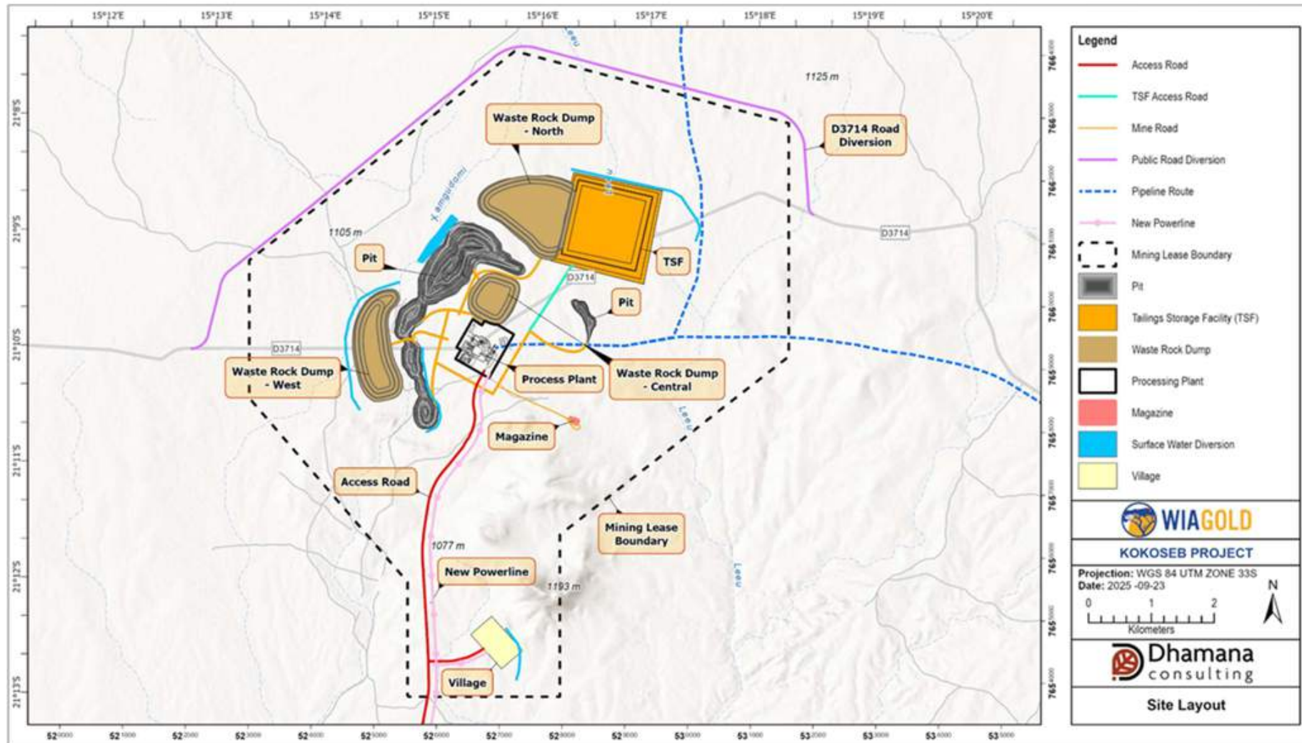
Figure 13 - Kokoseb Gold Mine site layout (Source: WiaGold, 2025)
