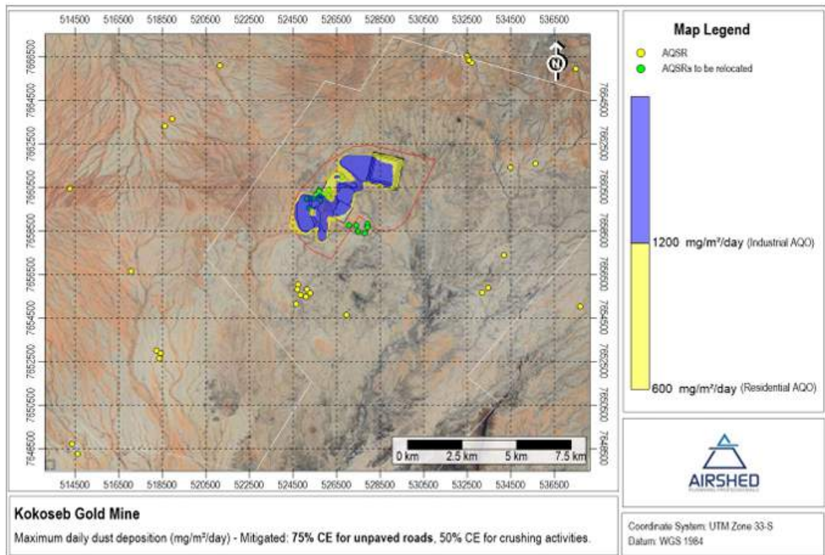
Figure 105 - Dust fallout concentration (post mitigation) during year three (3) of operations (Source: Airshed, 2025)
