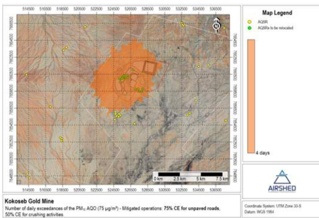
Figure 107 - Simulated daily PM10 dispersion concentrations (post mitigation) during year three (3) of operations (Source: Airshed, 2025)
