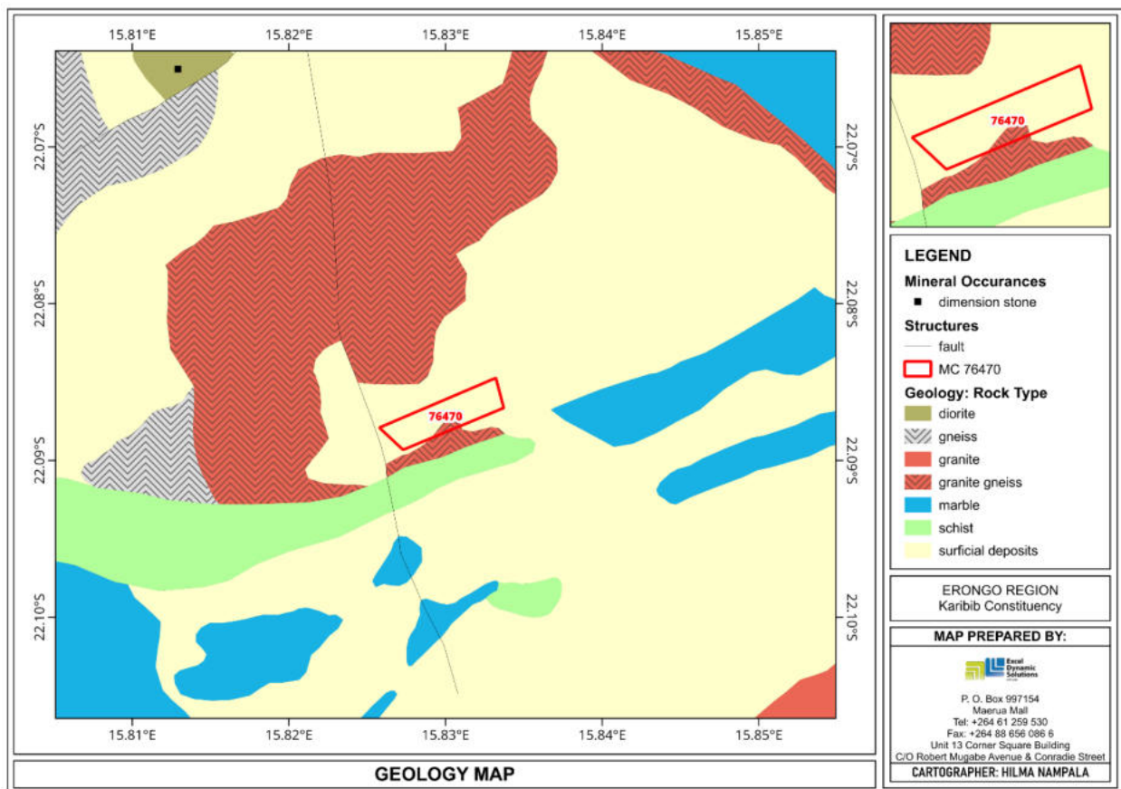
Figure 5: General geology and lithology map of the MC.
