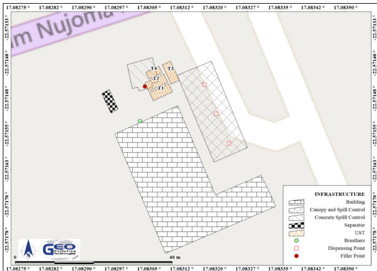
Figure 3-1 Site layout
