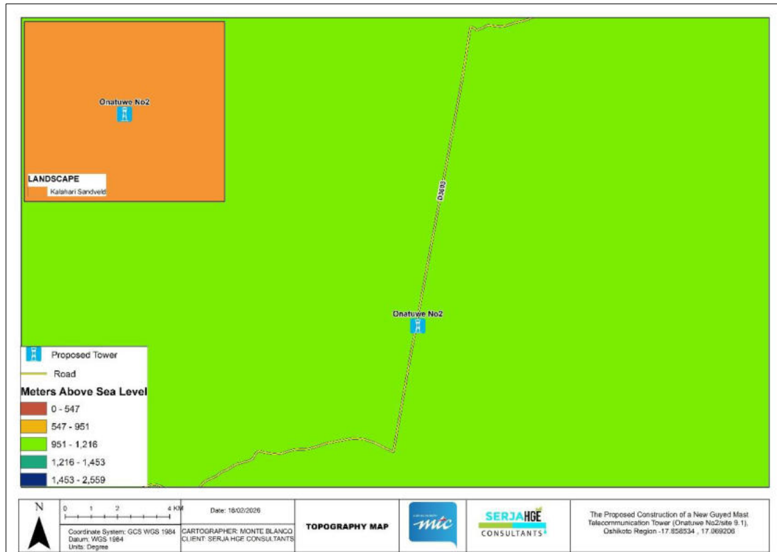
Figure 5-3: The topography and landscape of the area
