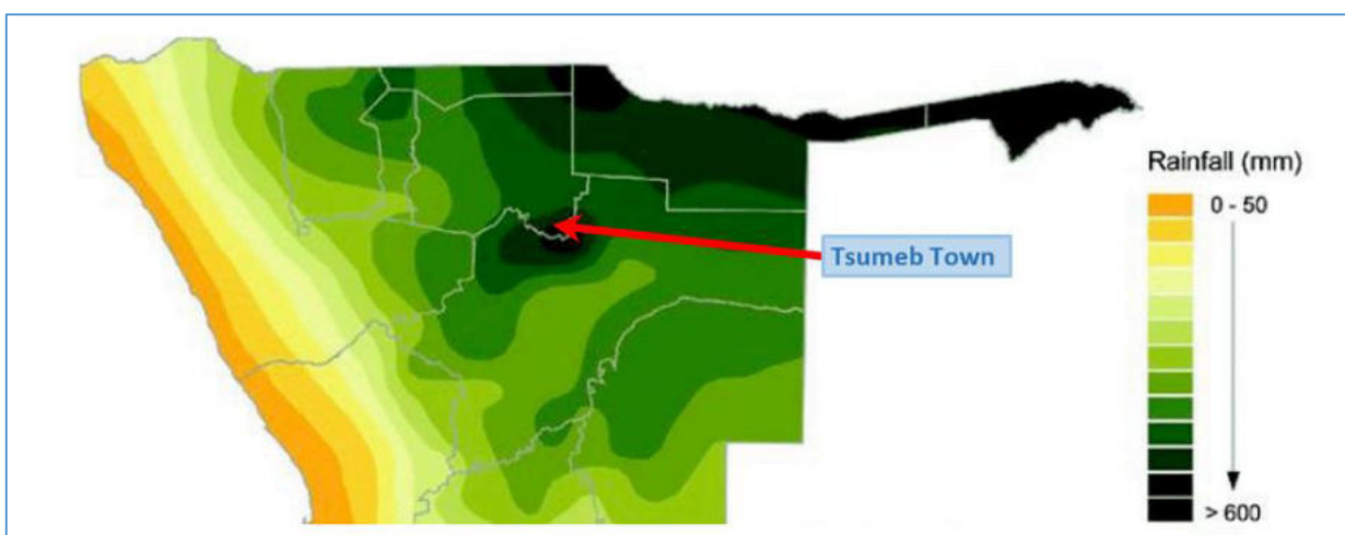
Figure 7: The summary rainfall, with average rainfall at site ranging between 450- and 550-ml pa.
