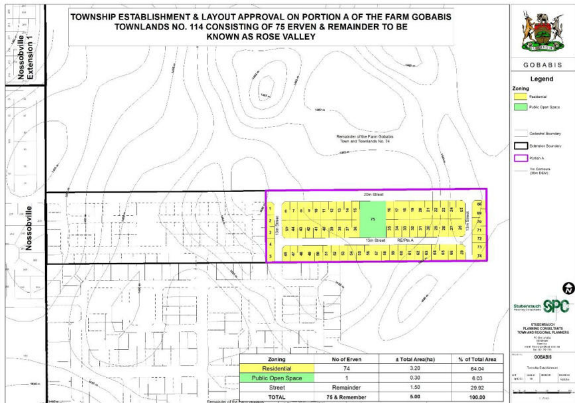
Figure 5: Layout Plan for Rose Valley
