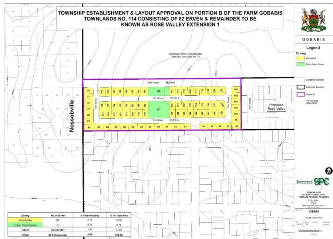
Figure 7: Layout Plan for Rose Valley Extension 1
