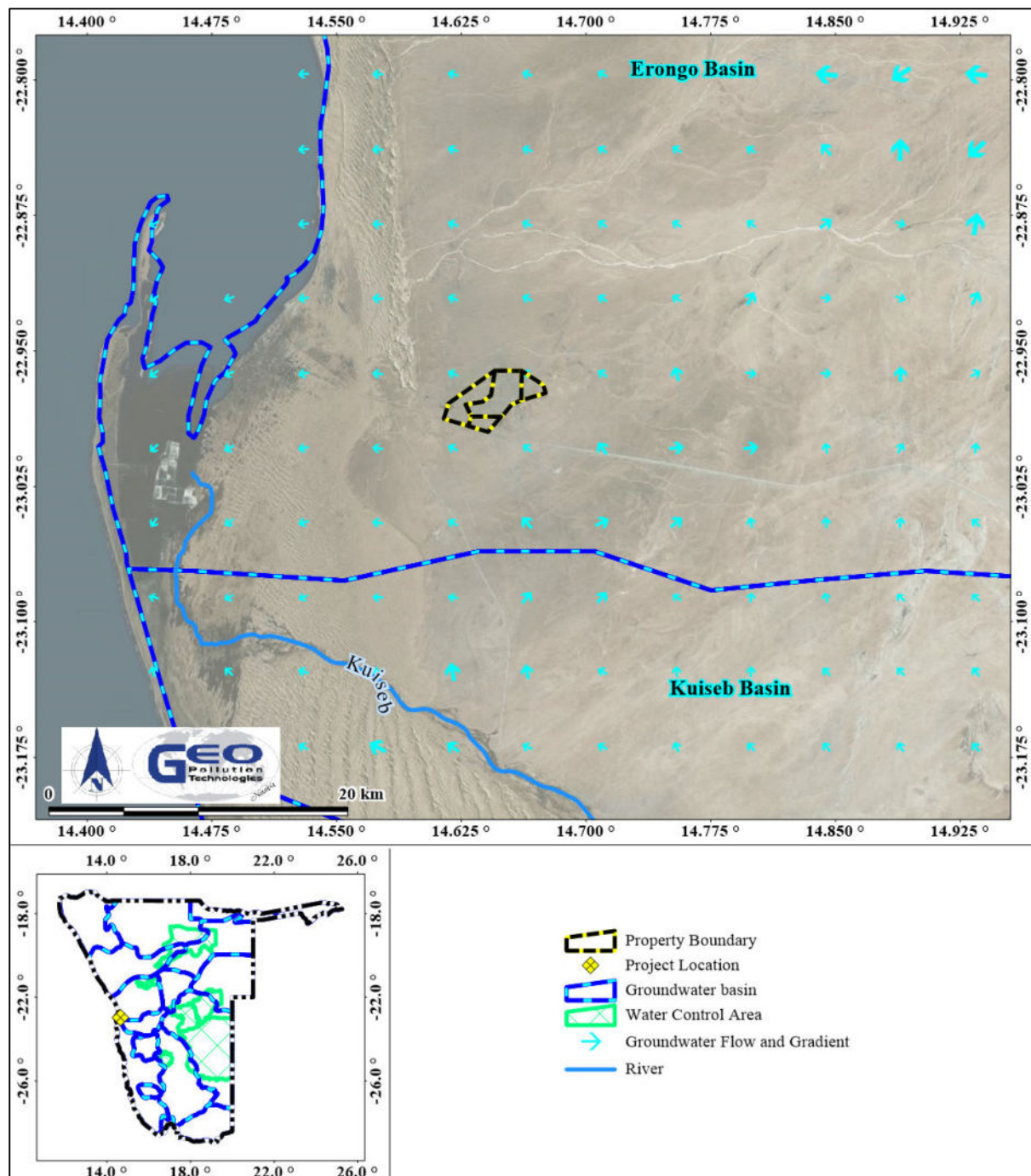
Figure 6-7 Groundwater flow
