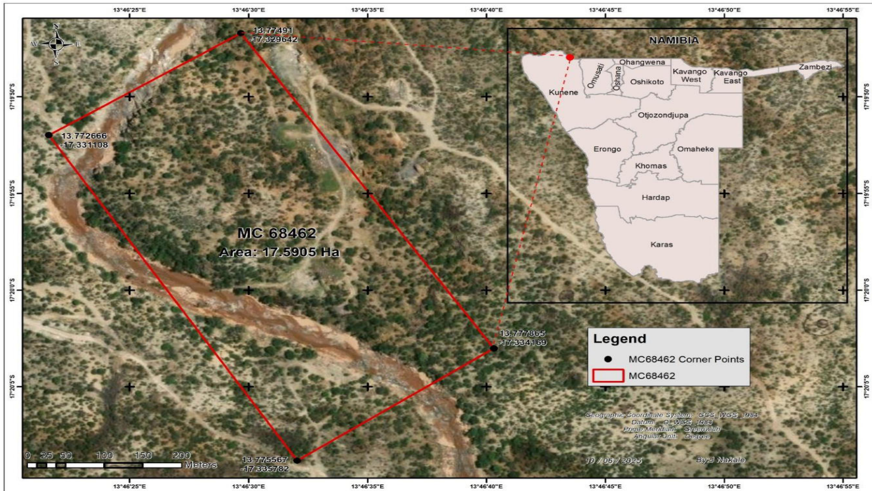
Figure 1: Location of Mining Claim 68462, Oroutumba Village, Opuwo district in Kunene Region (geo-reference point - 17.332222 S, 13.774444 E).
