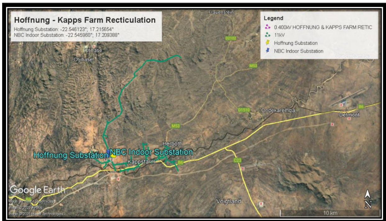
Figure 1: Locality map showing the Hoffnung – Kapps Farm - Hoffnung electrical reticulation system
