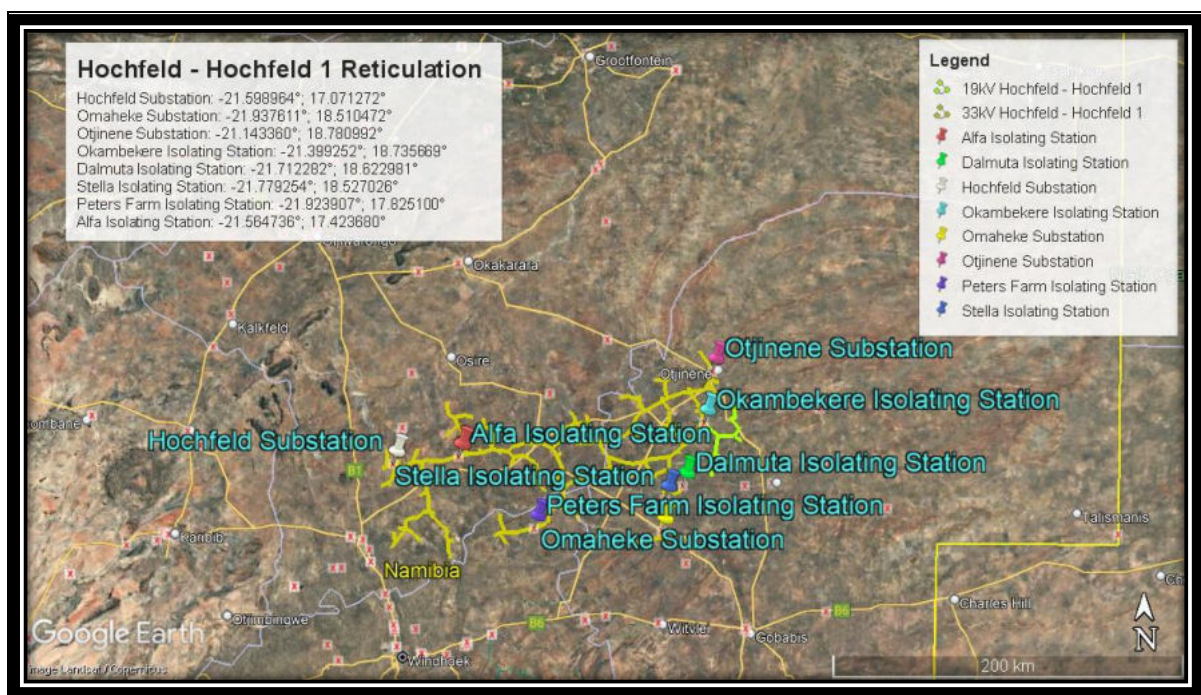
Figure 1: Locality map showing the Hochfeld - Hochfeld 1 reticulation system
