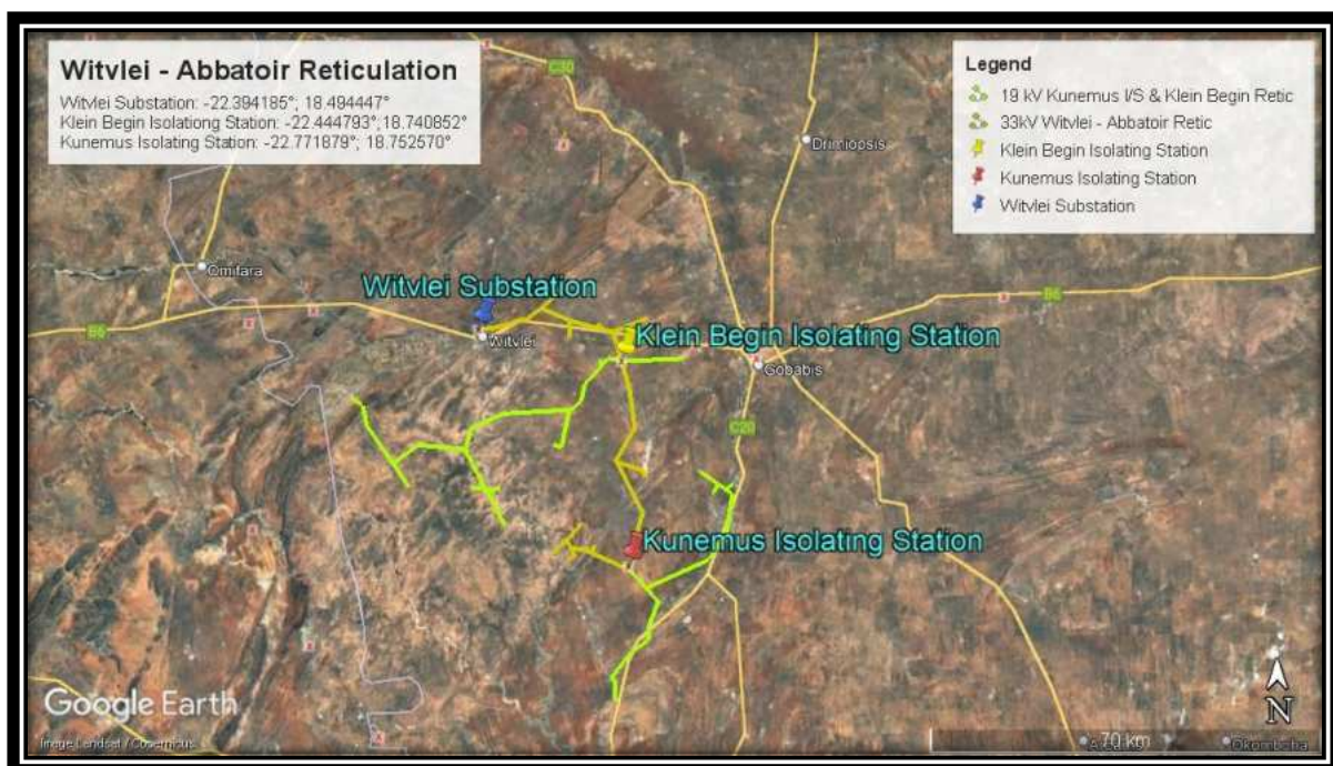
Figure 1: Locality map showing the Witvlei – Abbatoir reticulation system
