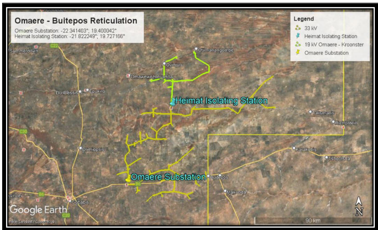
Figure 1: Locality map showing the Omaere – Buitepos - Kroonster electrical reticulation system
