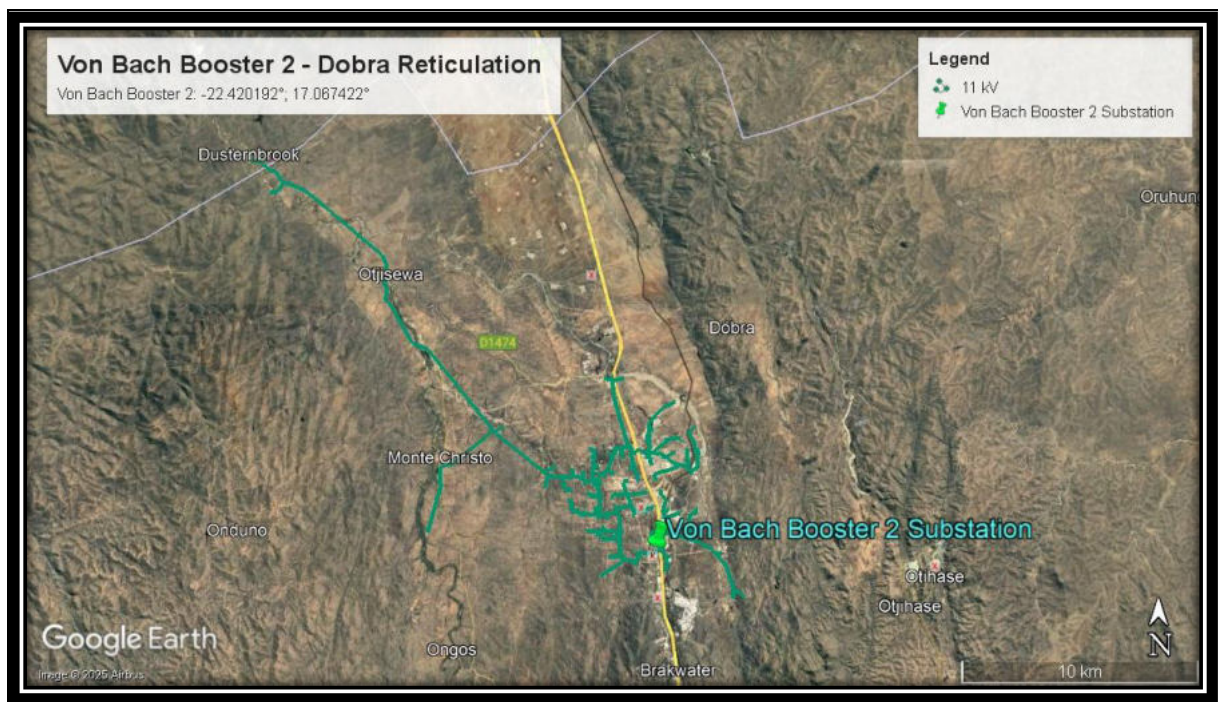
Figure 1: Locality map showing the Von Bach Booster 2 – Döbra - Brakwater electrical reticulation system
