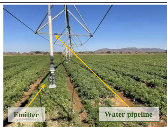
Photo 4-36 Centre pivot system close up
