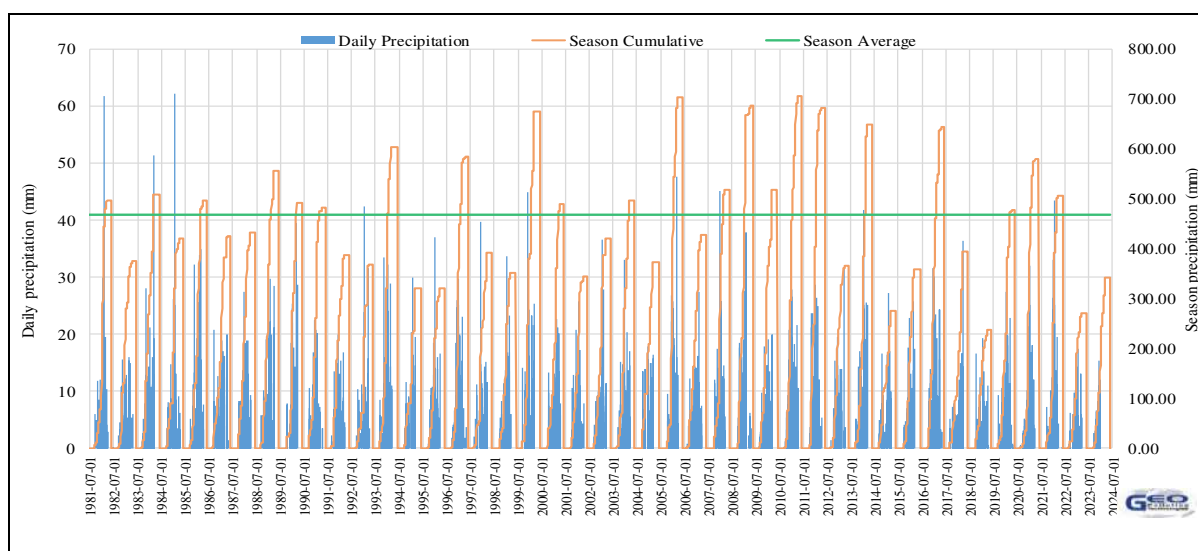
Figure 7-2 Daily and seasonal rainfall (modelld) (Funk et al., 2015)
