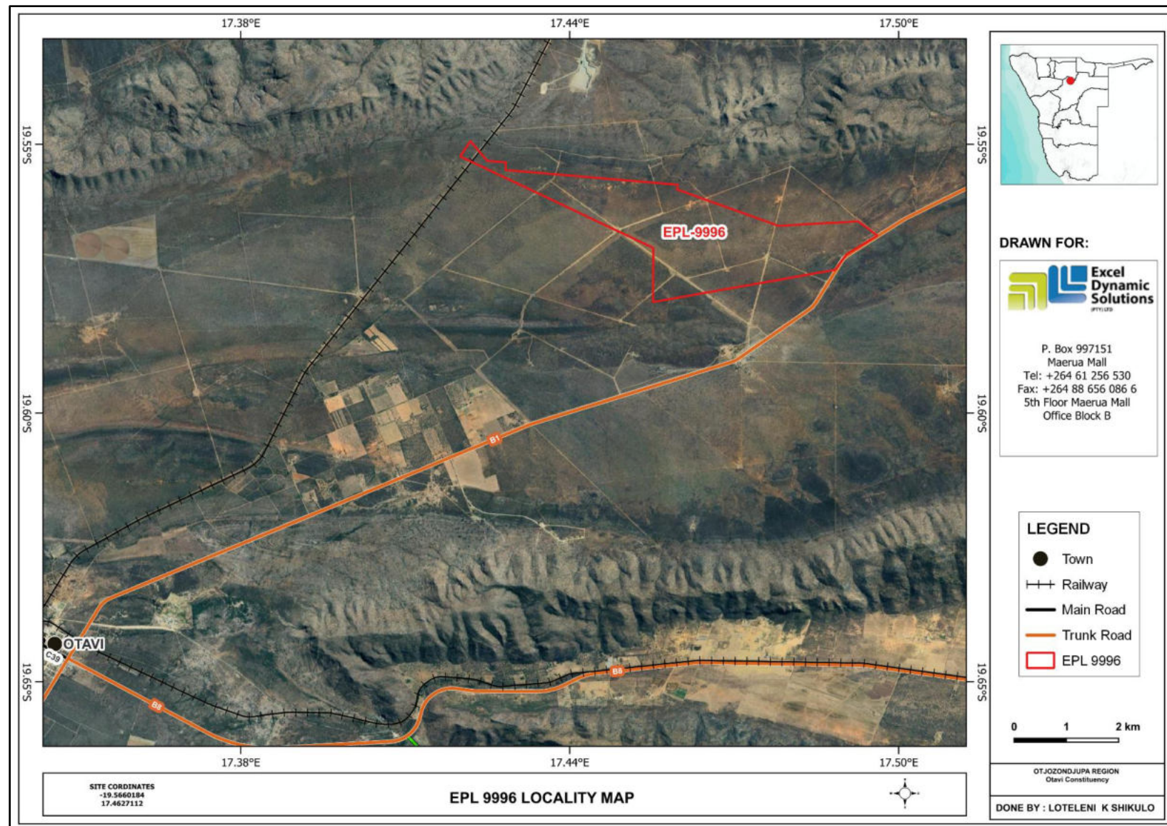
Figure 1: Locality Map for EPL 9996
