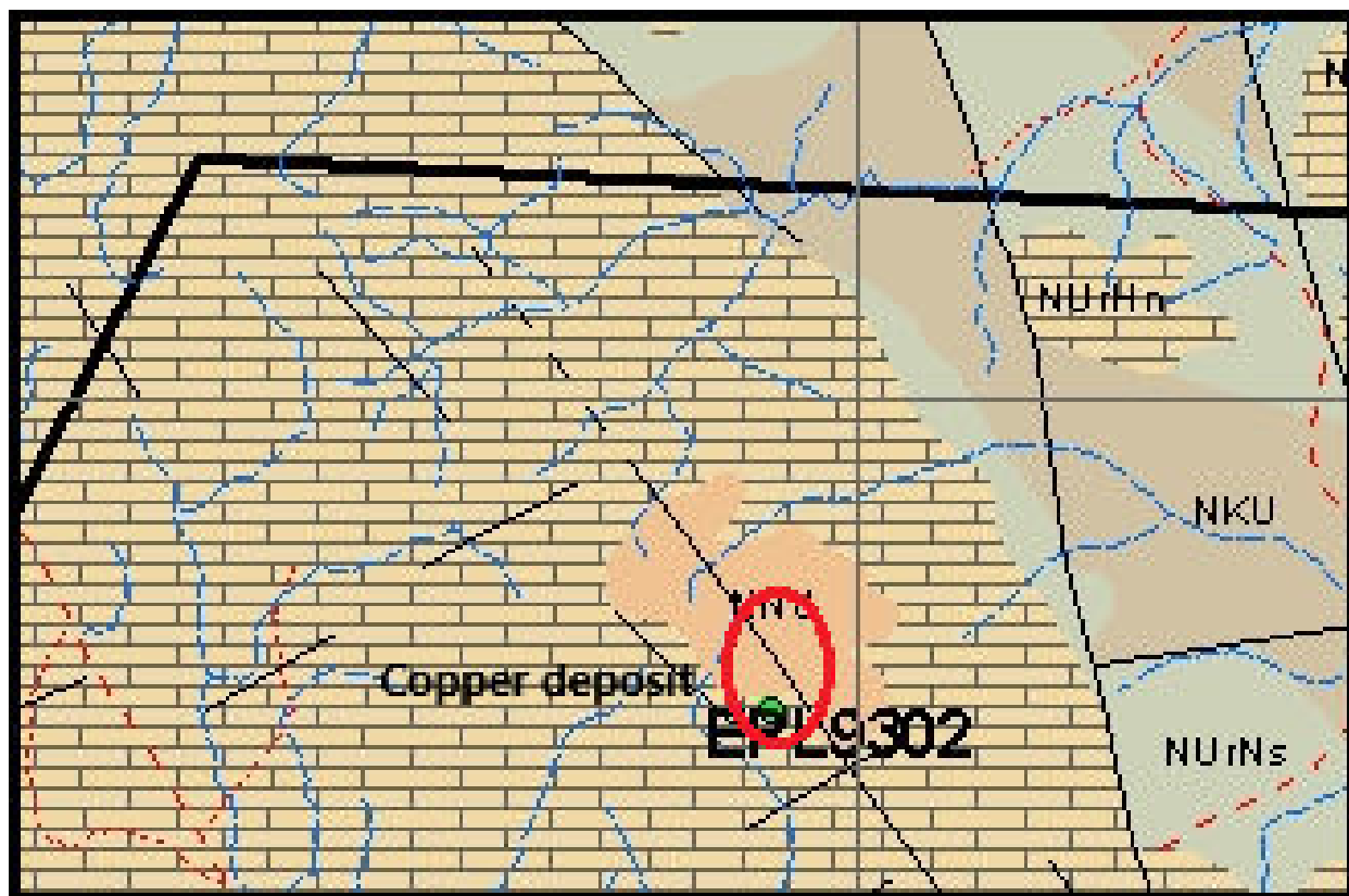
Figure 4.5: The target minerals in epl 9302 (Geological Survey of Namibia,1999)
