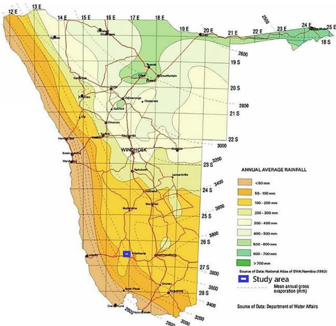
Figure 4.1: Regional climatic patterns of Namibia showing the location of the study area (Directorate of Environmental Affairs, 2002).
