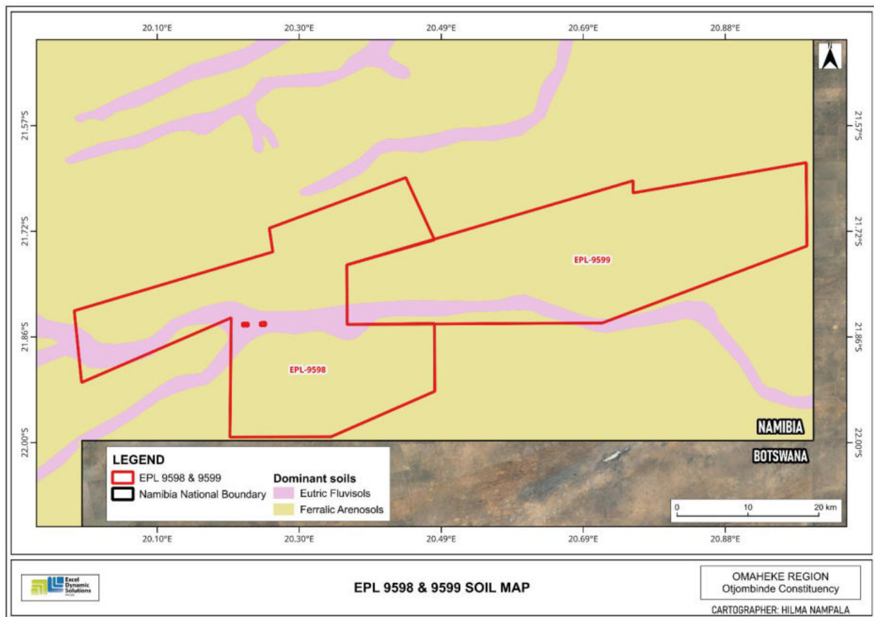
Figure 6: Soils map - EPL 9598 - 9599
