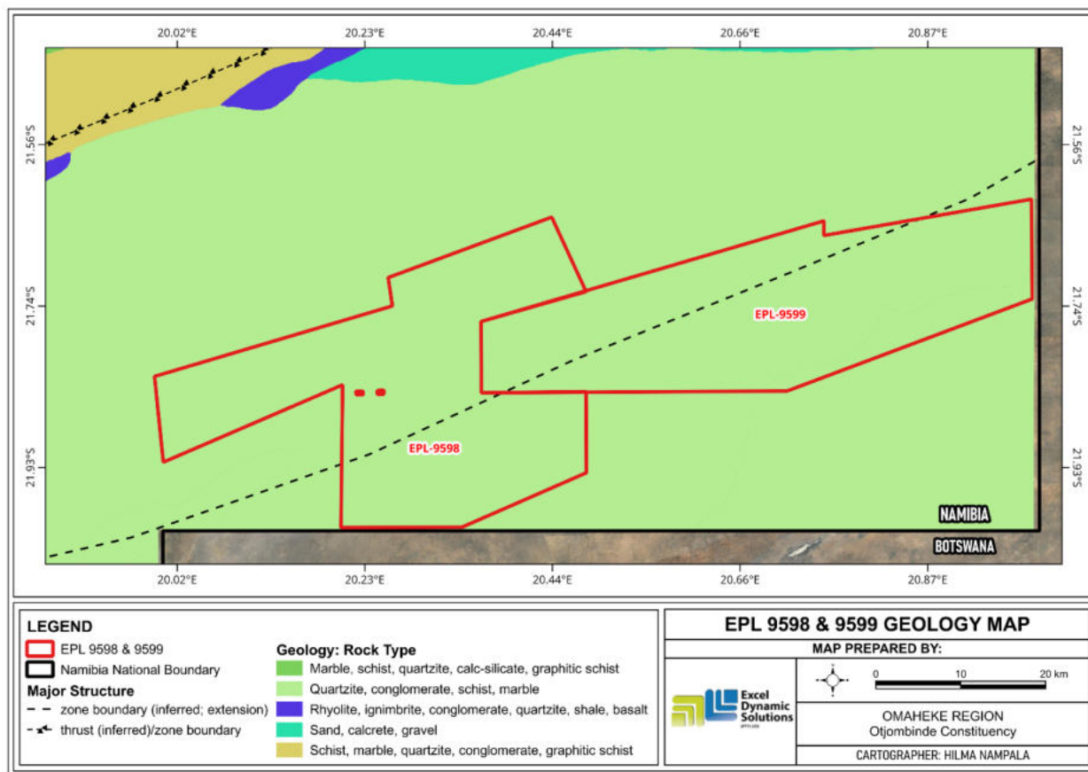
Figure 5: General Geology map - EPL 9498 - 9599
