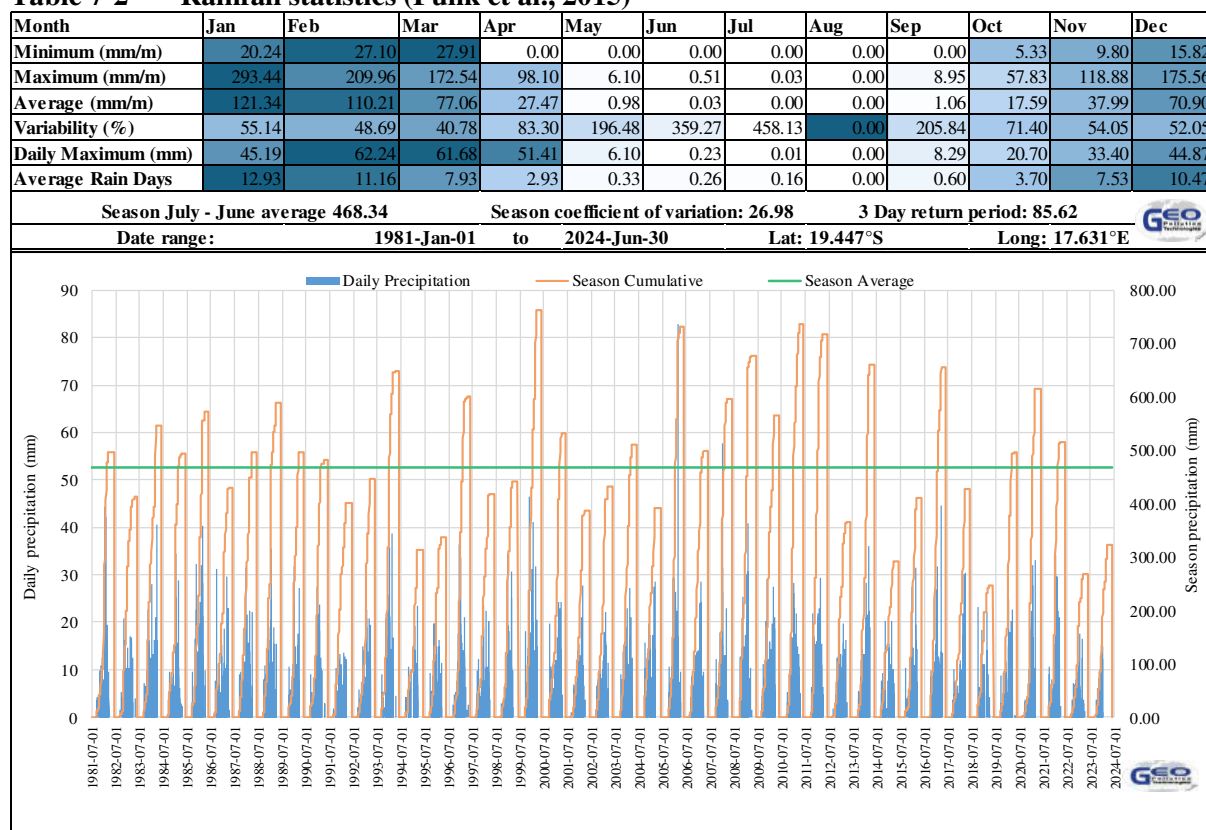
Figure 7-2 Daily and seasonal rainfall (Funk et al., 2015)
