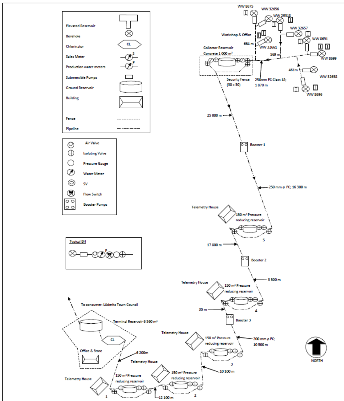
Figure 2: Lüderitz Scheme Schematic Layout
