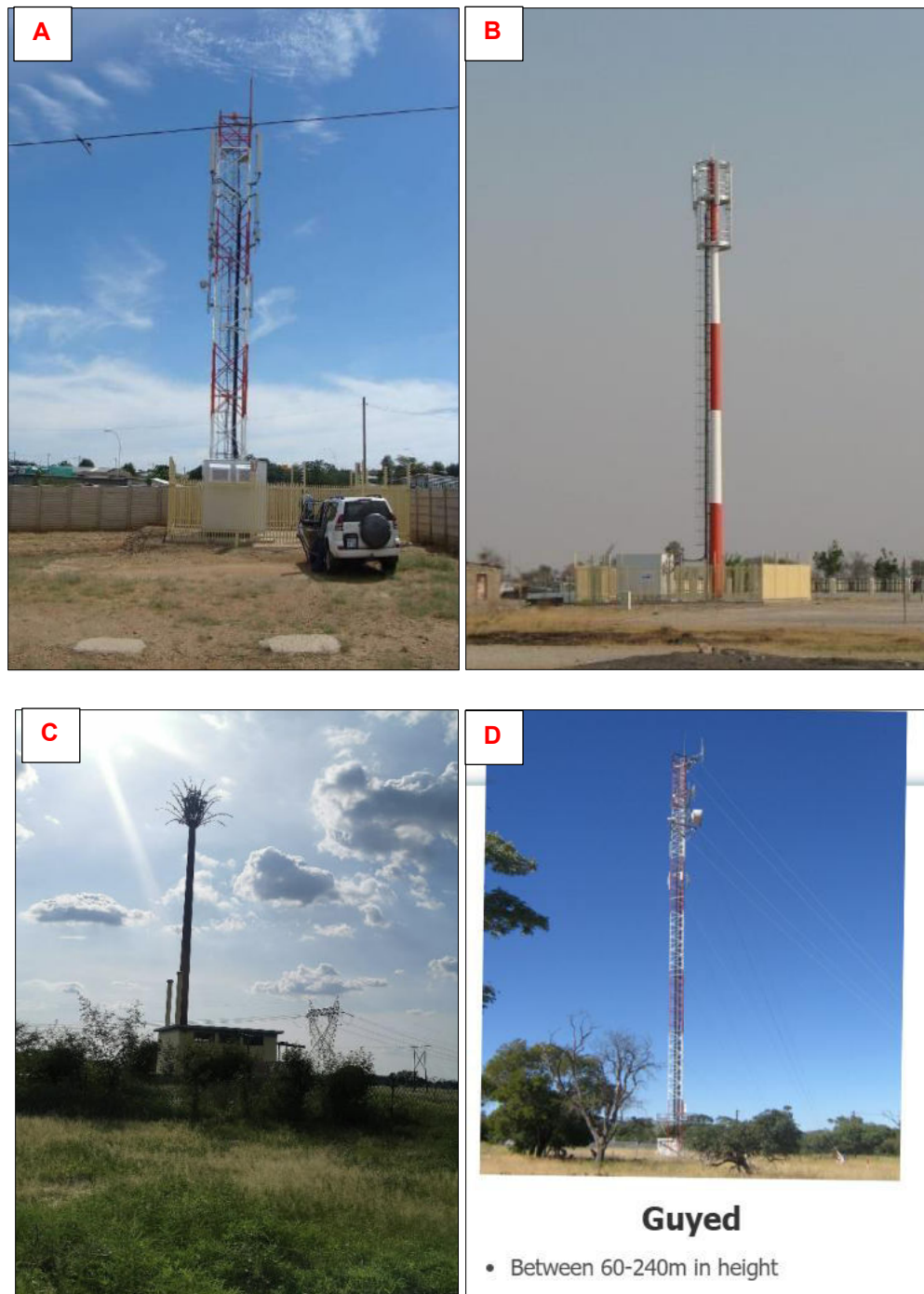
Figure 3-1: Types of network structures: A - Lattice, B - Monopole, C - Camouflage, and D – Guyed
