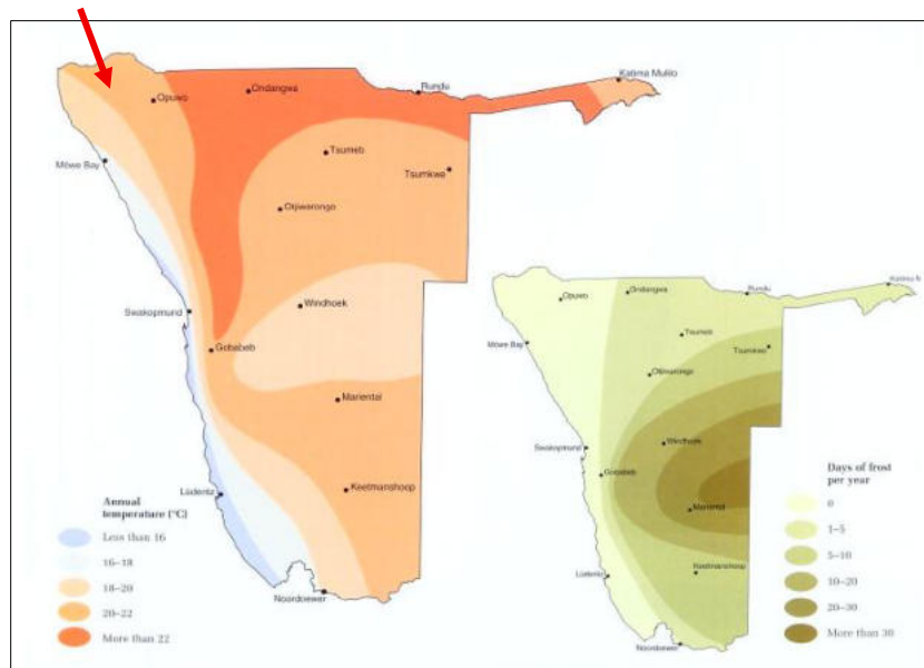
Figure 5-5: The annual temperatures for the project area (Mendelsohn et al. , 2002)
