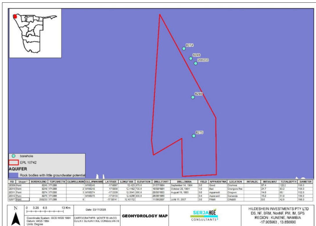
Figure 5-11: The geohydrology (groundwater) map with the existing (database recorded) boreholes near and within the EPL boundaries
