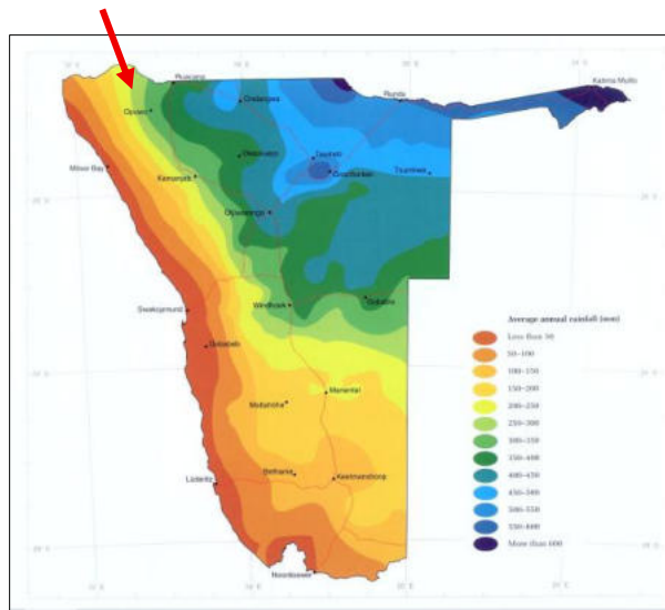
Figure 5-4: The annual rainfall for the project area (Mendelsohn et al. , 2002)
