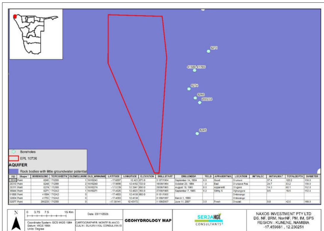
Figure 5-13: The geohydrology (groundwater) map with the existing (database recorded) selected boreholes within a 10km radius of the EPL boundaries
