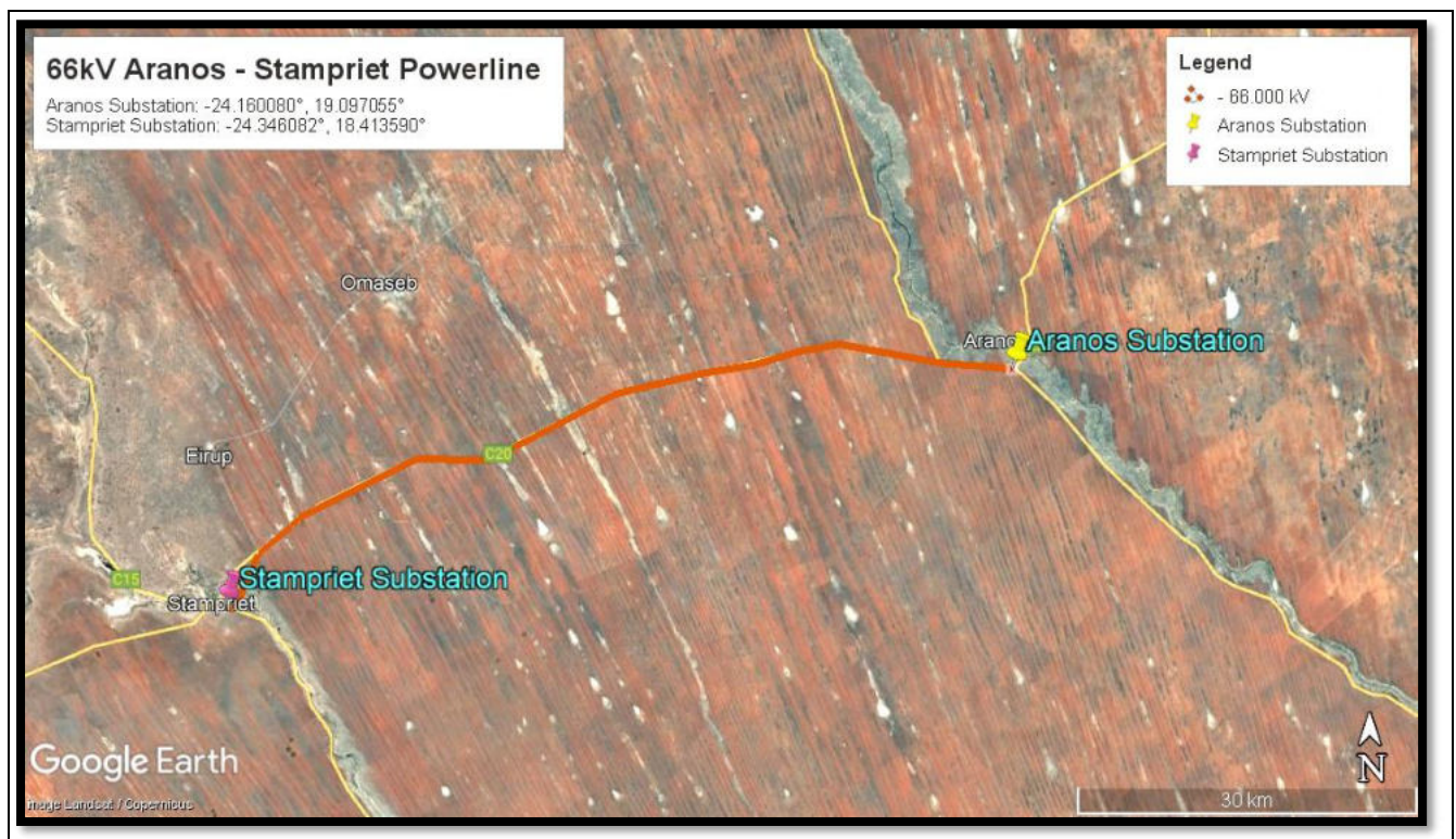
Figure 1: Locality map showing the 66kV Aranos - Stampriet transmission line
