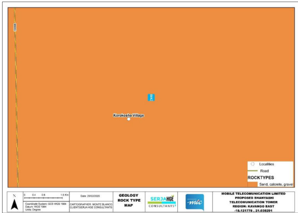
Figure 5-4: The geology of the site area
