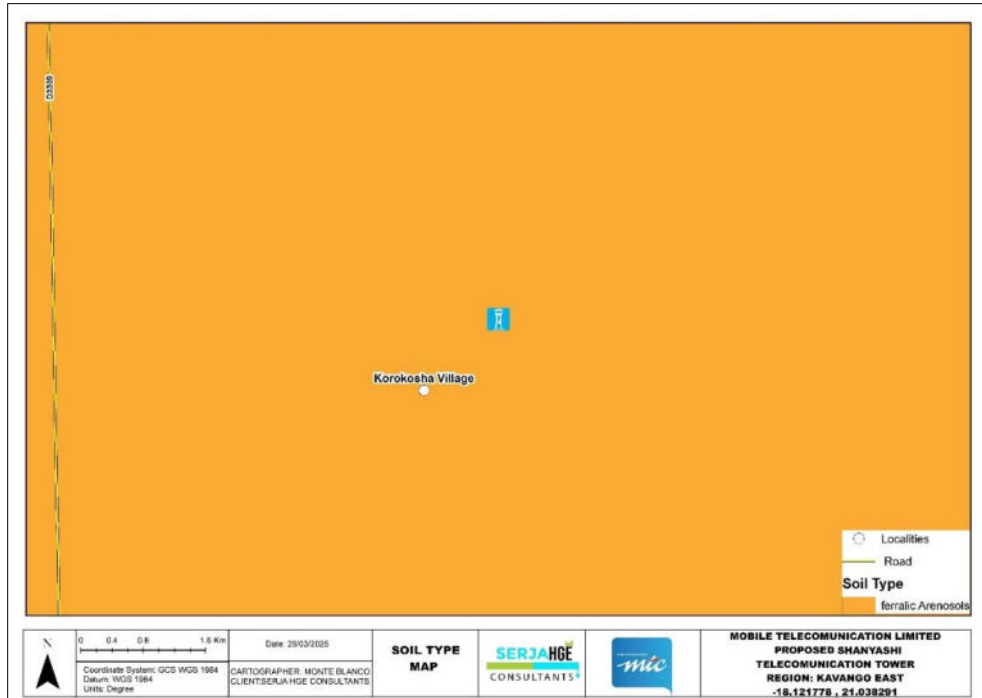
Figure 5-5: The dominant soil types around the site
