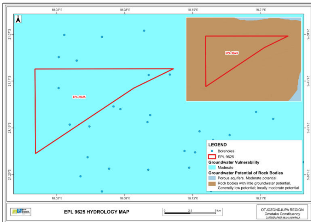
Figure 8: Hydrology map for EPL 9625
