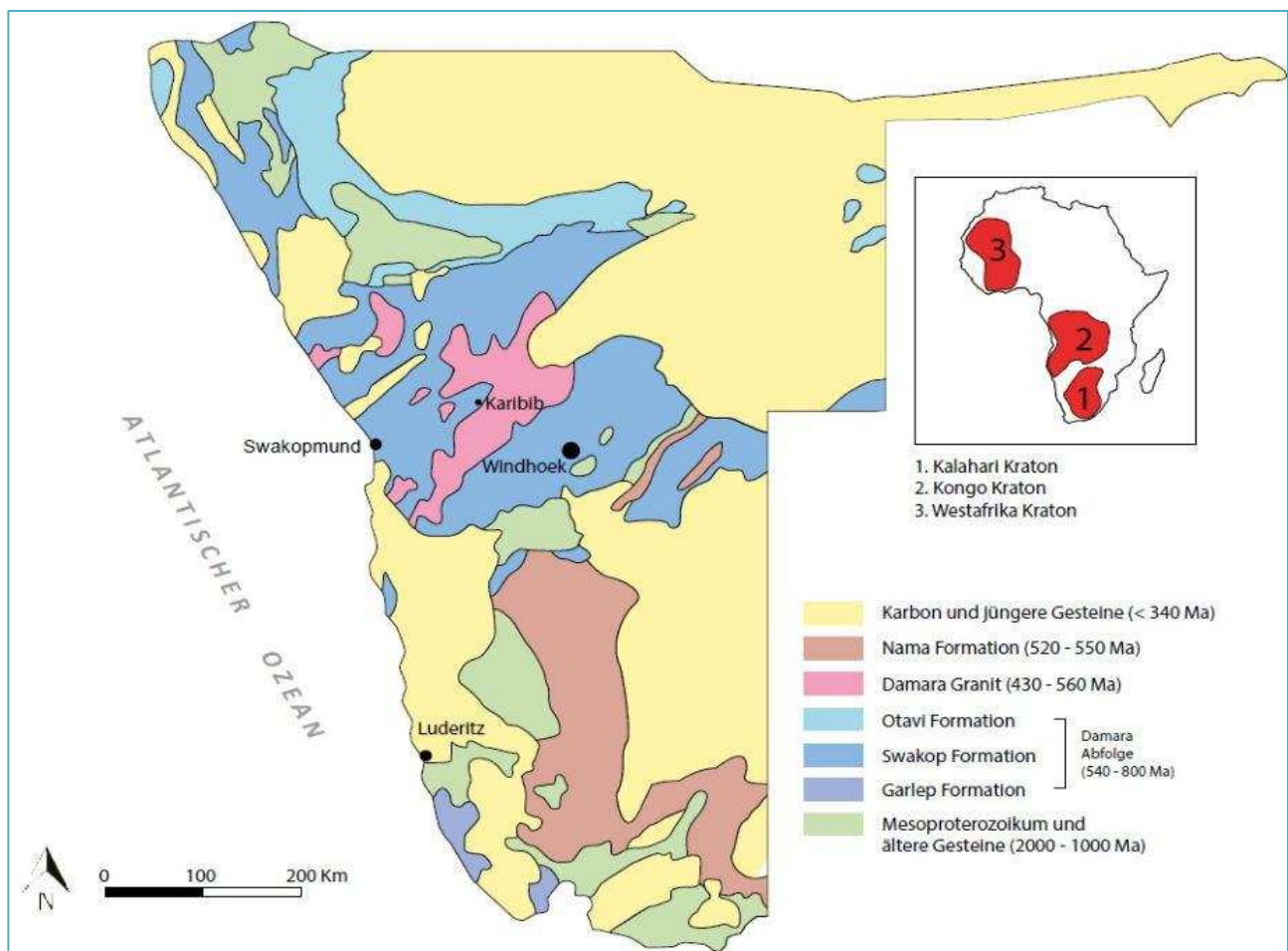
Figure 10: Simplified geology of Simplified geological map of Namibia. Modified after Clifford (2008).
