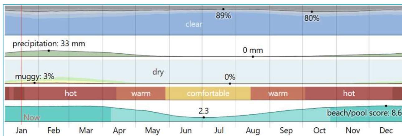
Figure 6: The summary of the climate at Keetmanshoop by month, //Karas Region
