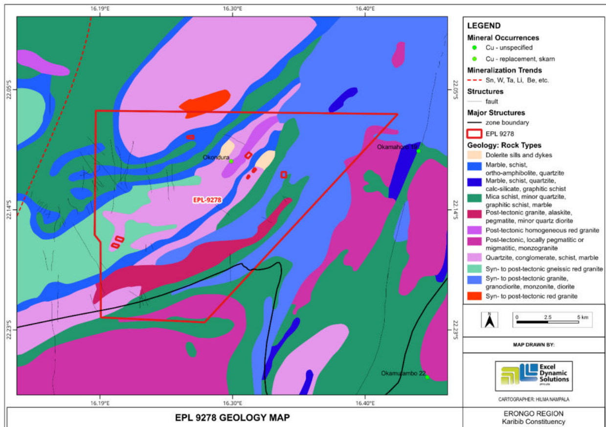
Figure 5: General Geology map for EPL 9278
