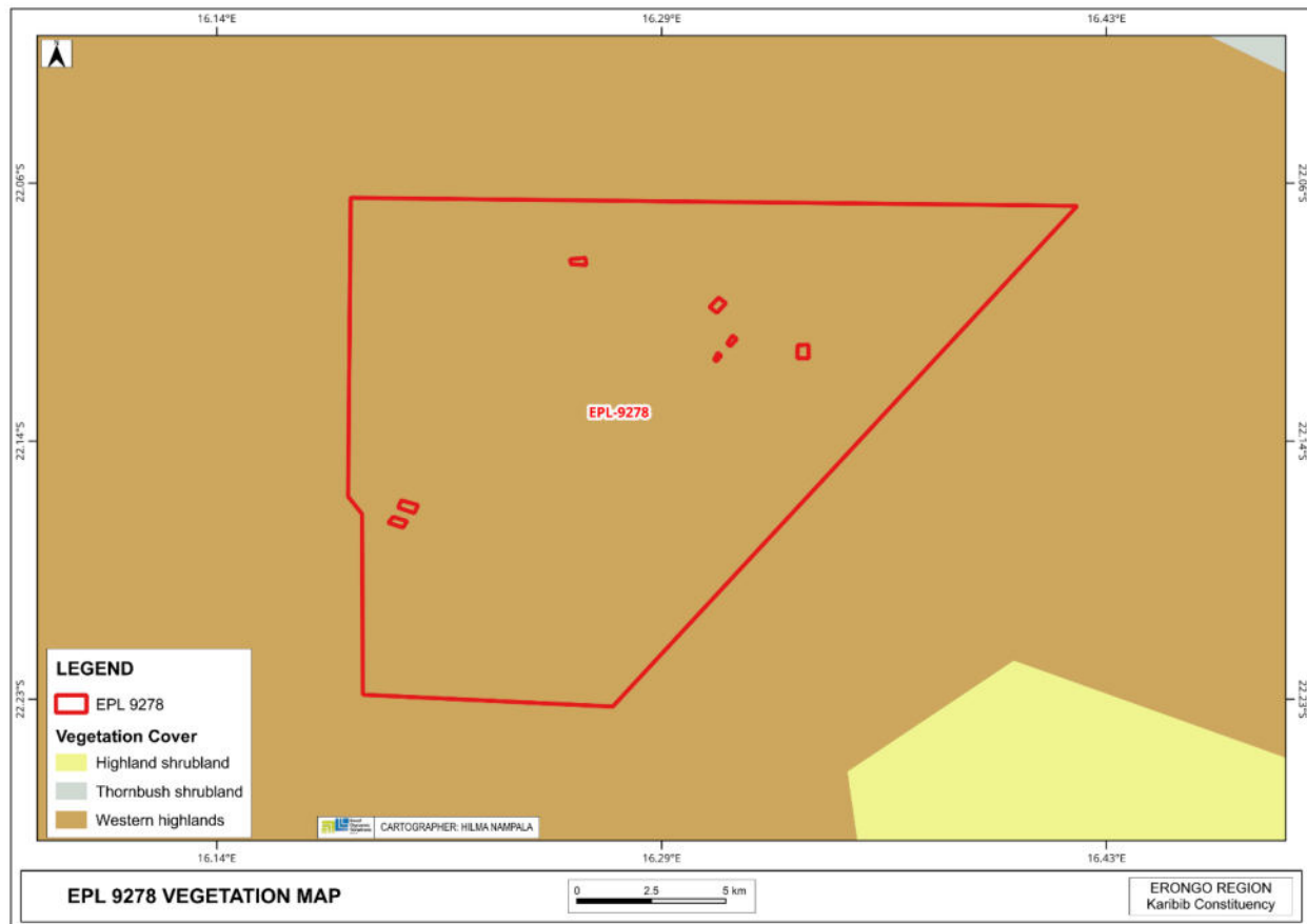
Figure 8: Vegetation map - EPL 9278
