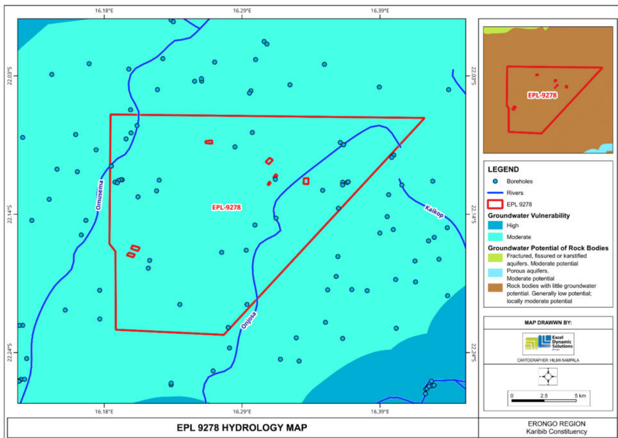
Figure 7: Hydrology map for EPL 9278
