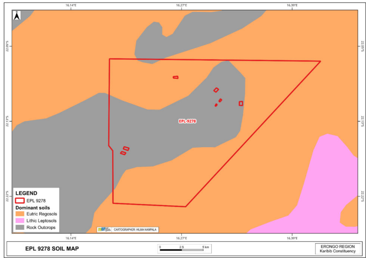
Figure 6: Soils map for EPL 9278
