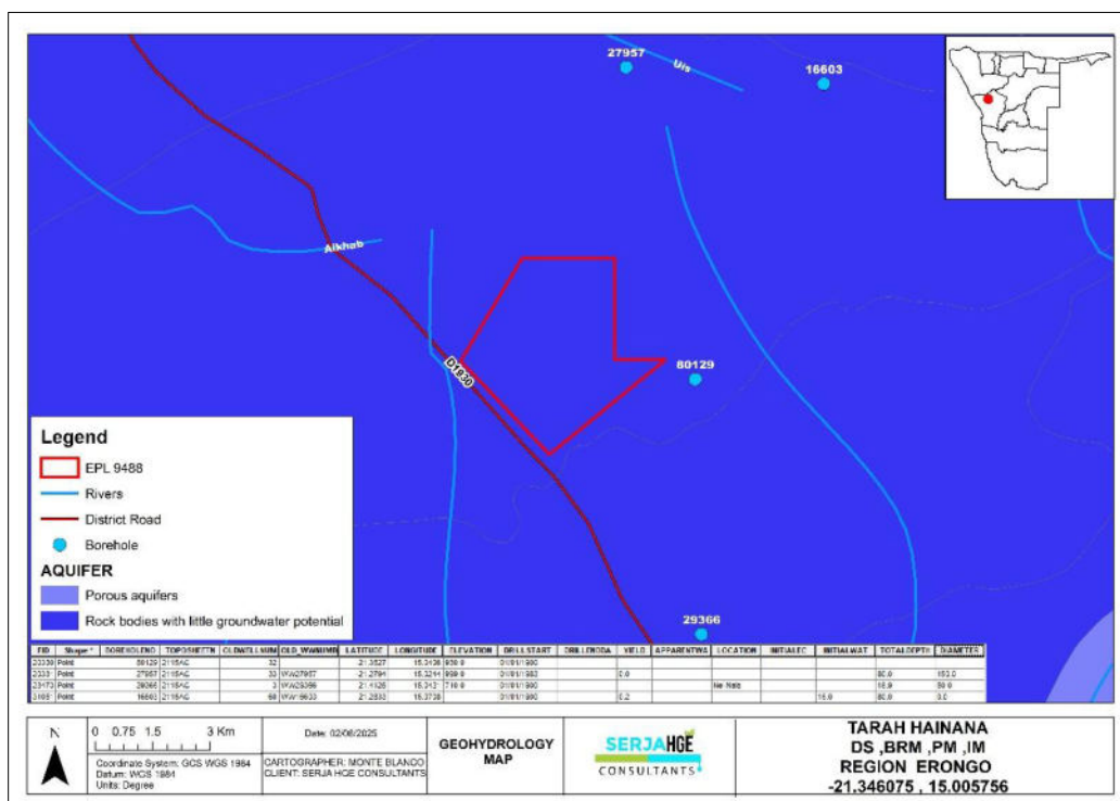
Figure 5-13: The surface and groundwater map of the EPL area
