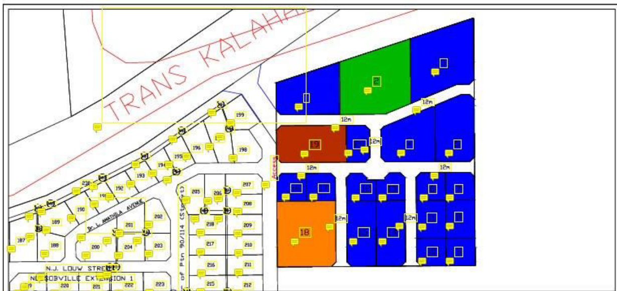
PROPOSED LAYOUT PLAN OF PORTION 165 OF THE REMAINDER OF THE FARM GOBABIS TOWN AND TOWNLANDS NO. 114 TO BE KNOWN AS NOSSOBVILLE EXTENSION 3
