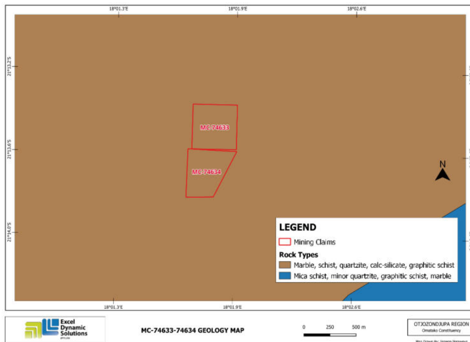
Figure 5: General geology and lithology map of the MCs.
