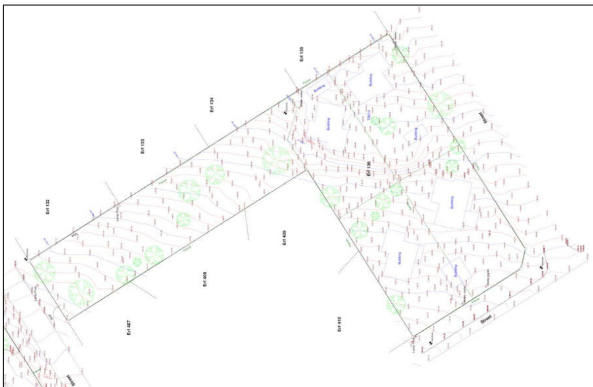
Figure 17: Topographic survey of Erf 136 Karibib (Namib Geomatics Technologies, Sept 2021)
