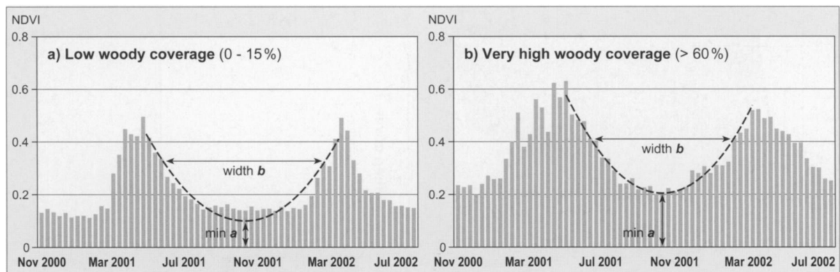
Fig. 5: NDVI trajectories (bars) for areas with low woody coverage (a) and high woody coverage (b) and corresponding polynomial curve fit
