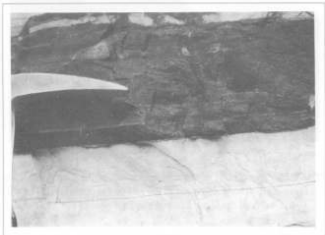
Plate 2.E: In many instances there is no evidence of compositional grading in the white marbles and they rather have a sharp contact with the overlying black schist giving the appearance of a Zebra rock (cf. Plate 2.C).
