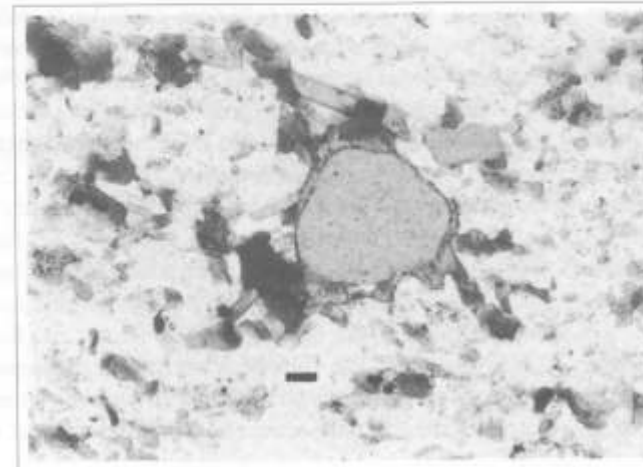
Plate 9.D: Overgrowth of tourmaline on a well-rounded detrital tourmaline grain. Scale bar 0.2 mm.
