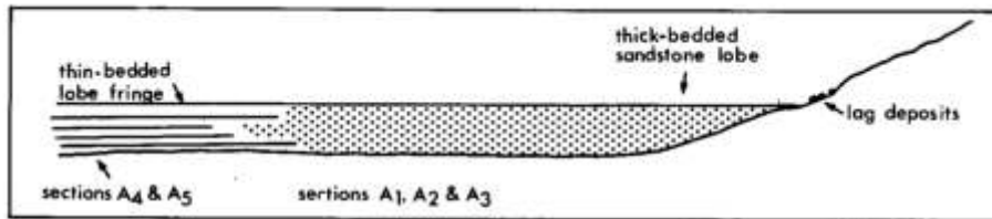
Fig. 3.30: Proposed model for the deposition of the Amis River Formation. The system developed by aggradation, not progradation, and is similar to the type I system of Mutti (1985). This type of system requires a major input of sand.
