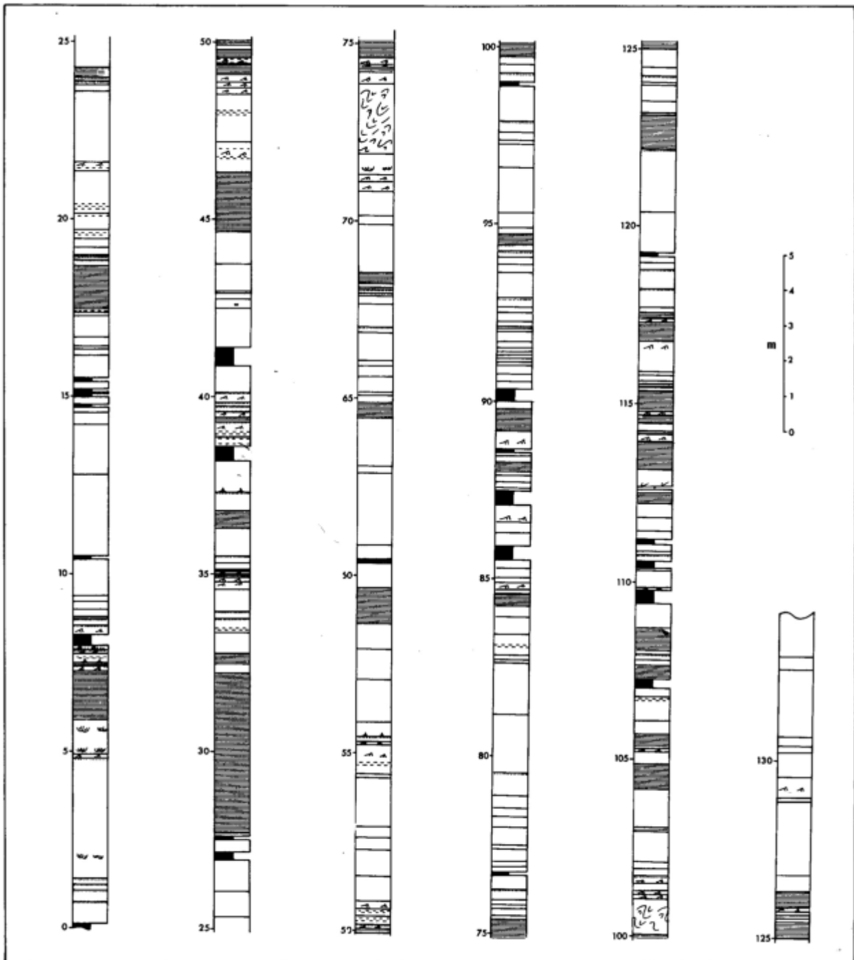
Fig. 3.10: Sedimentary log of the Brak River section.
