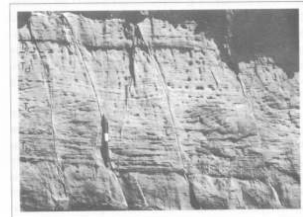
Plate 5.F: T bede sequence in the Amis River Formation (locality: Lonely River section).
