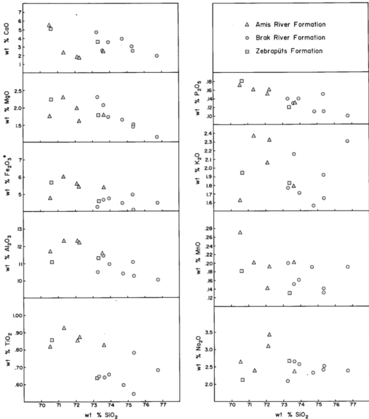
Fig. 4.1: Harker variation diagram for the analysed samples of Zerrissene greywackes.
