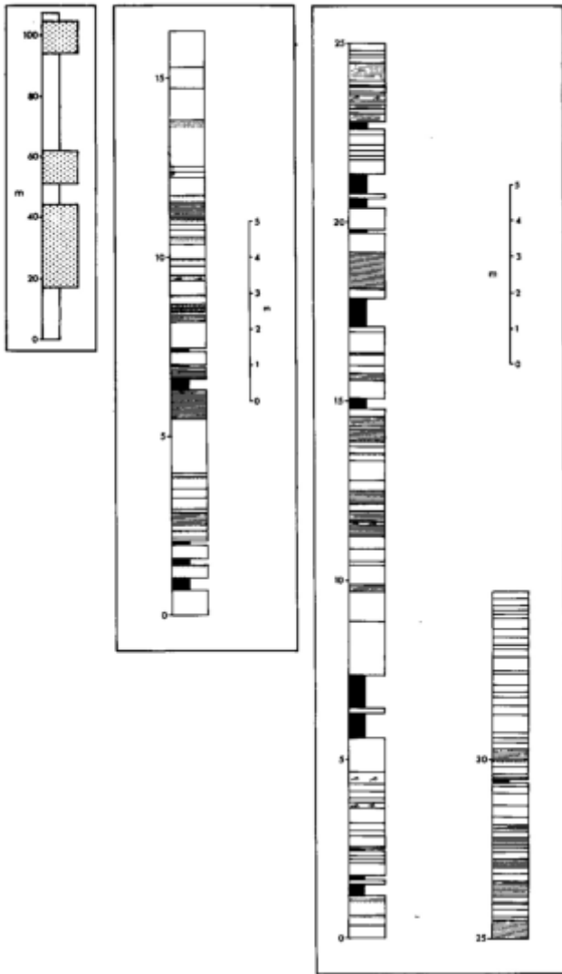
Fig. 3.26 (left): The same facies groups found in the Jeppie east and west sections are found in the Lonely River section. These groupings are shown here. See Fig. 3.22 for key.
