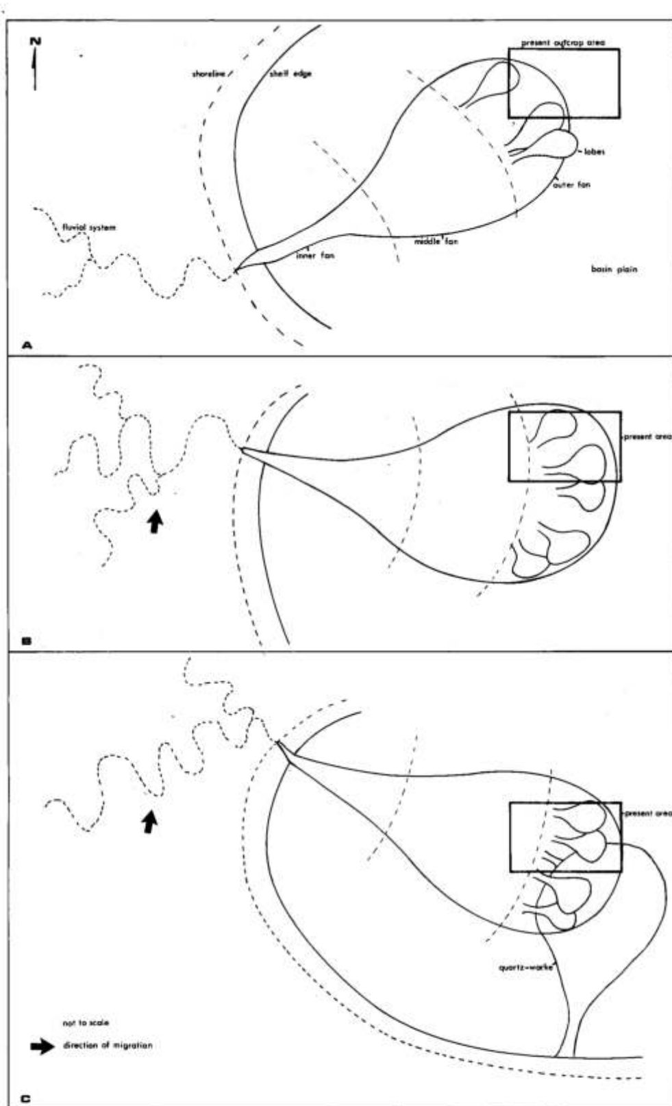
Fig. 5.2: Cartoon illustrating the envisaged evolution of the Zerrissene siliciclastic deposits. The lack of reliable palaeocurrent indicators in the carbonates precludes development of a similar model for their development. Notably only the distal parts of the siliciclastic system are preserved in the lower Ugab River area. Firstly, an open ocean appears to have been already fully developed by the time that the turbidites of the Zebra pits Formation were deposited (a). The next episode (b) of siliciclastic sedimentation, the Brak River Formation, also occurred on an unconfined ocean floor, and was accompanied in its later stages by a glacial period. The final stage (c) of exposed sedimentation possibly developed in a more restricted basin with a voluminous sediment supply. Indications of lateral sources are the presence of the coarse-grained quartz-wacke beds interbedded with the distal sediments in the east.
