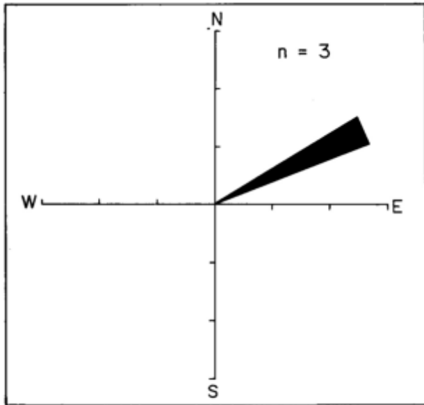
Fig. 4.7: Palaeocurrent rose diagram (in 10° sectors) for the Zebrapüts turbidites. This formation has few directional structures.
