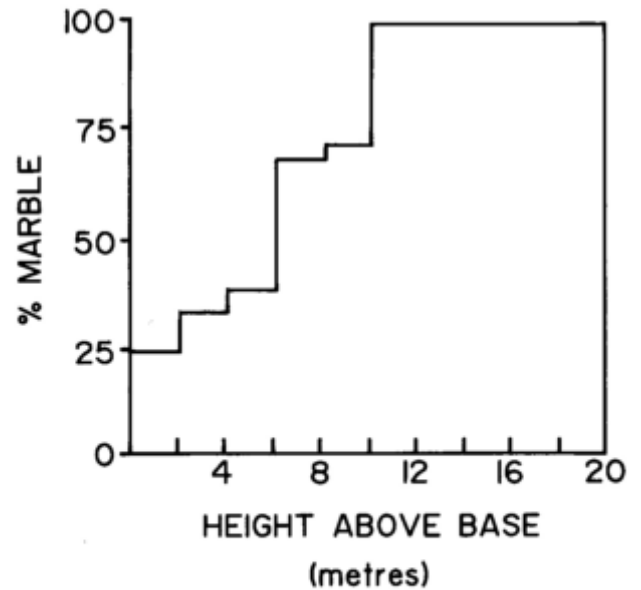
Fig. 2.4: Histogram showing the progressive increase in carbonate content with height in the section depicted in Fig. 2.1.
