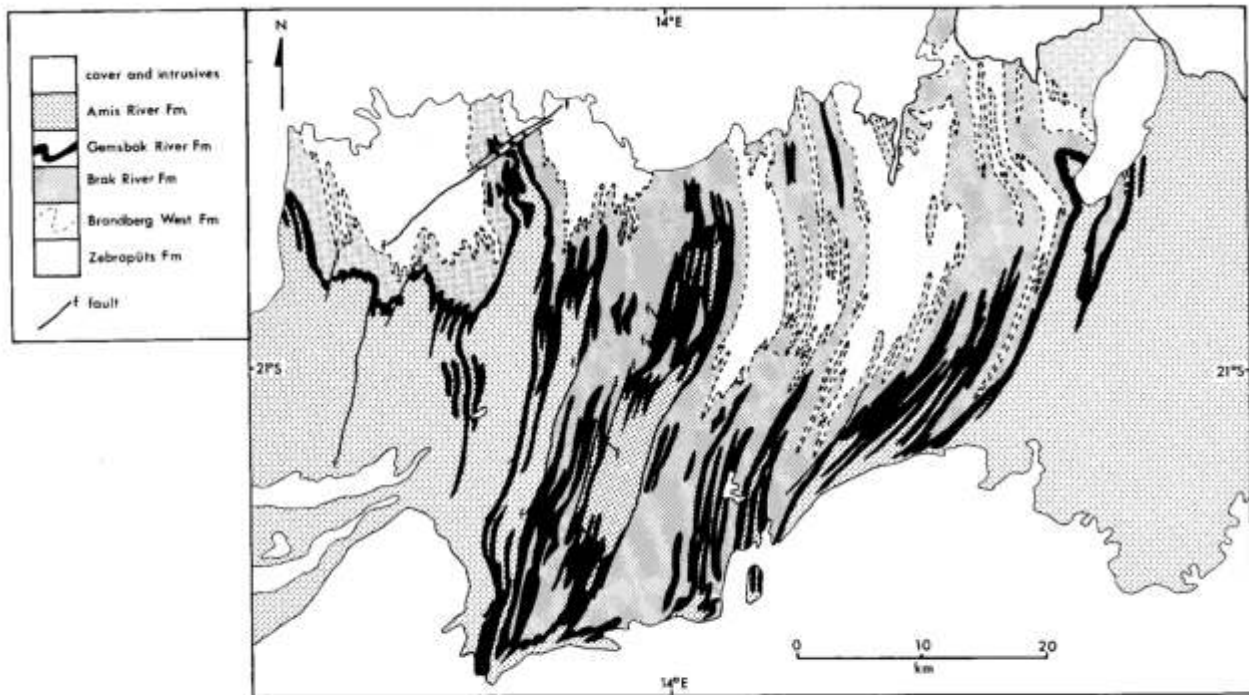
Fig. 1.4: Simplified geological map of the Zerrissene basin (after Geological Map of the Damara Orogen, 1988). The tight folding is clear from the repetition of the various units.
