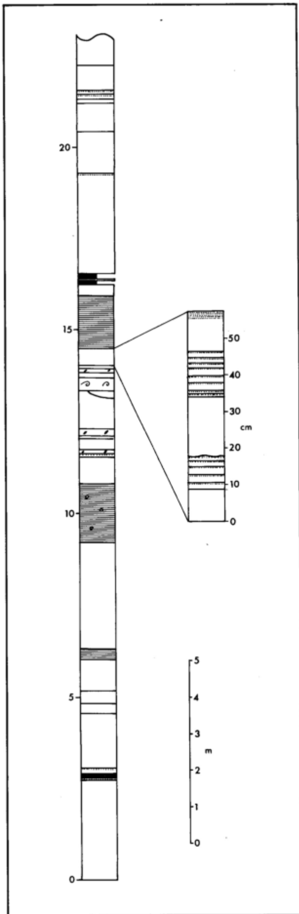
Fig. 3.12: Sedimentary log of the Shelter section of Brak River Formation.
