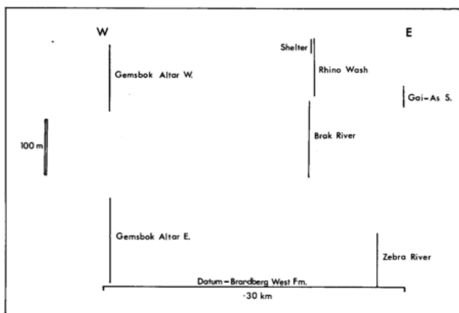
Fig. 3.18: Relative stratigraphic positions of the various measured sections of the Brak River Formation, using the uppermost blue marble of the underlying Brandberg West Formation as a datum, and projected onto an east-west line. Unfolding of the north-south oriented folds will significantly increase the distance between sections
