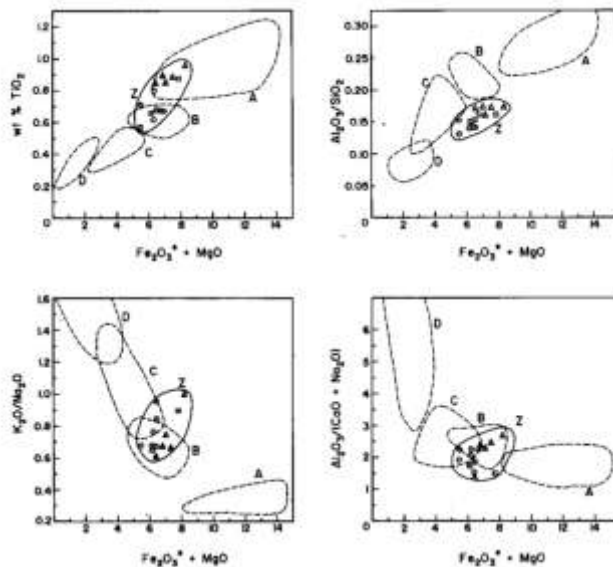
Fig. 4.6: Various plots of major element ratios are used for tectonic setting discrimination of greywackes. Shown here are the Zerrissene data plotted on the diagrams proposed for this purpose by Bhatia (1983). Symbols as for Fig. 4.1. The key to the tectonic setting is: A - oceanic island-arc; B - continental island-arc; C - active continental margin; D - passive margin; Z - Zerrissene greywacke. See text for discussion.
