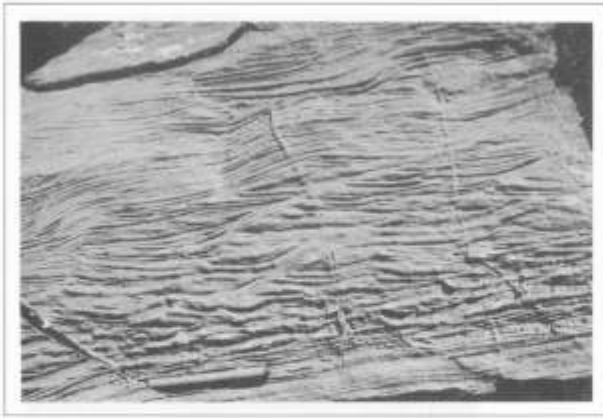
Plate 3.A: Well-developed ripple lamination in silicified facies Cc beds in the Gemsbok River Formation (locality: 2 km south of Ugab River in Brak River).
