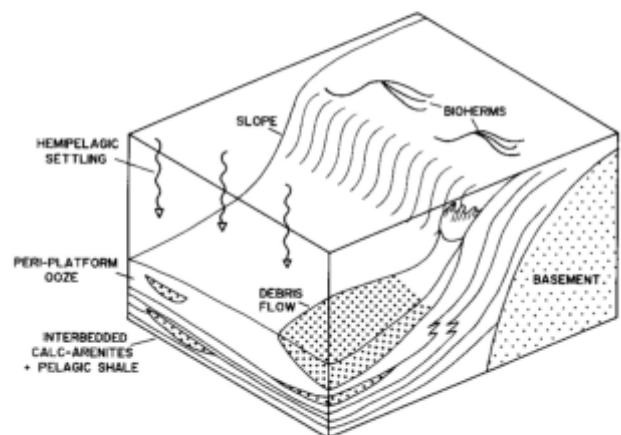
Fig. 2.7: Block diagram illustrating features of the probable palaeogeography during deposition of the Brandberg West and Gembok River Formations.
