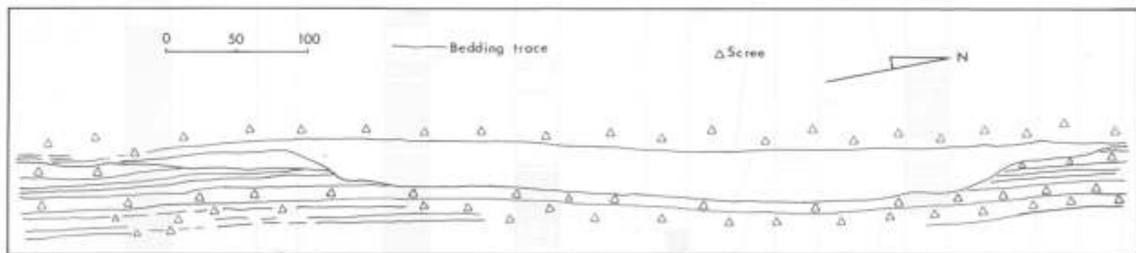
Fig. 3.19: Interpretation of the area around the channel in the aerial photograph shown in Plate 8.A.
