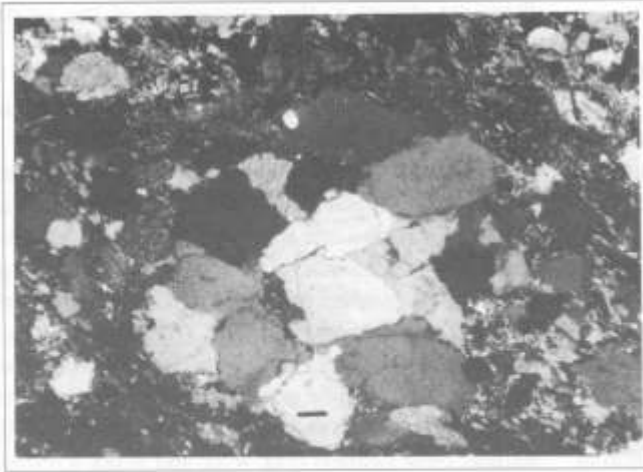
Plate 9.A: Photomicrograph of a quartz-arenite clast which shows well-developed, optically continuous overgrowths on individual quartz grains (sample UR 6/87). Scale bar 0.1 mm.
