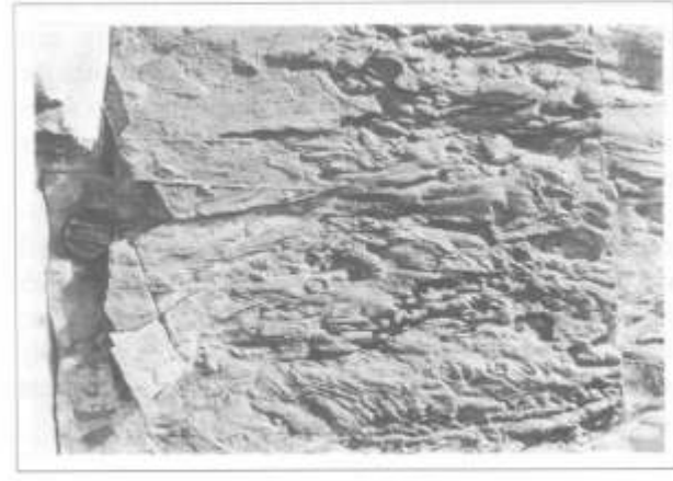
Plate 5.D: Load structures at the base of a thin facies D 1 bed (locality: east of Lonely River Section).
