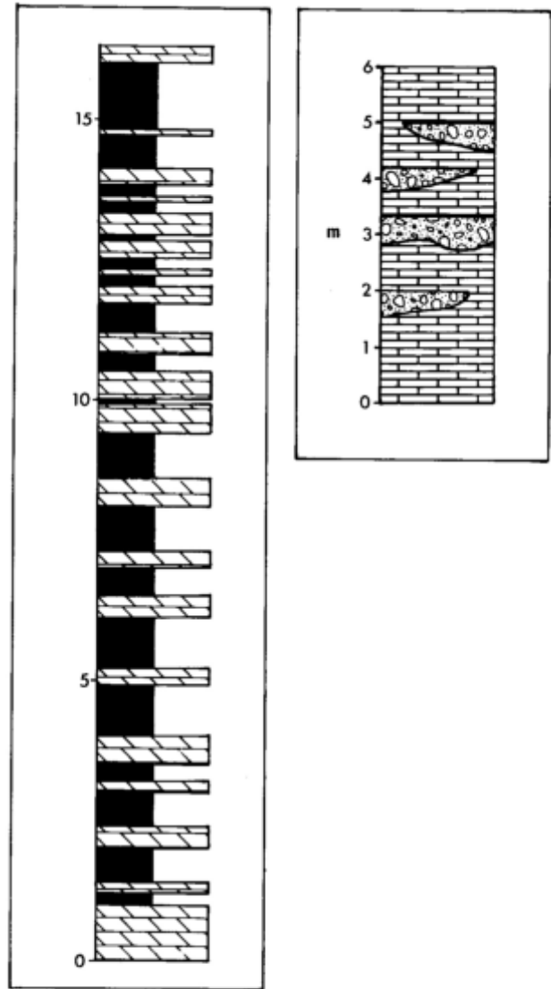
Fig. 2.6: The corner section of the Gembok River Formation.
