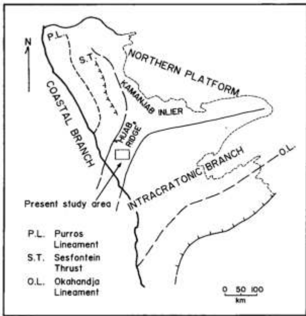
Fig. 1.7: Map showing position of assumed "Huab Ridge" of Porada (1983). This basement high is situated over the current study area.
