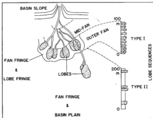
Fig. 3.4: Submarine fan model showing different types of lobe sequences as defined by Pickering (1981). Type I sequences develop by continual switching and stacking of lobes to produce sand-dominated sequences, whereas intermittent, irregular progradation of lobes over the basin plain produces mud-rich sequences, or type II (from Pickering, 1981, his Fig. 9).
