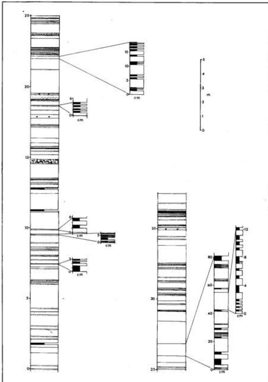
Fig. 3.2: Graphic log of the Ridge 6 section through the Zebrapüts Formation. The section is dominated by facies D 1 with a high sand:shale ratio. Most beds are capped by a very thin pelitic top. For the key to all sections of the siliciclastics see Fig. 3.3.
