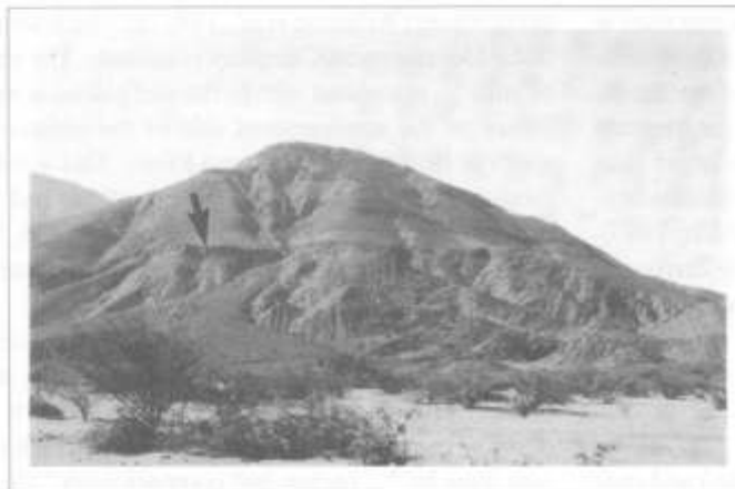
Plate 1.C: The unconformity between the folded Precambrian Zerrissene turbidites and the Mesozoic Karoo Sequence is particularly well developed on the western margins of the Brandberg massif. This photograph shows the unconformity (arrowed) in the Naib Gorge.
