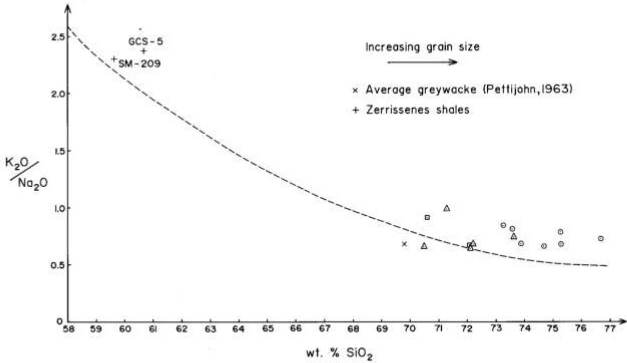
Fig. 4.2: Grain size variations strongly affect the geochemical composition of sediments, with decreasing grain size corresponding to a decrease in SiO 2 , and an increase in the K 2 O/Na 2 O ratio (adapted from Roser and Korsch, 1986). Symbols as for Fig. 4.1.
