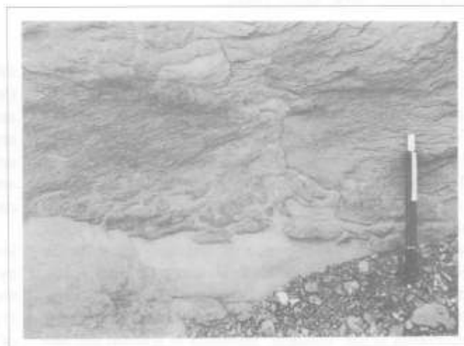
Plate 4.E: Dewatering structures at base of a facies B 1 bed (locality: Lonely River).
