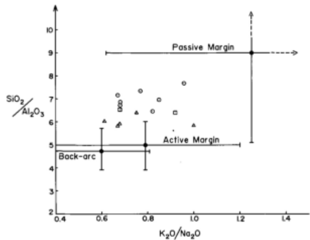
Fig. 4.4: Chemistry of modern deep-sea sands compared with that of the Zerrissenes greywackes. Extensive overlap of modern sands from different tectonic settings occurs and it is therefore difficult to categorise the ancient greywackes. The error bars on the modern analyses are one standard deviation each side of the mean (from Maynard et al. , 1982). Symbols as for Fig. 4.1.
