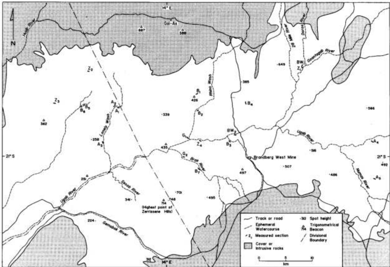
Fig. 1.3: Map of the lower Ugab River area showing major drainage lines, topographic features, routes and localities of measured sections. Section symbols are Z1 - Goantagab River; Z2- Ridge 6; Z3 - Skeleton Coast Park; Z4 - Augur; BW1 - Ulundi; BW2 - Ugab River; B1 - Shelter; B2 - Rhino Wash; B3 - Zebra River; B4 - Gai-as South; B5 - Gembok Altar East; B6 - Gembok Altar West; B7 - Brak River; G1 - Lookout; G2 - Corner; A1 - Jeppe East; A2 - Jeppe West; A3 - Lonely River; A4 - Bee; A5 - Tributary.
