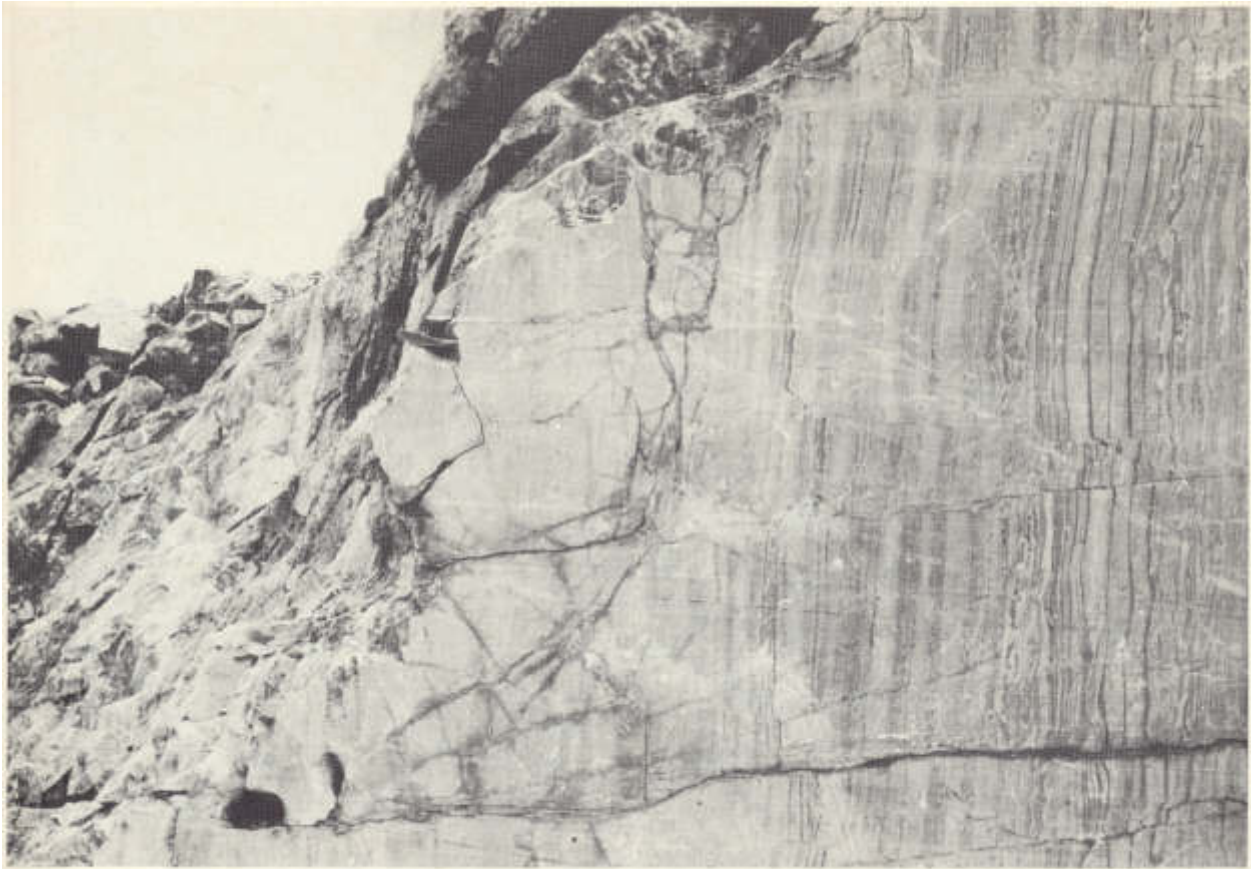
Plate VII.—Irregular joints near surface due to fluctuations in temperature. "Kudu" marble quarry, Karibib 54 (loc. 18). Plaat VII.—Onreëlmatige nate naby oppervlak te wyte aan temperatuurskommeling. "Kudu"-marmergroef, Karibib 54 (lok. 18).
