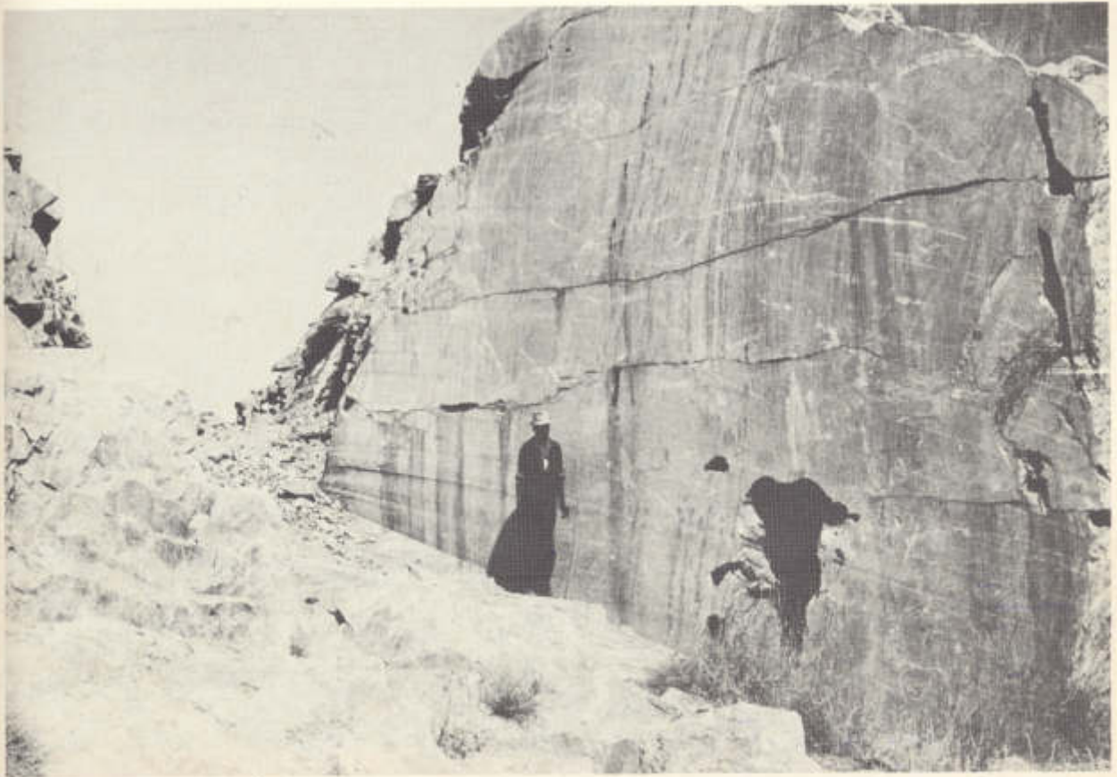
Plate VI.—Horizontal joints and solution cavities, "Kudu" marble quarry, Karibib 54 (loc. 18). Plaat VI.—Horizontale nate en oplossingsholtes, "Kudu"-marmargraef, Karibib 54 (lok. 18).
