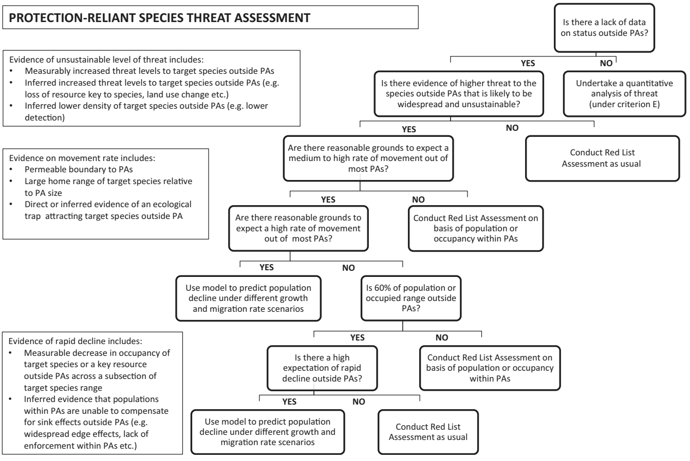
Fig. 4. Decision tree for threat assessment of protection-reliant species.
