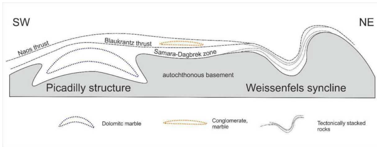
Figure 9. Schematic cross-section across the Samara-Dagbrek Zone, which illustrates the development of major sheath folds and/or tectonic stacks. Fold axes and stretching lineations are perpendicular to the cross section.
