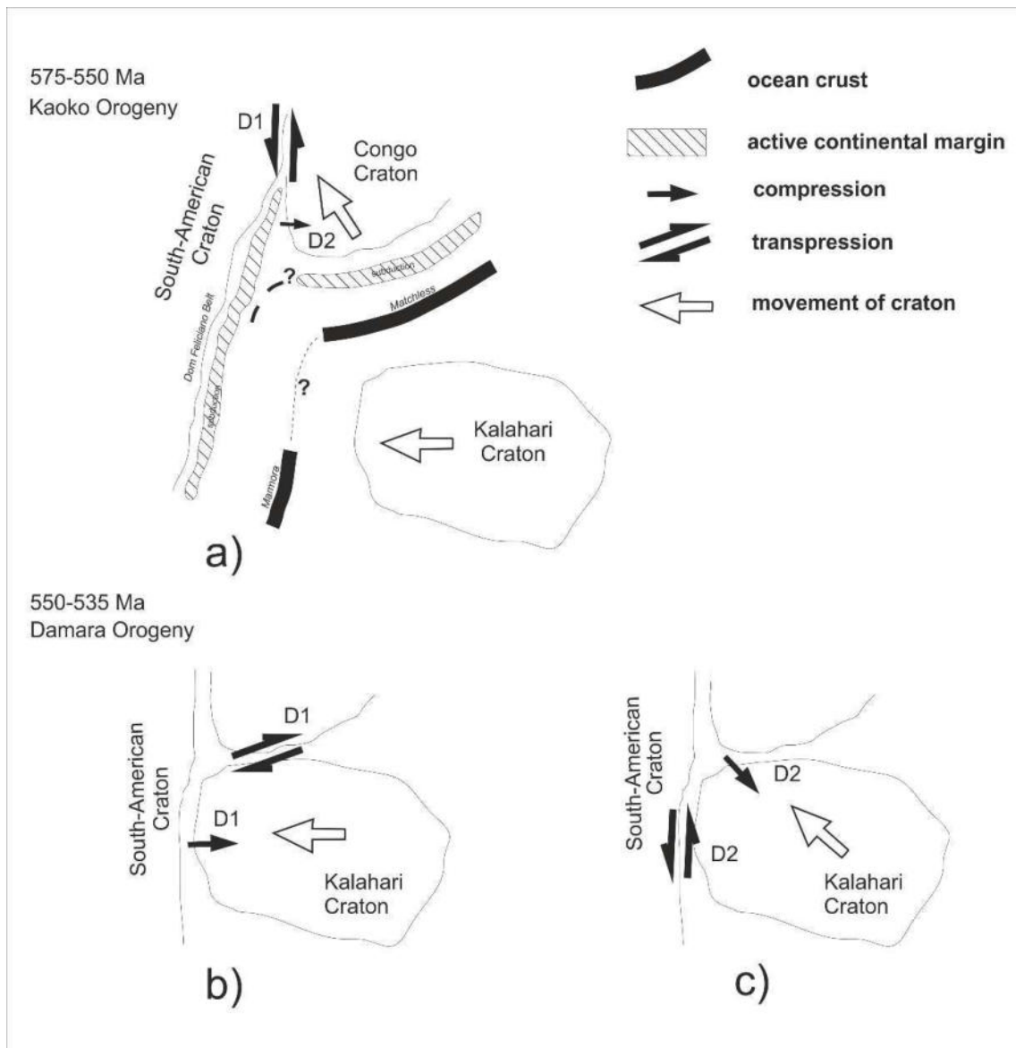
Figure 12. Interpretation of the observed deformation stages D1 and D2 in relationship to the relative plate movements of the Kalahari, Congo and South American cratons during the Kaoko and Damara orogenies.
