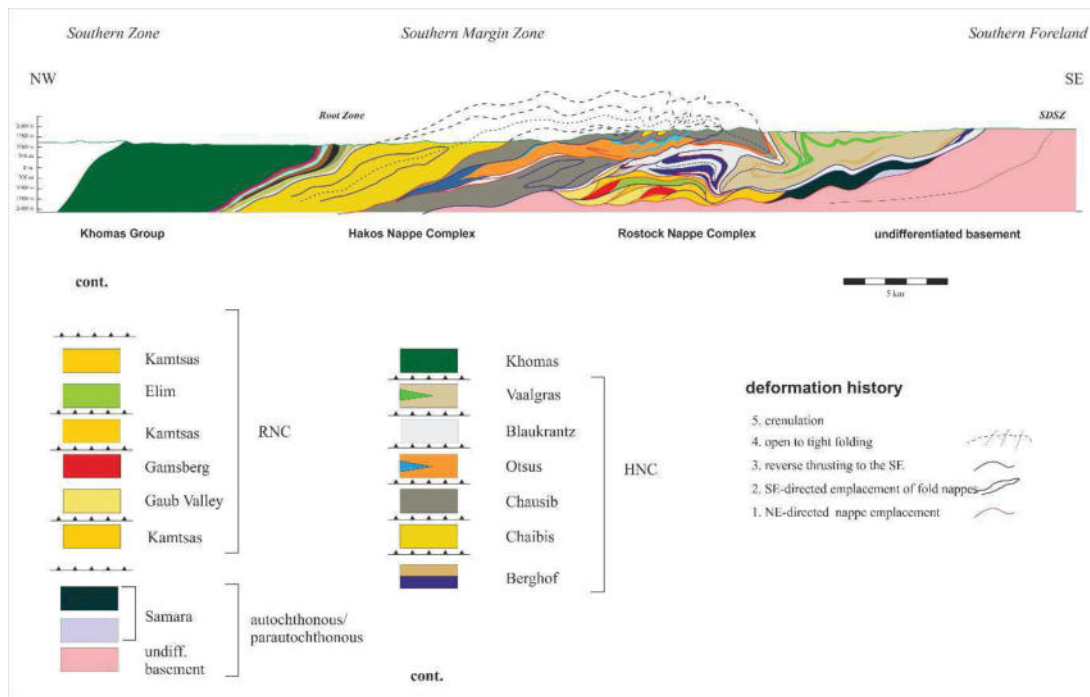
Figure 4. Synthetic cross-section and tectonic pile as derived from geological mapping.
