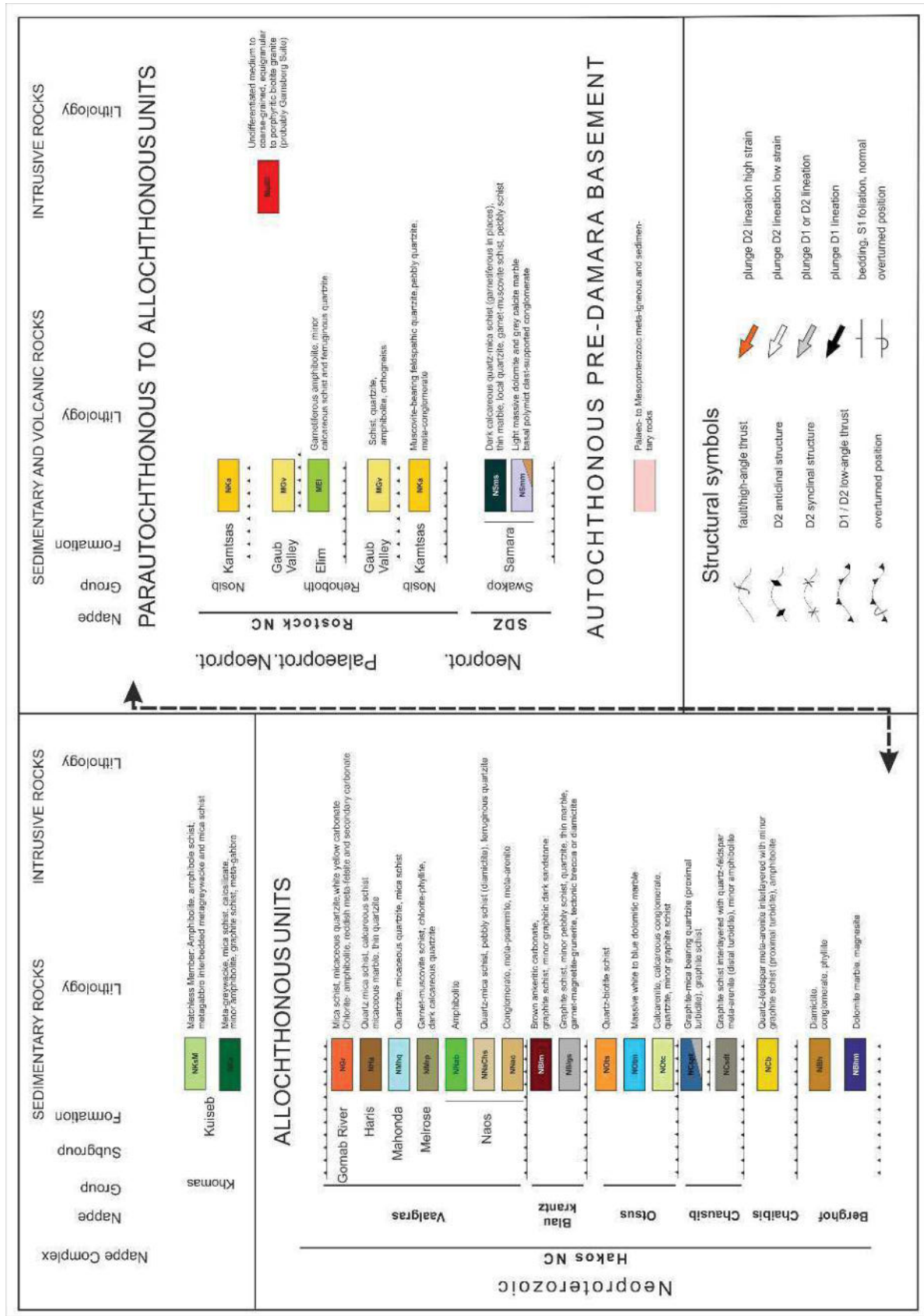
Figure 3. Geological map legend of the Hakos study area.
