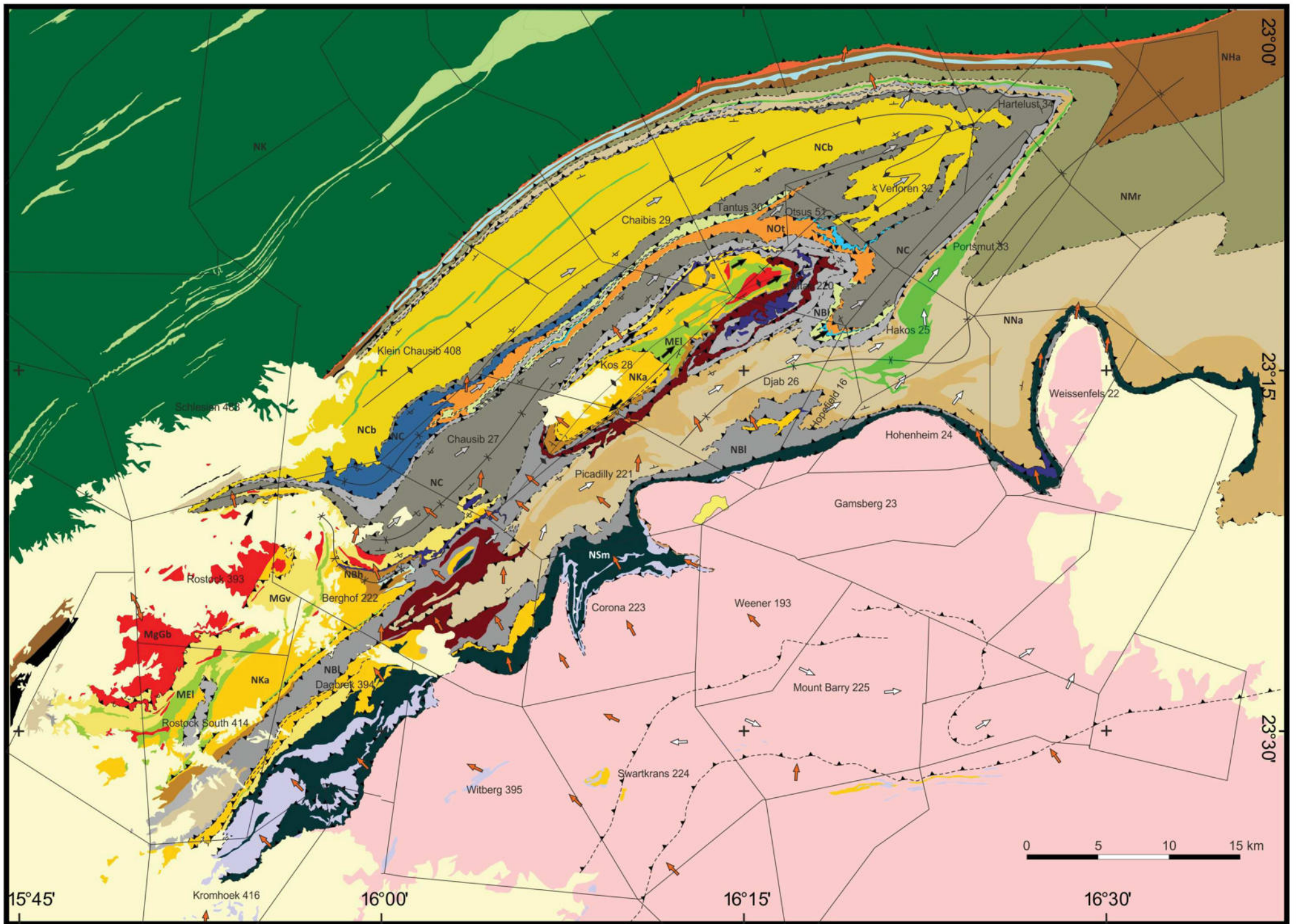
Figure 3. Geological map of the Hakos area
