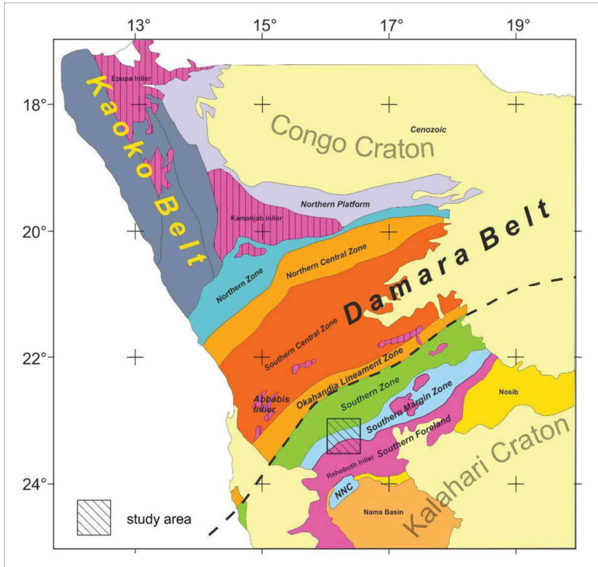
Figure 1. Simplified tectono-metamorphic map of Namibia illustrating the position of the Kalahari and Congo cratons with the Damara Mobile Belt in-between (supposed boundary marked by stippled line). Tectono-metamorphic subunits of the Kaoko belt are merged.
