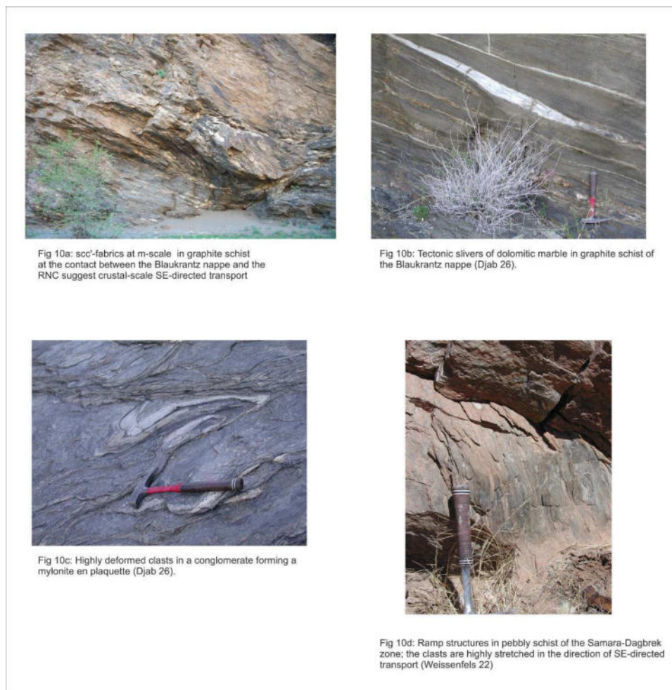
Figure 10. Structures at the basal contact of the Blaukrantz Nappe.
