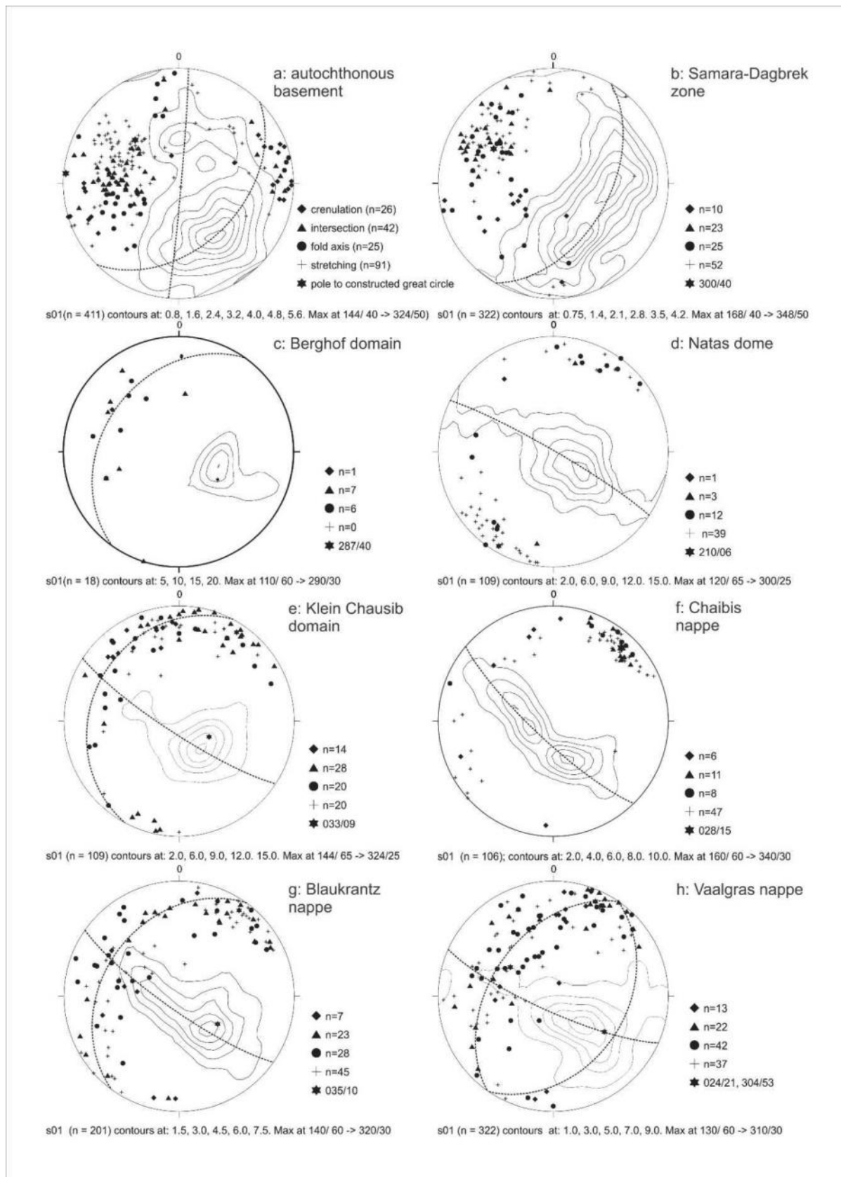
Figure 6. Presentation of structural data of the analysed domains in stereograms.
