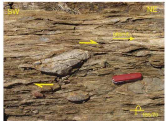
Figure 7f: D1 sigma-clasts are rotated during D2 around NE-plunging fold axes and, hence, indicate at the steeply overturned limb of the Hakos fold a dextral shear sense with the top (i.e. the lower part of the photo) to the SW (Natas 220)
