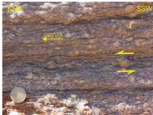
Figure 7e: Top to the NNE shear sense in orthogneiss of the Rostock Nappe Complex
