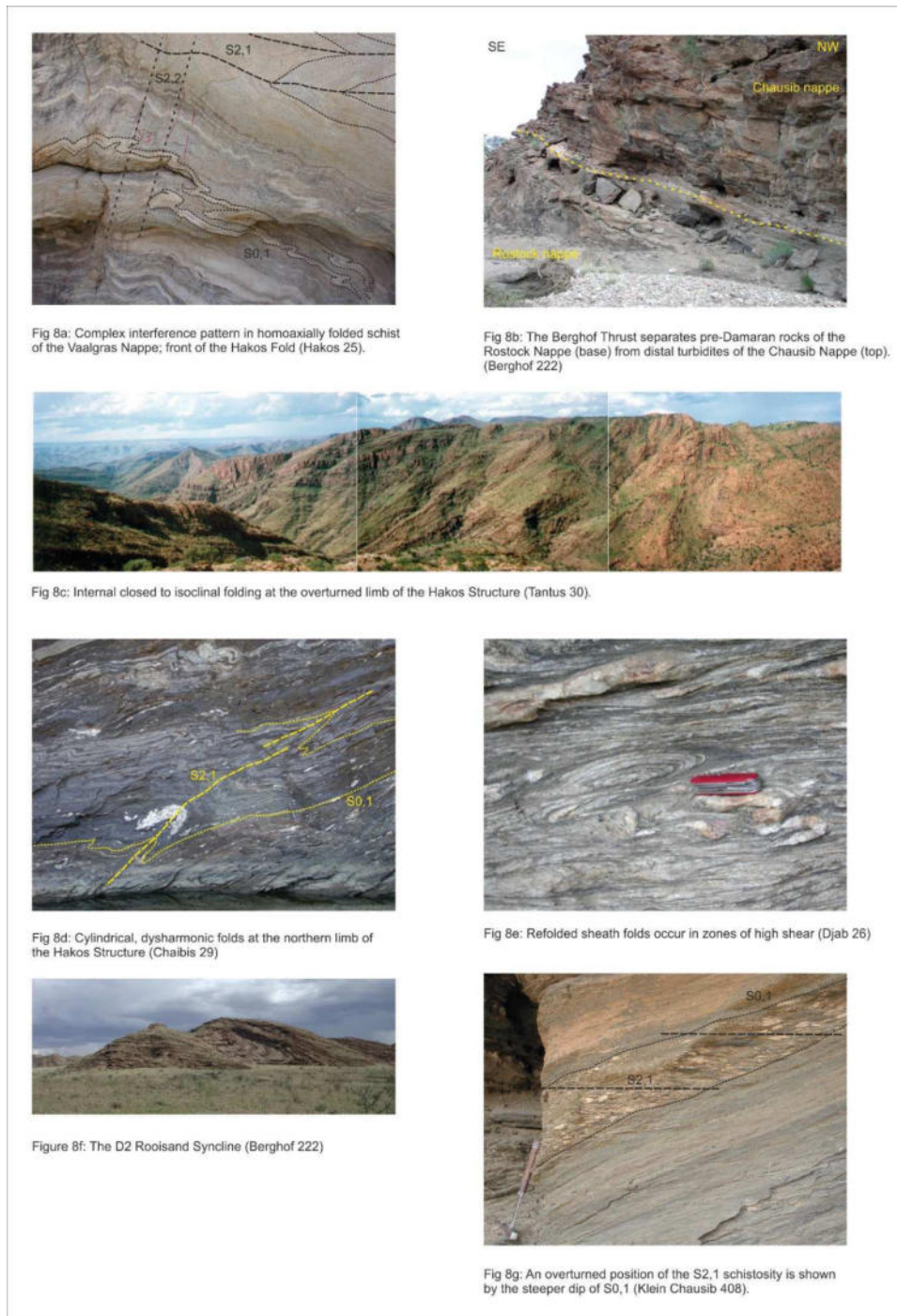
Figure 8. Tectono-metamorphic structures related to the SE-directed D2-deformation.
