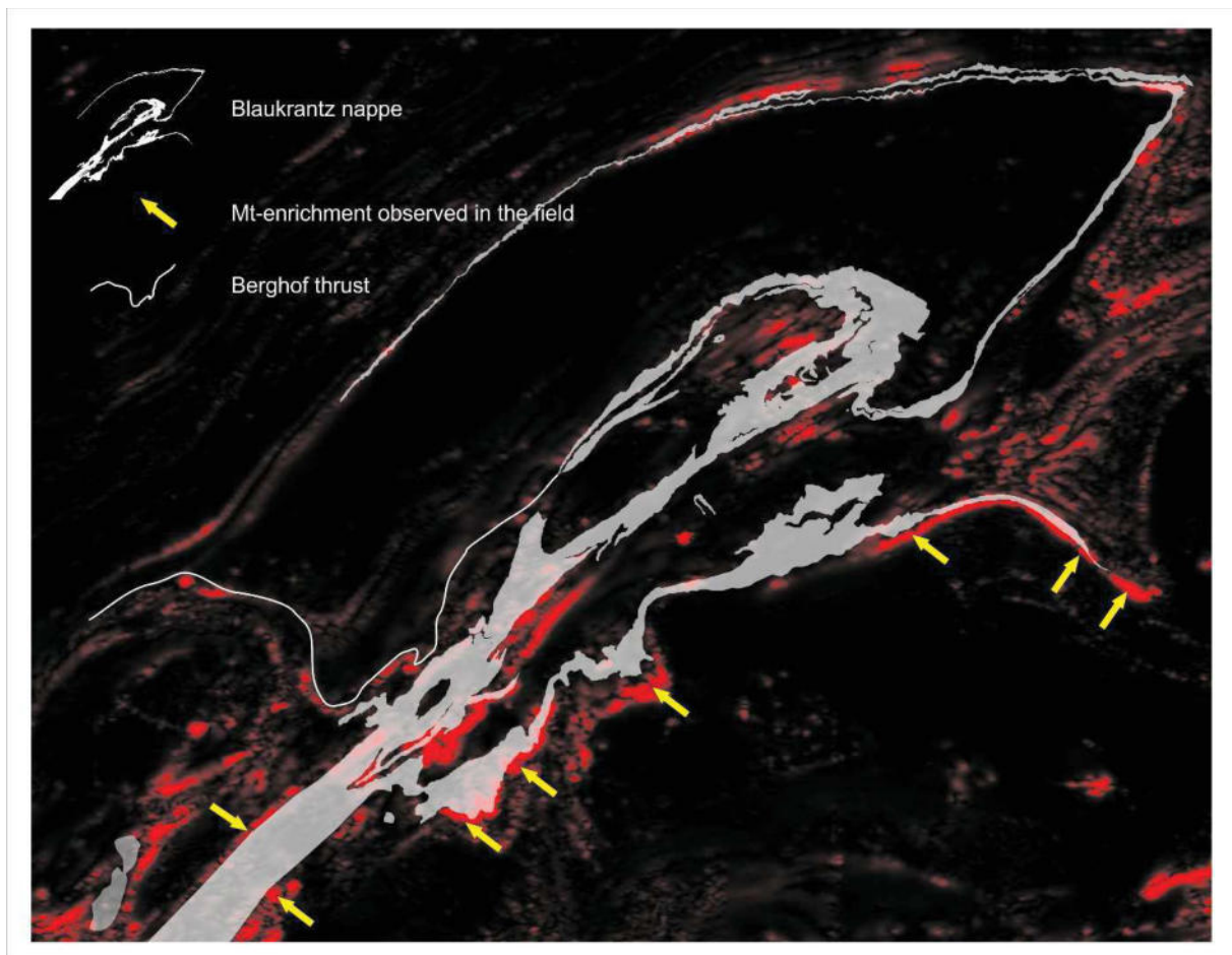
Figure 11. High-resolution airborne geophysics (magnetics; 1st vd) demonstrates? near the basal contact of the Blaukrantz Nappe? irregular positive anomalies in various underlying formations caused by the enrichment of magnetite. The iron was probably transported by metamorphic fluids and crystallised in the thrust; the overlying graphite schist may have acted as an impermeable barrier.
