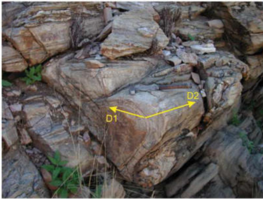
Fig 7a: Interference pattern of D1 (330/15) and D2 (060/10) folds in quartzite of the Nosib G (Berghof 222)
