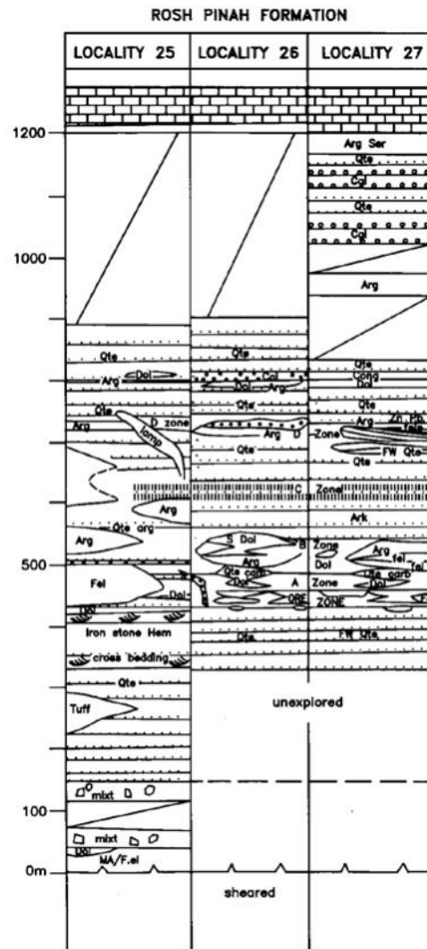
Figure 3: Provisional stratigraphic sketch of the Rosh Pinah unit at the type area at localities 24, 25, and 26 (after Kindl, 1979)
