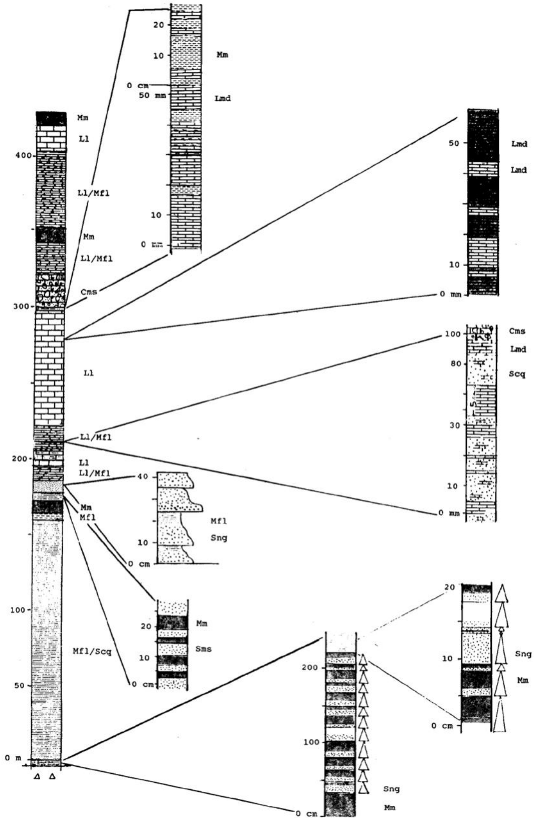
Figure 13: Measured section through the Pickelhaube Formation at Dreigratberg
