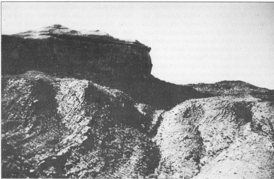
Figure 25: Little-deformed carbonates of the Pickelhaube Formation thrust over strongly folded and foliated sandstones and conglomerates of the Rosh Pinah Formation at Pickelhaube
