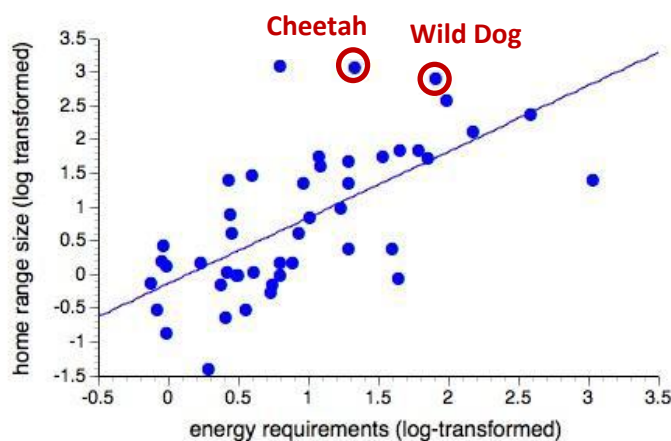
Figure 2.1 The relationship between energy requirements and home range size in multiple carnivore species, showing the large home ranges occupied by cheetah and wild dogs in comparison with their energy needs. Wild dogs are recorded as having greater needs than cheetah because the social unit is a pack rather than an individual. Data are from Gittleman & Harvey (1982).
