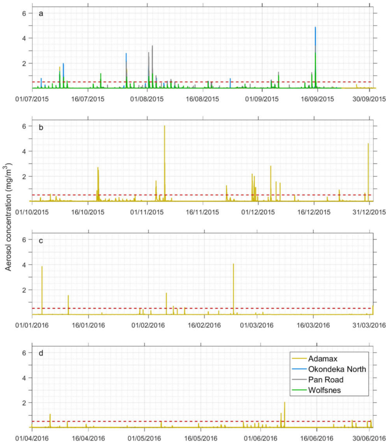
Figure 4. Time series of measured aerosol concentration (PM 10 , mg/m 3 ) throughout the full experimental period for the four monitoring stations at the west of the Pan. The horizontal red dashed line indicates the threshold used to identify individual dust events, where measured aerosol concentration exceeded 0.5 mg/m 3 ( n = 51 ). (a) July–September 2015, (b) October–December 2015, (c) January–March 2016, (d) April–June 2016.
