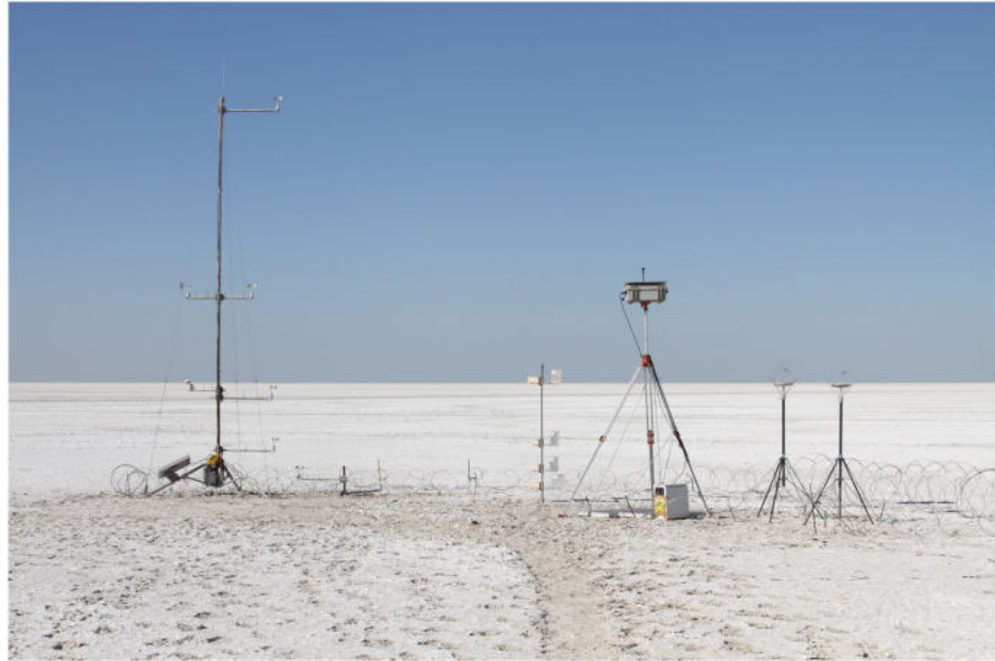
Figure 2. A typical monitoring station (Pan Road) showing a 6 m anemometer tower on the left and a TSI DustTrak DRX aerosol monitor on the tripod in the center-right. All instrument data were logged at an interval of 10 min.
