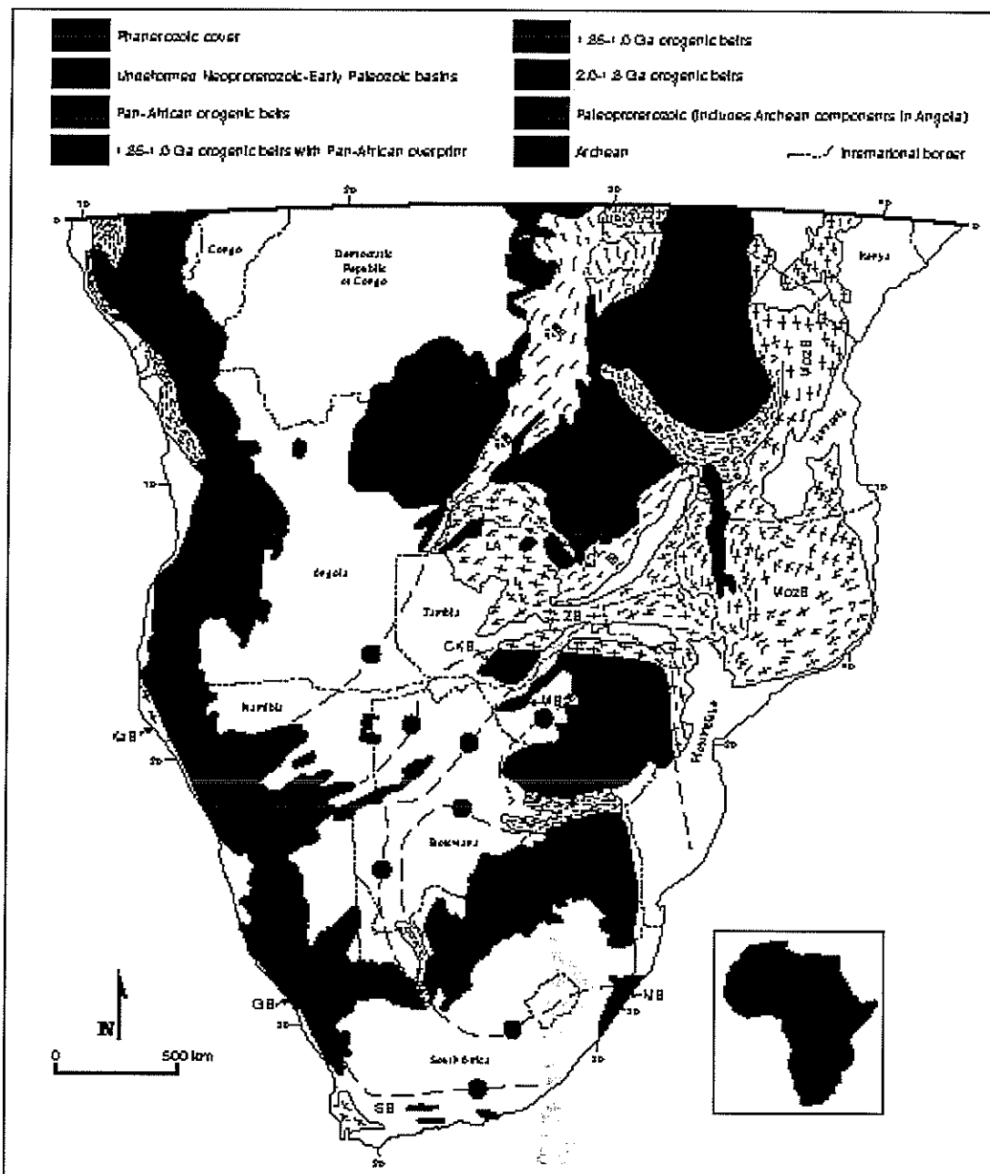
Figure 1. Precambrian tectonic framework of southern Africa. Transcurrent shear zones and many basement inliers within younger belts are not shown. 2.0-1.8 Ga belts: UsB = Usagaran belt; UB = Ubendian belt; BB = Bangweulu block; MB = Magondi belt; KhB = Kheis belt; R = Richtersveld terrane; LB = reactivation in Archean Limpopo belt. 1.35-1.0 Ga belts: KB = Kibaran belt; IB = Irumide belt; CKB = Choma-Kalomo block; NaqB = Namaqua belt; NB = Natal belt. Pan-African belts: MozB = Mozambique belt; ZB = Zambezi belt; LA = Lufilian arc; DB = Damara belt; WCB = West Congo belt; KaB = Kaoko belt; GB = Gariiep belt; SB = Saldania belt. Inferred boundaries beneath cover: 1 = eastern margin of Kheis-Magondi belt; 2 = boundary between Kheis-Magondi belt and 1.35-1.0 Ga belt to west; 3 = boundaries of Damara-Lufilian-Zambezi system; 4 = boundaries of Namaqua-Natal belt.
