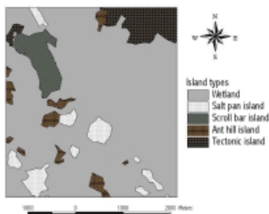
Figure 7: Object-oriented island classification of the same area as in Fig. 6 (see text).
