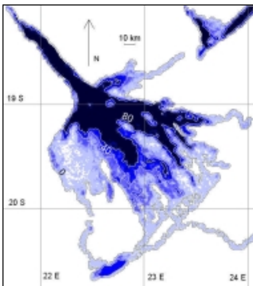
Figure 2: Percent of time with water cover – isolines for 0, 40 and 80 % water coverage are shown.
